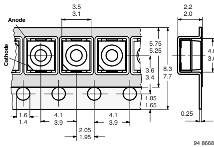
Figure 9. Tape dimensions in mm for PLCC-2
