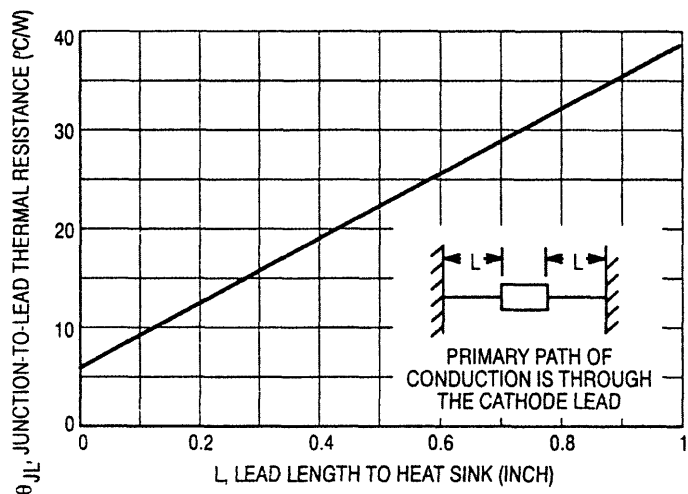
Figure 5. Typical Thermal Resistance
