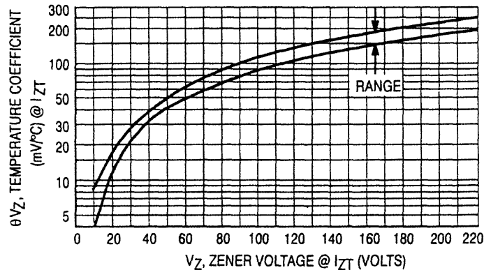
Figure 3. Temperature Coefficient-Range for Units 10 to 220 Volts
