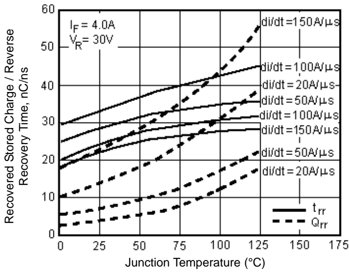
Reverse Switching Characteristics
