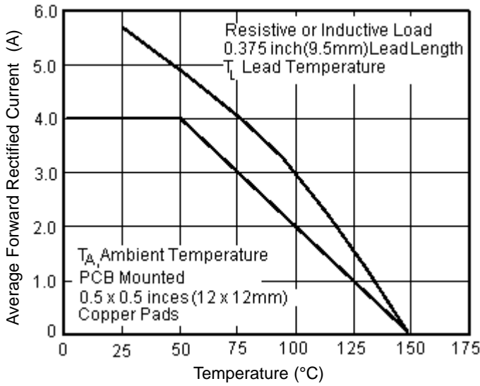
Forward Current Derating Curves
