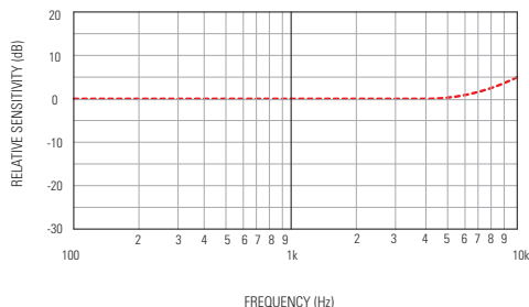
9.7x4.5 FREQUENCY RESPONSE
