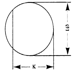
Recommended Panel Cutout (For Single Hole Mounting)
