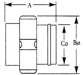
Inline Plug
