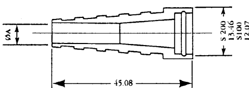
2007 Arr. 7*20 Contacts
