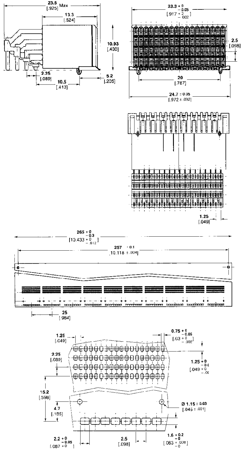
Recommended PCB Layout
