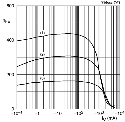
V_{CE} = -2 V (1) T_{amb} = 100\text{ }^{\circ}C (2) T_{amb} = 25\text{ }^{\circ}C (3) T_{amb} = -55\text{ }^{\circ}C
