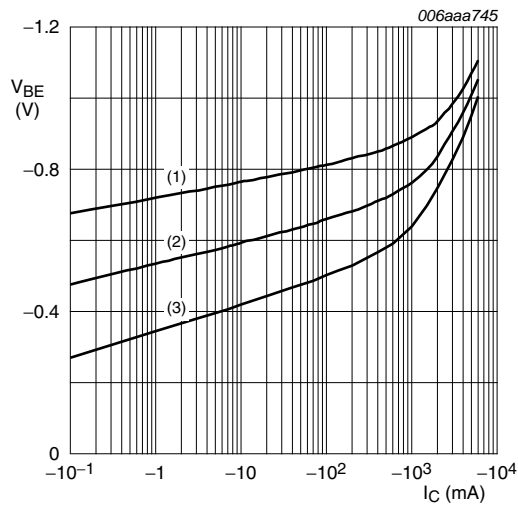
V_{CE} = -2 V (1) T_{amb} = -55\text{ }^{\circ}C (2) T_{amb} = 25\text{ }^{\circ}C (3) T_{amb} = 100\text{ }^{\circ}C
