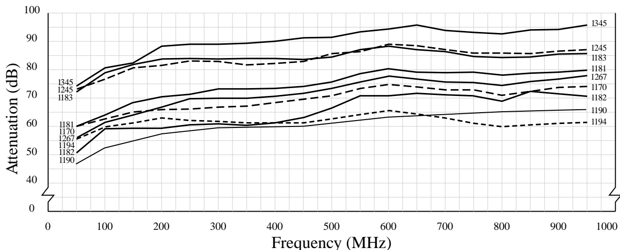
Shielding Effectiveness (Far Field) - Typical Values (ASTM-D-4935)
