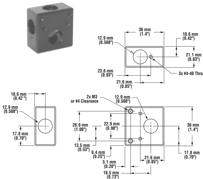
SMB127 Mounting Block
