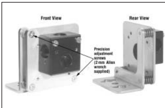
Figure 1a. Mounting bracket model SMB46X3, front and rear views
