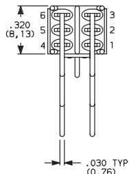
Terminal Nos. For Reference Only
