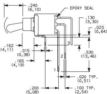
Terminal Nos. For Reference Only
