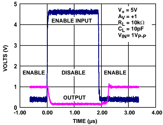
FIGURE 13. ENABLE/DISABLE TIMING
