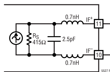
Figure 8. IF Output Small-Signal Model
