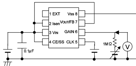
Circuit ⑦
