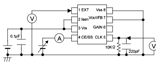
Circuit ⑦
