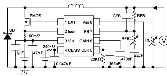
Circuit ① (FB Type)
