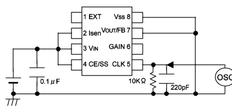
Circuit ③
