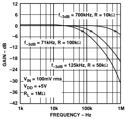
Figure 20. Normalized Gain Flatness vs. Frequency
