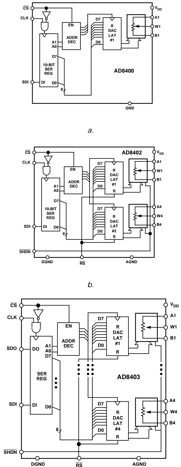
c. Figure 38. Block Diagrams
