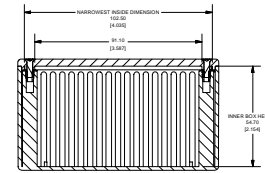
SECTION D-D SCALE 3/4
