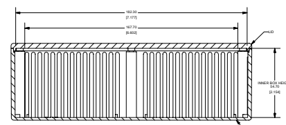
SECTION C-C SCALE 3/4
