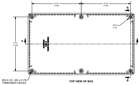
TOP VIEW OF BOX
