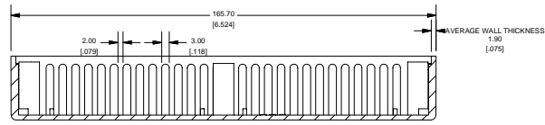
SECTION A-A SCALE 3 / 4
