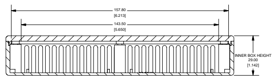
SECTION C-C SCALE 3 / 4
