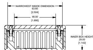
SECTION D-D SCALE 3 / 4
