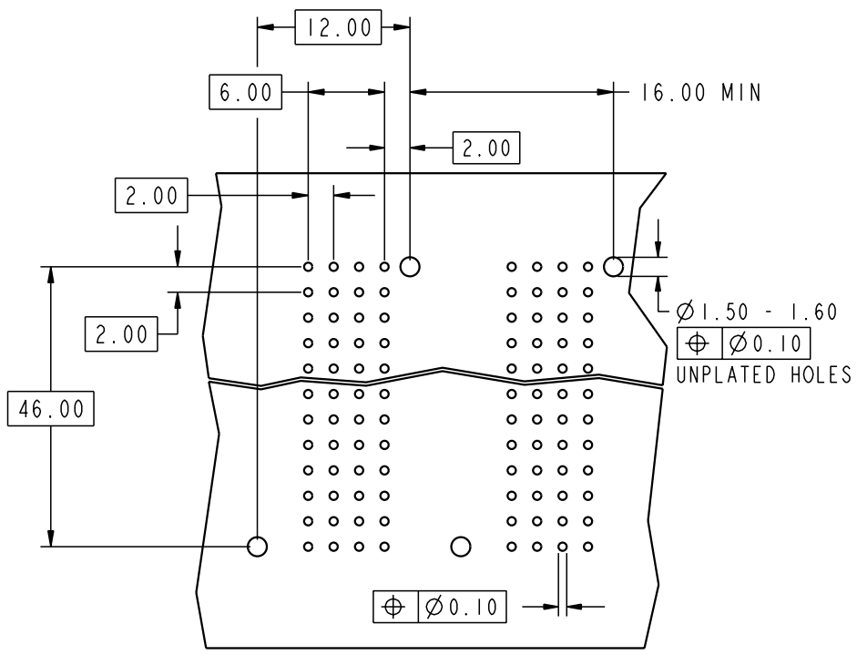
REQUIRED PC BOARD LAYOUT COMPONENT SIDE SEE PRINT 58351 FOR ADDITIONAL PCB INFORMATION
