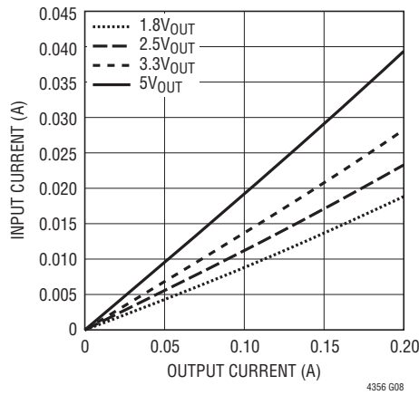
Input Current vs Output Current (36V IN )
