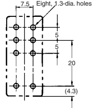
Mounting Holes
