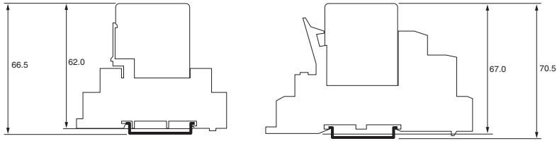
P2RF-□
