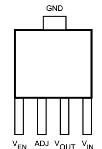
20126703 SOT-223, Top View LP38692MP-ADJ
