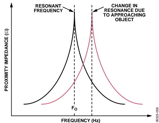
Figure 36. Detecting a Change in Resonant Frequency
