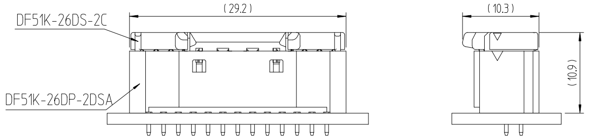
ENGAGEMENT FIGURE (2:1)
