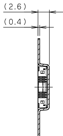
SECT. E-E (8~21P)
