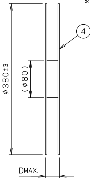
REEL DIMENSION
