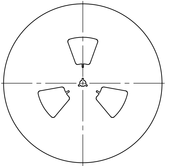
REEL DIMENSION
