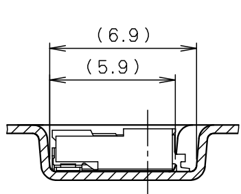
SECT. F-F (s=4:1)
