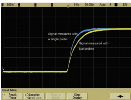
Figure 2-1. Probe loading check with two probes.
