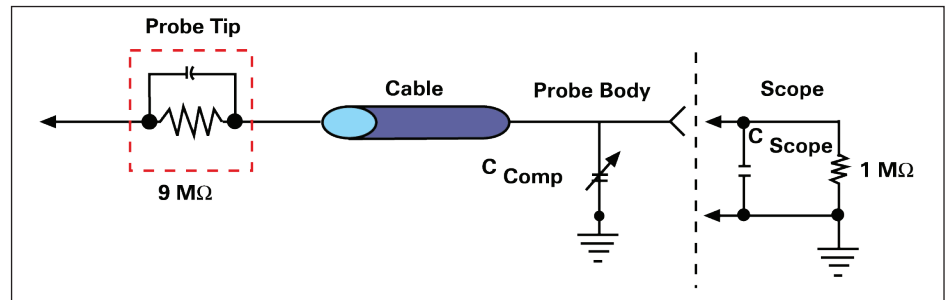
Figure 3-1. Use a small screw driver to adjust the probe's variable capacitance.
