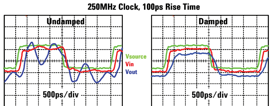
Figure 8-3. As the speeds in your design increase, you may notice more overshoot, ringing and other perturbations. Overcome the resonance formed by the connection of a probe by adding a damp resistor to your probe tip.
