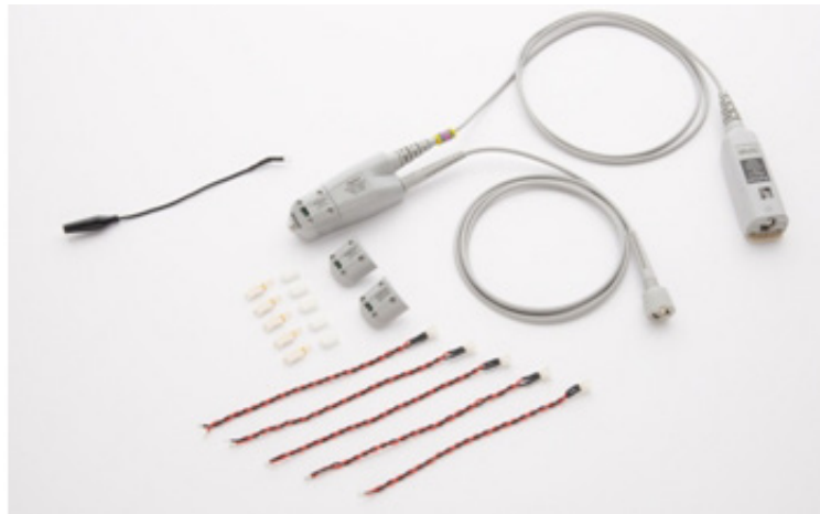
Figure 4-3. The new N2820A/21A AC/DC current probes offer the industry's highest sensitivity among oscilloscope current probes.
