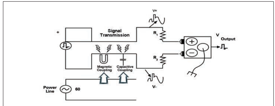
Figure 6-2. Differential active probe provides much higher common mode rejection ratio effectively eliminating common mode noise current.
