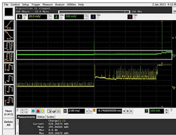
Figure 4-5. Keysight's Infiniium and InfiniiVision oscilloscopes provide an area under the curve measurement (Charge), where you can easily calculate the integrated current consumptions in Ah (Ampere x Hour) over time.
