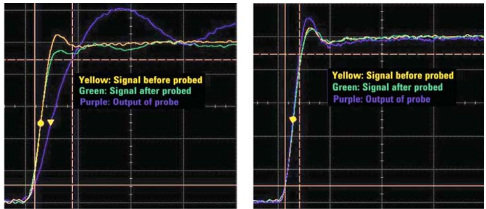
Figure 1-1. Comparison of passive and active probe measuring a signal that has a 600 psec rise time.
