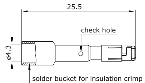
Main Dimension contact socket
