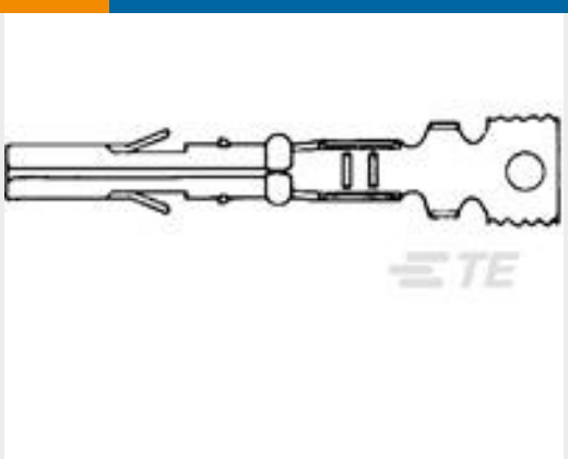
TE Part #641300-2 MR RECPT AUPHBZ LP 26-18
