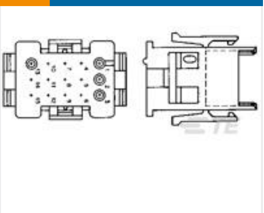
TE Part #1-640510-0 06P MR II CAP HSG V0
