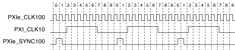
Figure 7. System Reference Clock Default Behavior
