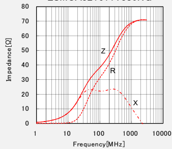
LSMCA321611T380NG
