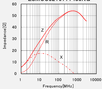
LSMCC321611T480NG
