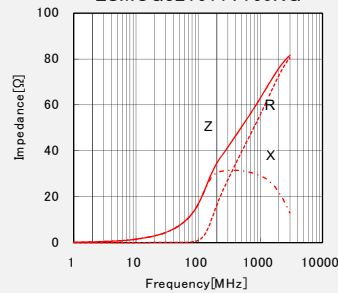
LSMCG321611T160NG
