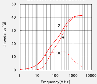
LSMCA160808T230NG
