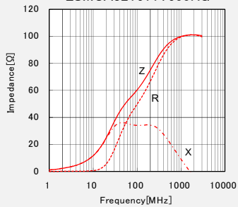
LSMCA321611T600RG
