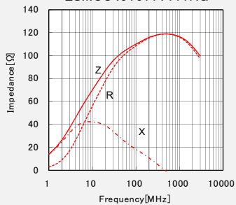
LSMCC451611T111RG
