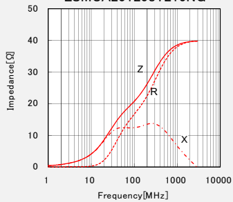
LSMCA201208T210NG
