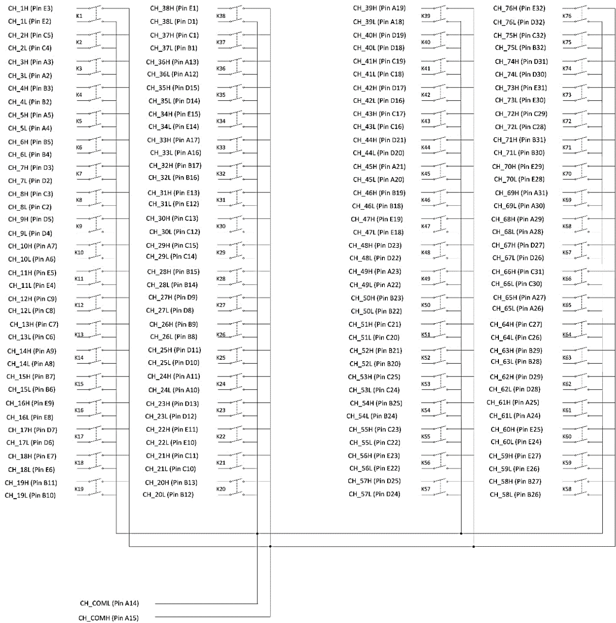
FIGURE 3-54: SMX-3279 LOGICAL DIAGRAM
