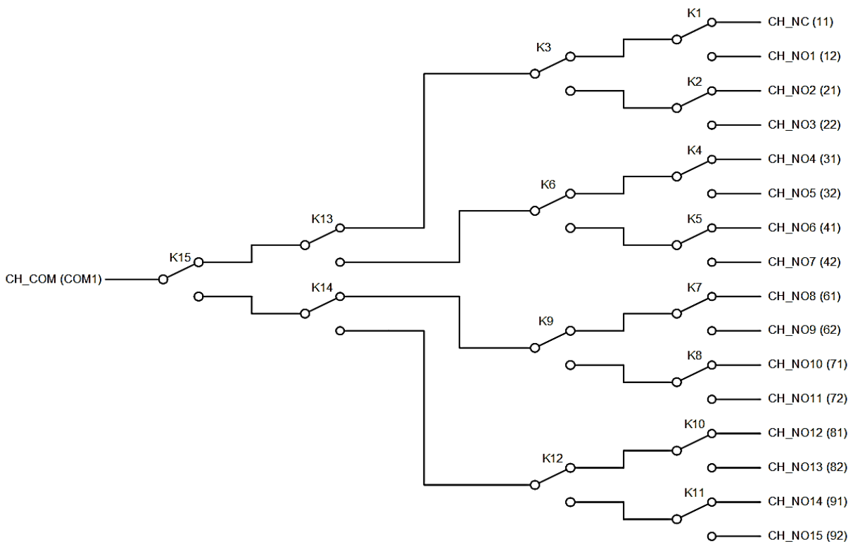
FIGURE 3-114: SMX-6116SMB LOGICAL DIAGRAM
