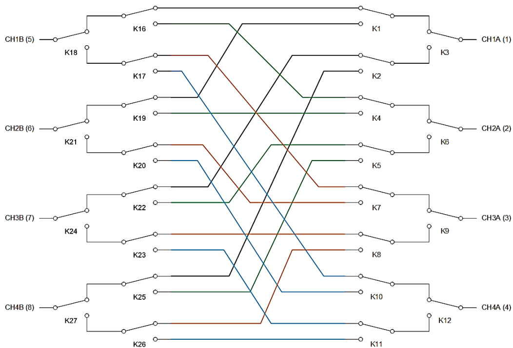
FIGURE 3-141: SMX-6144SMB LOGICAL DIAGRAM
