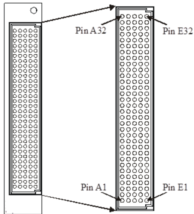
FIGURE 3-53: SMX-3279 FRONT PANEL CONNECTOR (FRONT VIEW)
