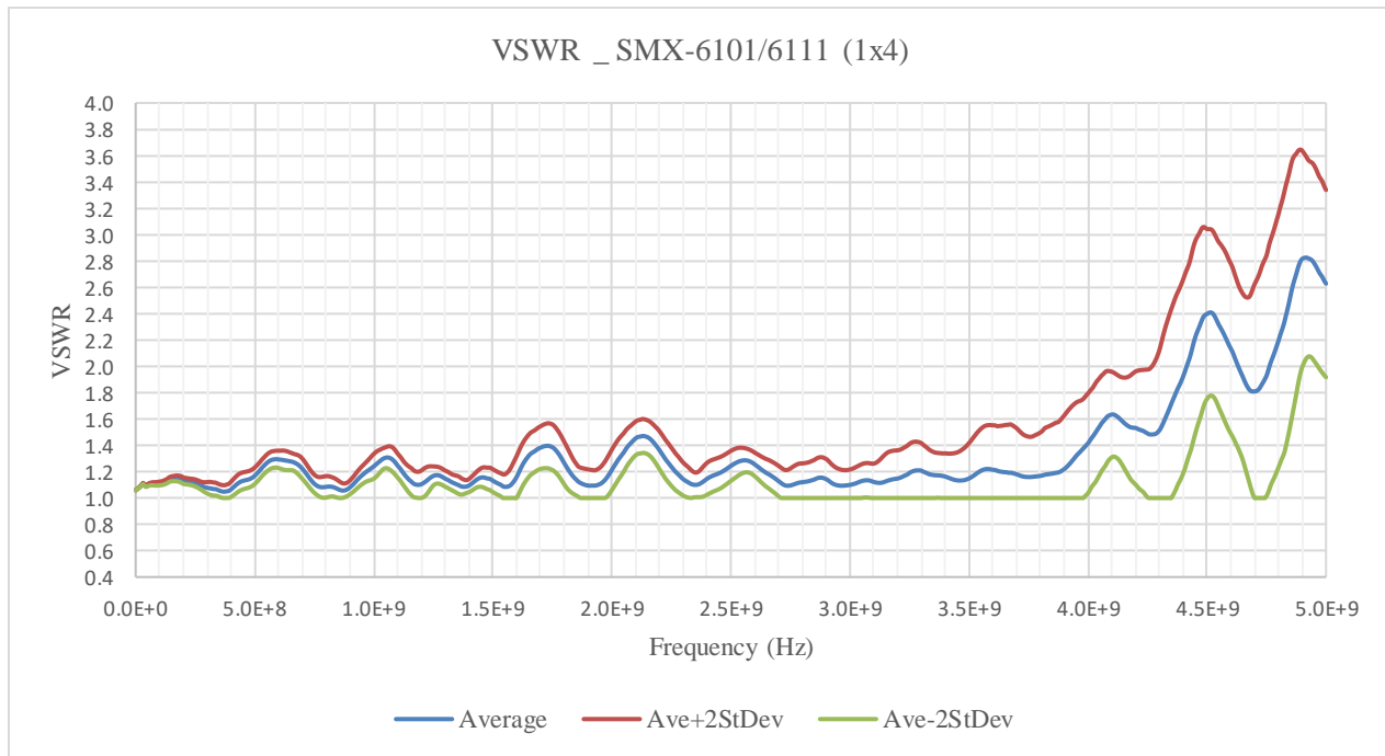
FIGURE 3-105: SMX-6111PKZ VSWR GRAPH
