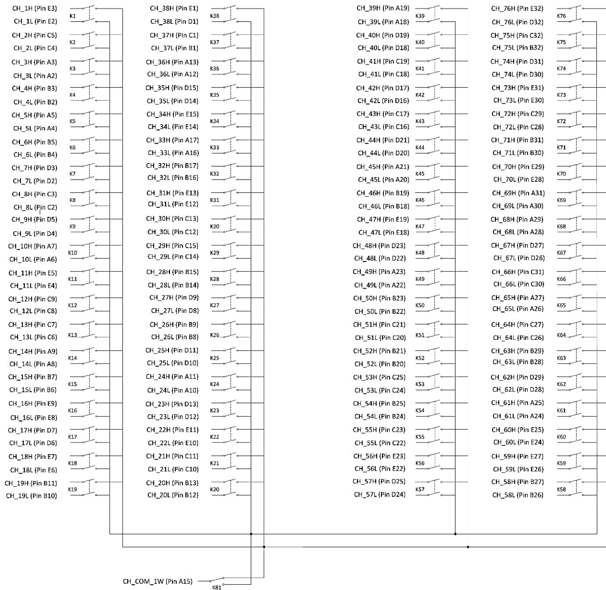
FIGURE 3-58: SMX-3280 LOGICAL DIAGRAM
