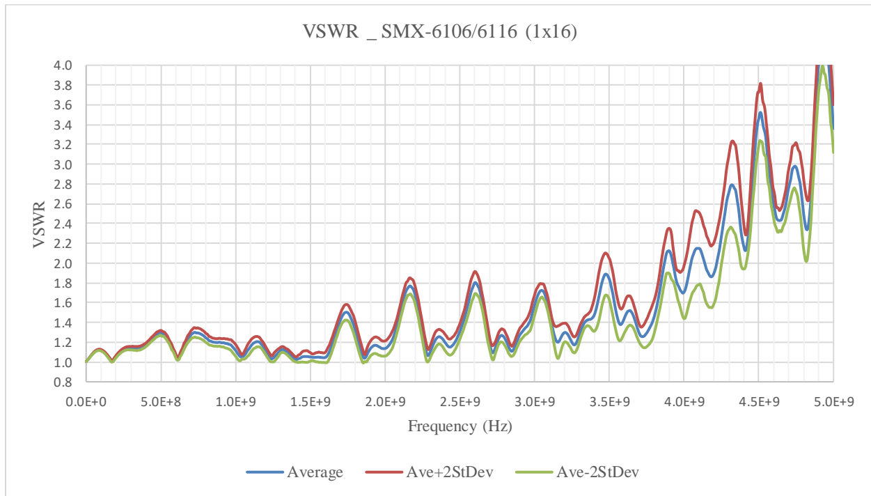
FIGURE 3-111: SMX-6106SMB AND PkZ VSWR GRAPH
