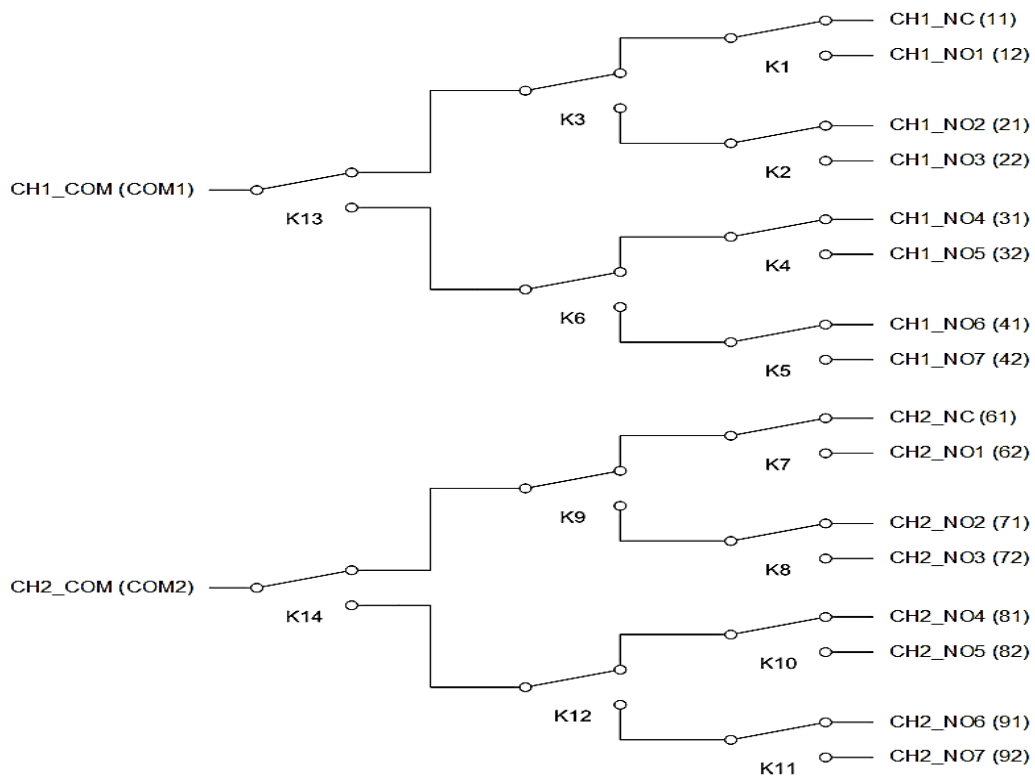
FIGURE 3-127: SMX-6115SMB LOGICAL DIAGRAM
