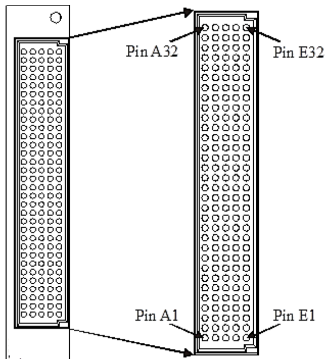
FIGURE 3-29: SMX-3004 FRONT PANEL CONNECTOR PINS (FRONT VIEW)
