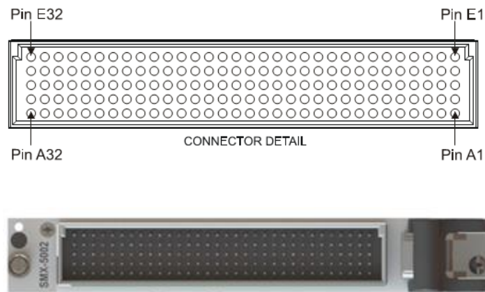
FIGURE 3-87: SMX-5002 CONNECTOR PIN LOCATIONS
