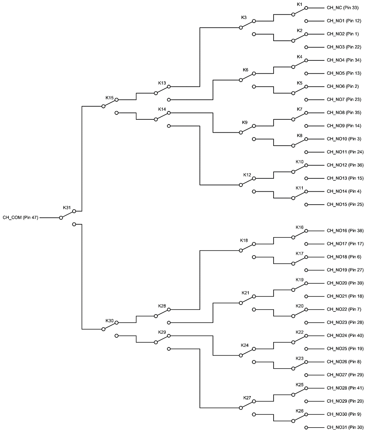
FIGURE 3-133: SMX-6103PkZ LOGICAL DIAGRAM
