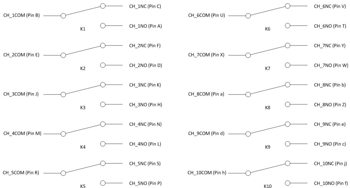
FIGURE 3-11: SMX-2002-10 LOGICAL DIAGRAM
