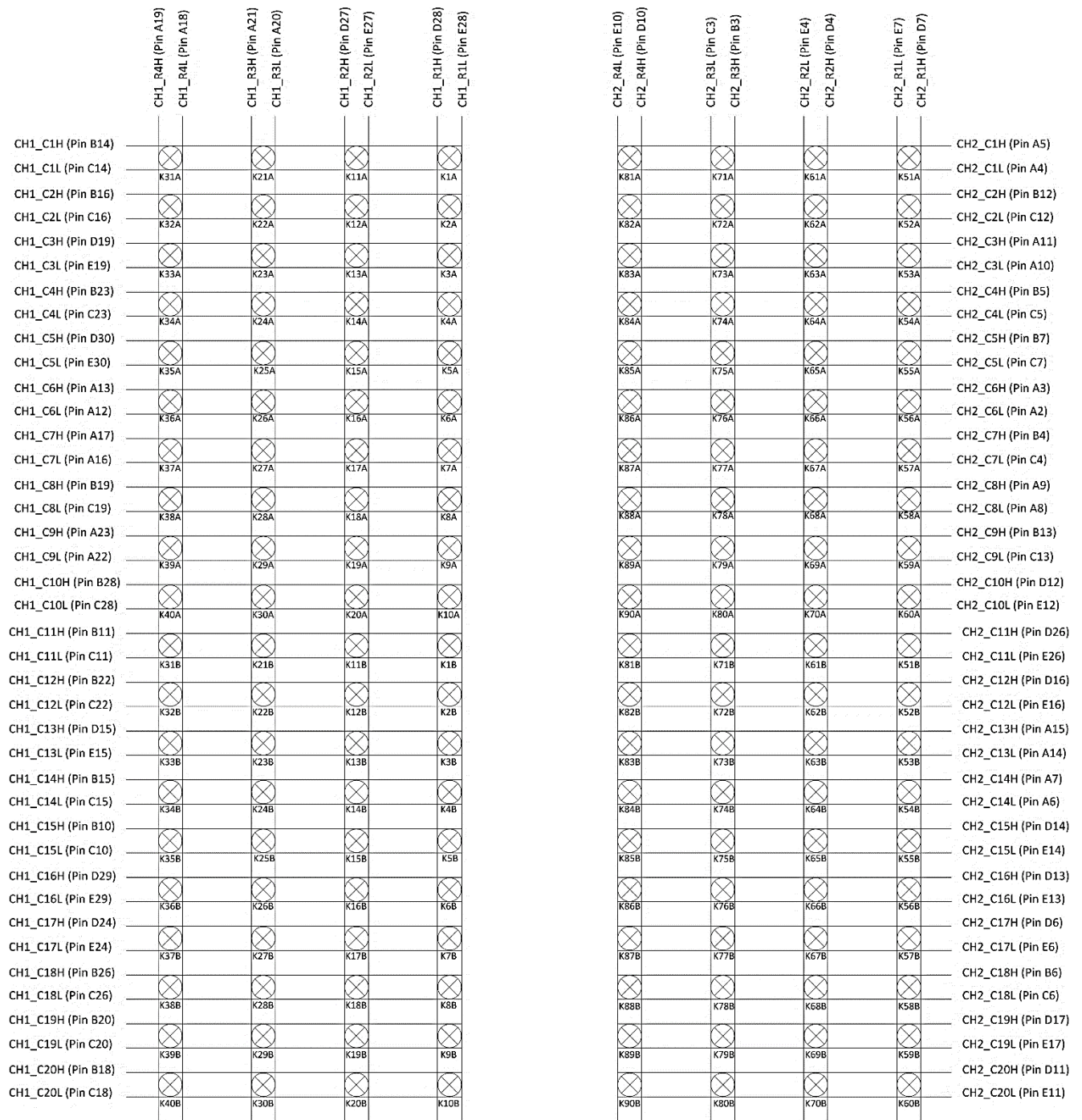
FIGURE 3-78: SMX-4412 LOGICAL DIAGRAM
