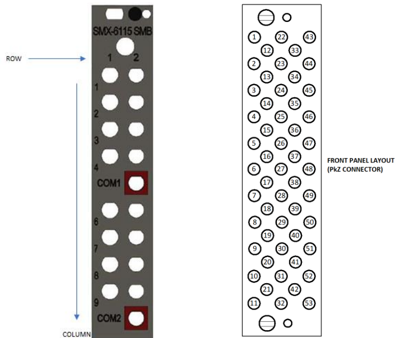
FIGURE 3-125: SMX-6115 FRONT PANEL LAYOUT (SMB CONNECTOR -LEFT IMAGE, PkZ CONNECTOR- RIGHT IMAGE)
