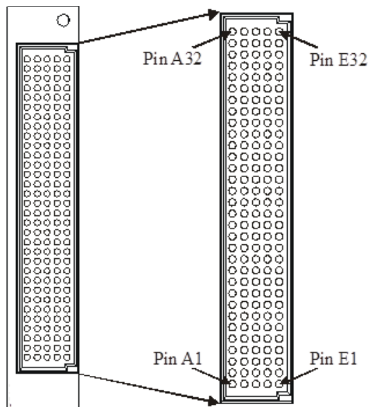
FIGURE 3-43: SMX-3276DS FRONT PANEL CONNECTOR (FRONT VIEW)
