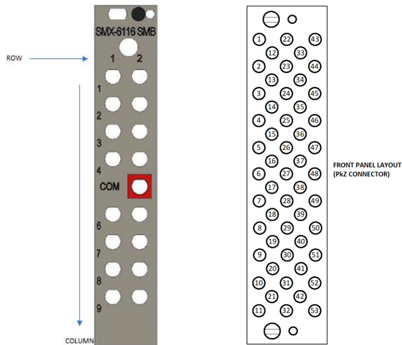
FIGURE 3-112: SMX-6116 FRONT PANEL LAYOUT (SMB CONNECTOR -LEFT IMAGE, PkZ CONNECTOR- RIGHT IMAGE)
