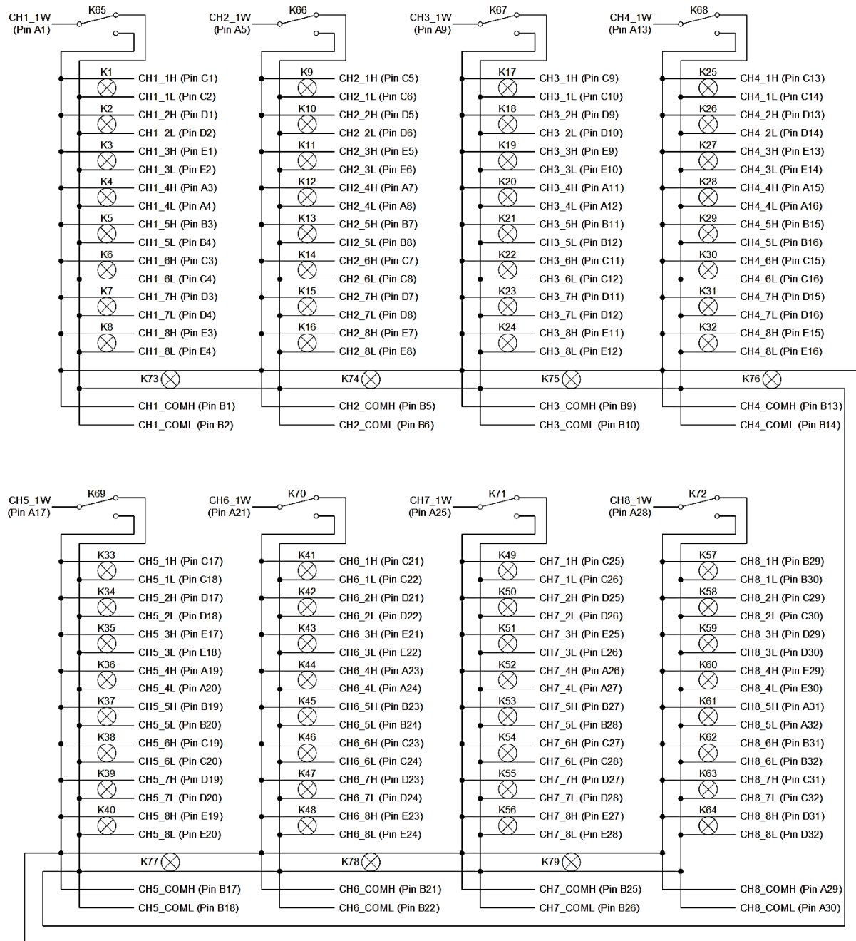
FIGURE 3-17: SMX-3001 LOGICAL DIAGRAM
