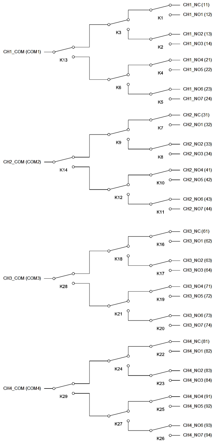
FIGURE 3-120: SMX-6105SMB LOGICAL DIAGRAM
