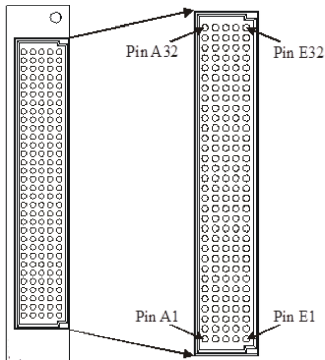
FIGURE 3-25: SMX-3003 FRONT PANEL CONNECTOR PINS (FRONT VIEW)
