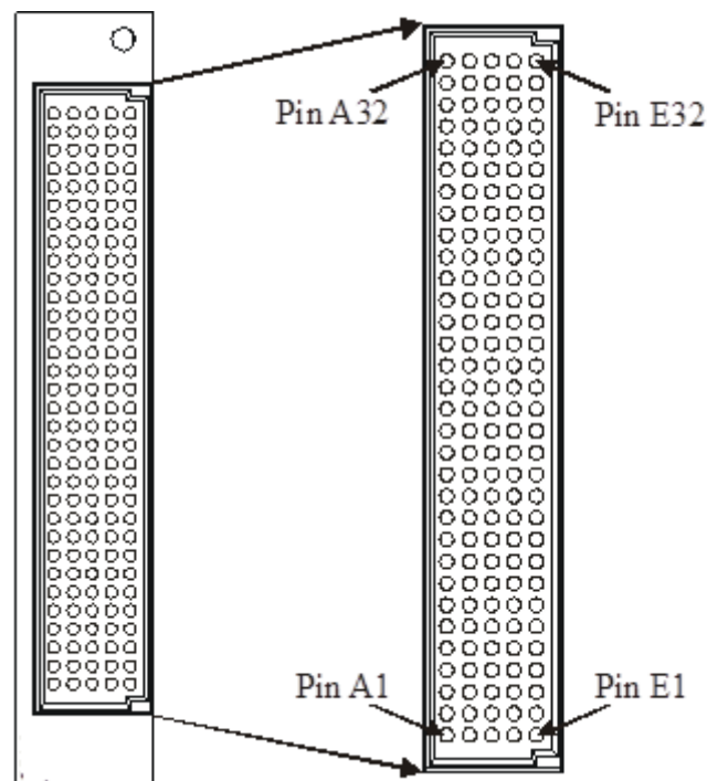
FIGURE 3-47: SMX-3277DS FRONT PANEL CONNECTOR (FRONT VIEW)
