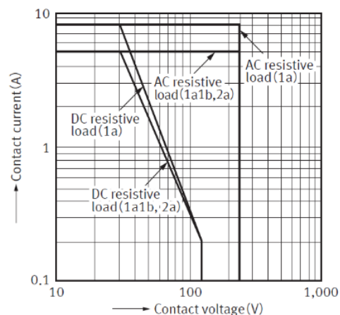
FIGURE 3-91C: SMX-5004 SWITCHING VOLTAGE AND CURRENT
