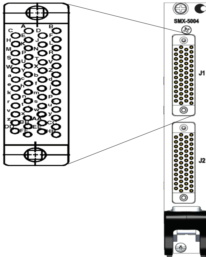
FIGURE 3-89A: SMX-5004 CONNECTOR PIN LOCATIONS
