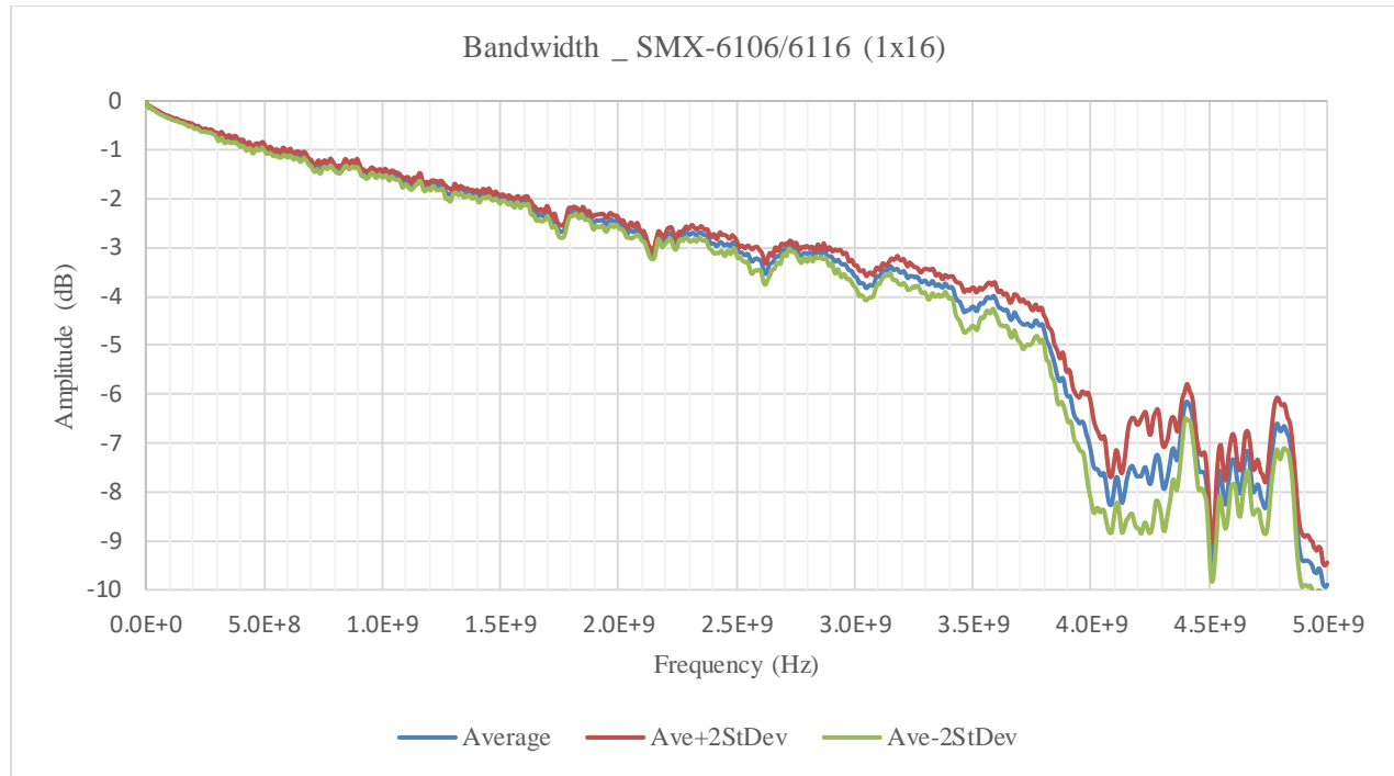
FIGURE 3-115: SMX-6116SMB BANDWIDTH GRAPH
