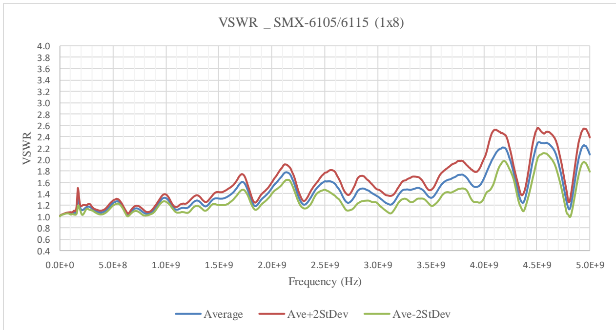
FIGURE 3-131: SMX-6115PkZ VSWR GRAPH
