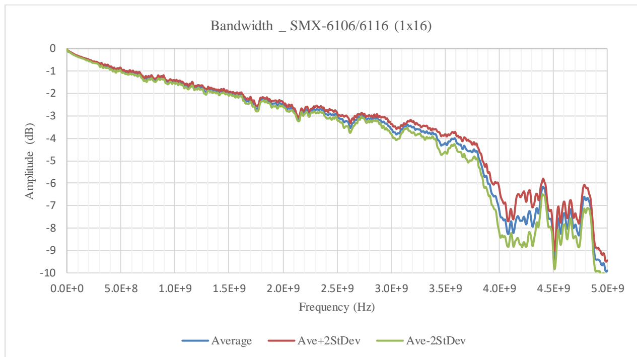
FIGURE 3-109: SMX-6106SMB BANDWIDTH GRAPH
