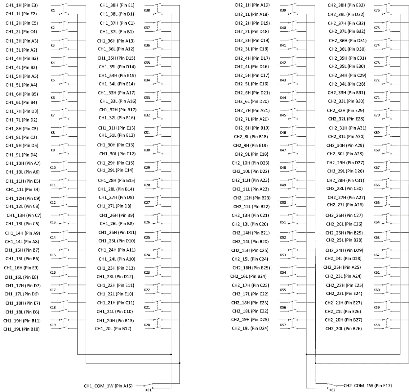
FIGURE 3-46: SMX-3277 LOGICAL DIAGRAM
