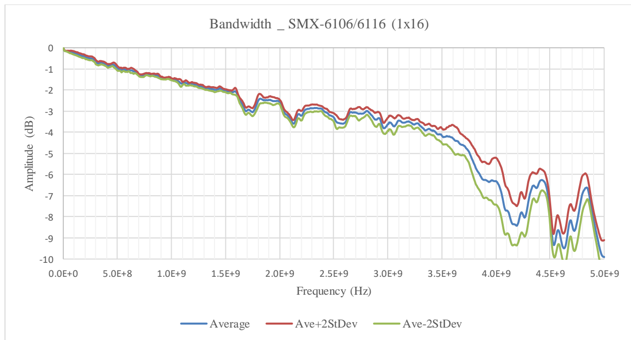
FIGURE 3-110: SMX-6106PkZ BANDWIDTH GRAPH
