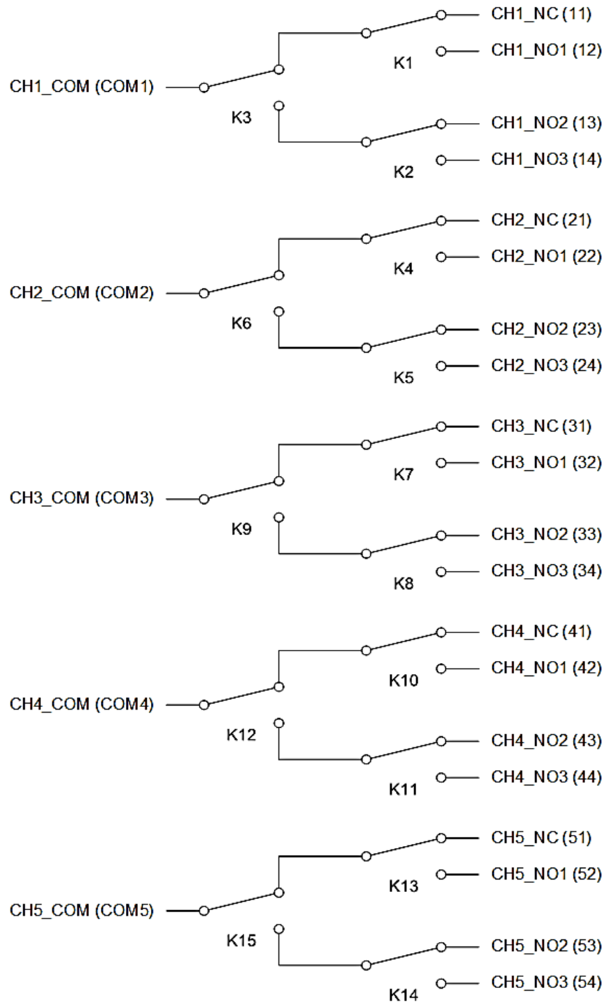
FIGURE 3-101: SMX-6111SMB LOGICAL DIAGRAM
