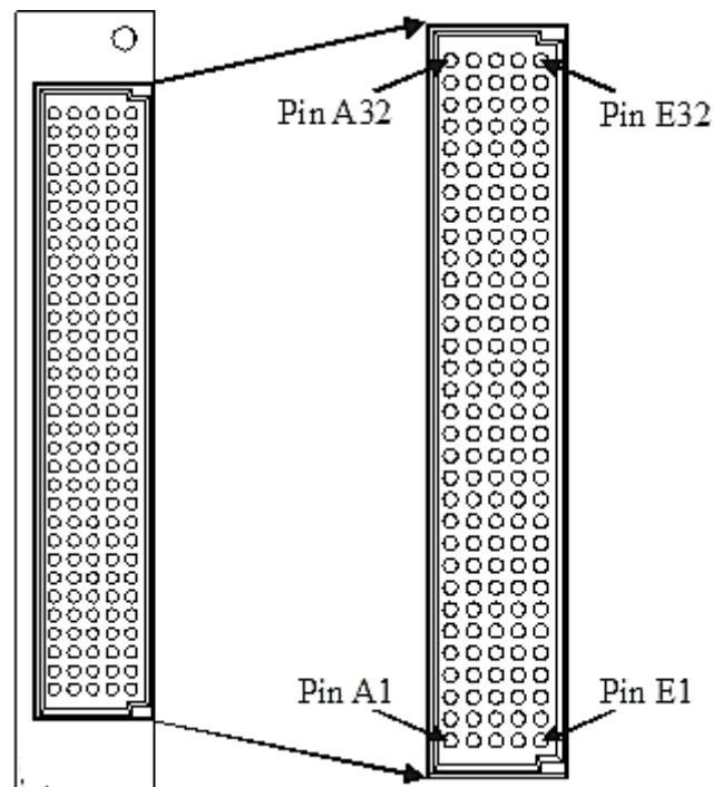
FIGURE 3-45: SMX-3277 FRONT PANEL CONNECTOR (FRONT VIEW)
