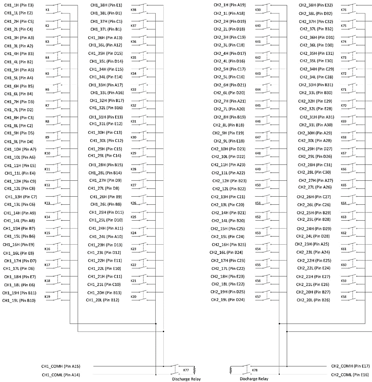
FIGURE 3-52: SMX-3278DS LOGICAL DIAGRAM
