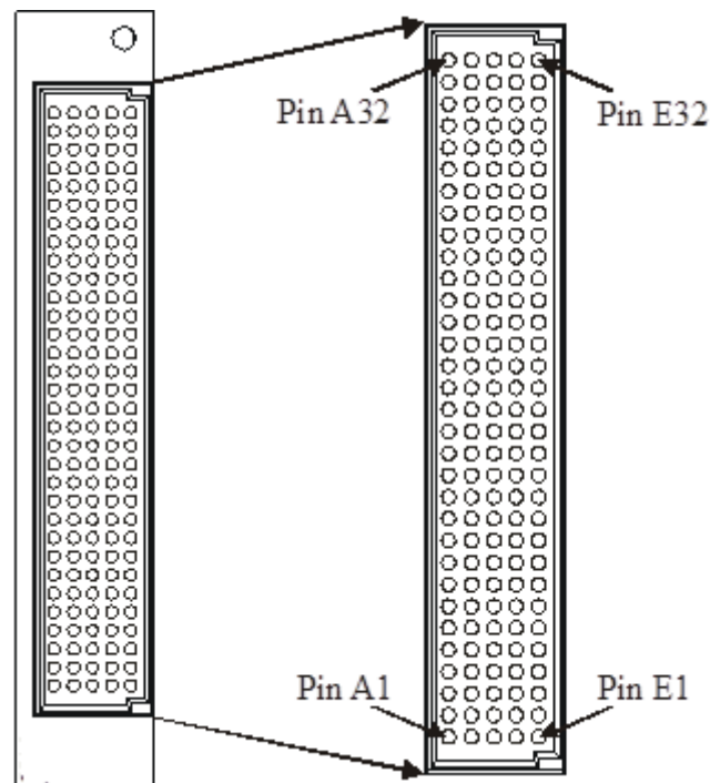
FIGURE 3-49: SMX-3278 FRONT PANEL CONNECTOR (FRONT VIEW)
