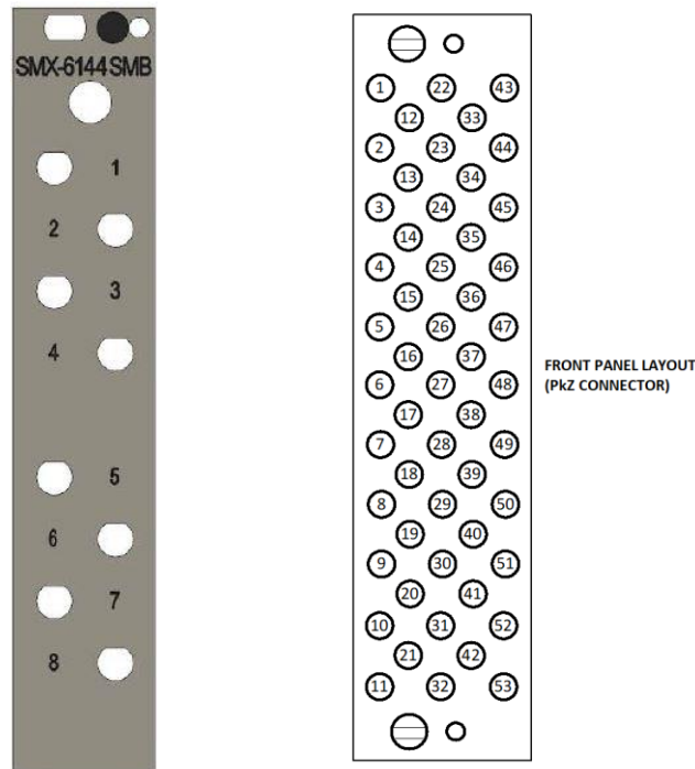
FIGURE 3-139: SMX-6144 FRONT PANEL LAYOUT (SMB CONNECTOR -LEFT IMAGE, PkZ CONNECTOR- RIGHT IMAGE)
