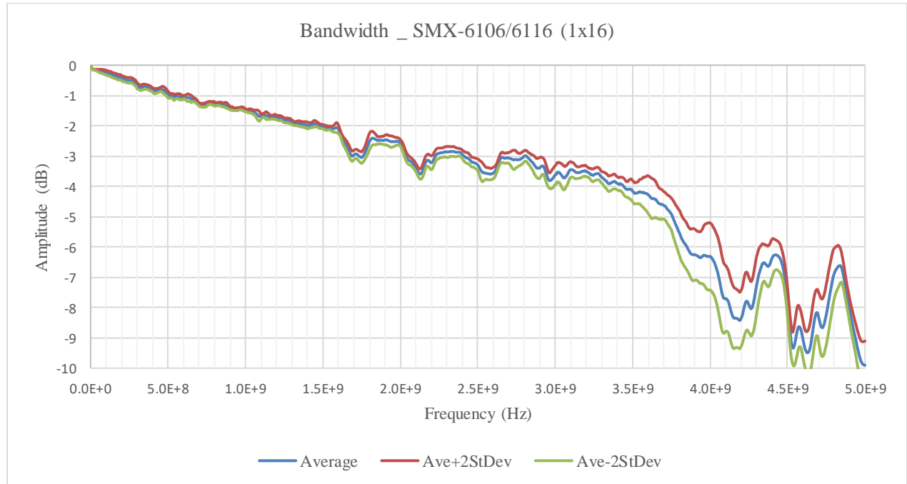
FIGURE 3-116: SMX-6116PKZ BANDWIDTH GRAPH
