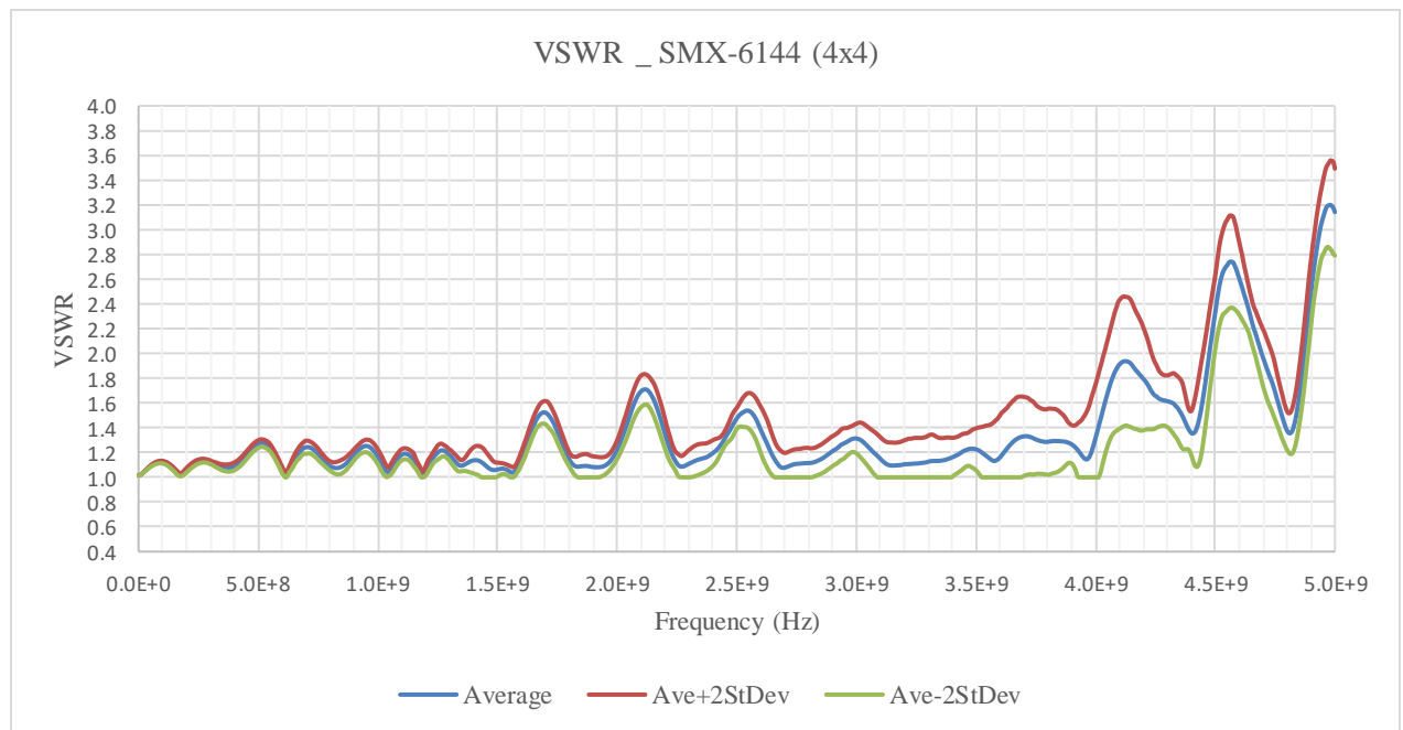
FIGURE 3-145: SMX-6144PkZ VSWR GRAPH
