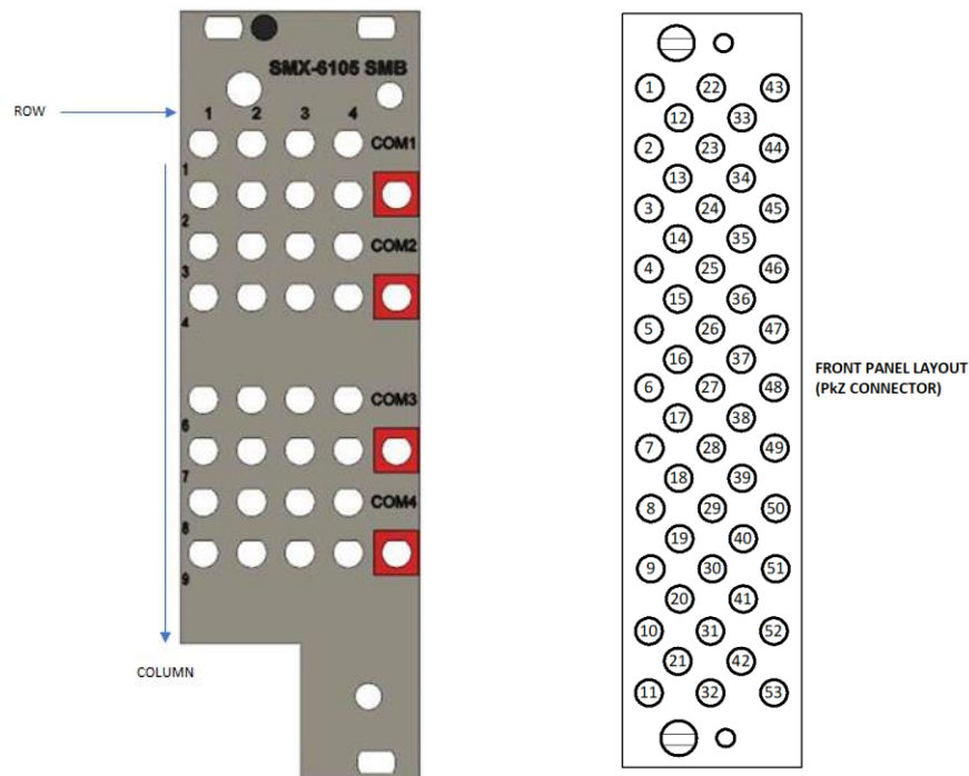
FIGURE 3-118: SMX-6105 FRONT PANEL LAYOUT (SMB CONNECTOR -LEFT IMAGE, PkZ CONNECTOR- RIGHT IMAGE)
