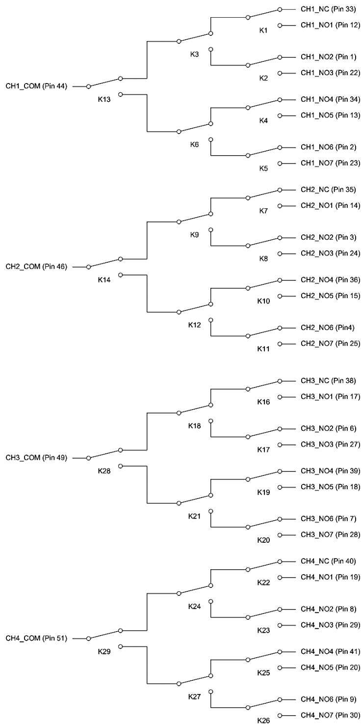
FIGURE 3-119: SMX-6105PkZ LOGICAL DIAGRAM
