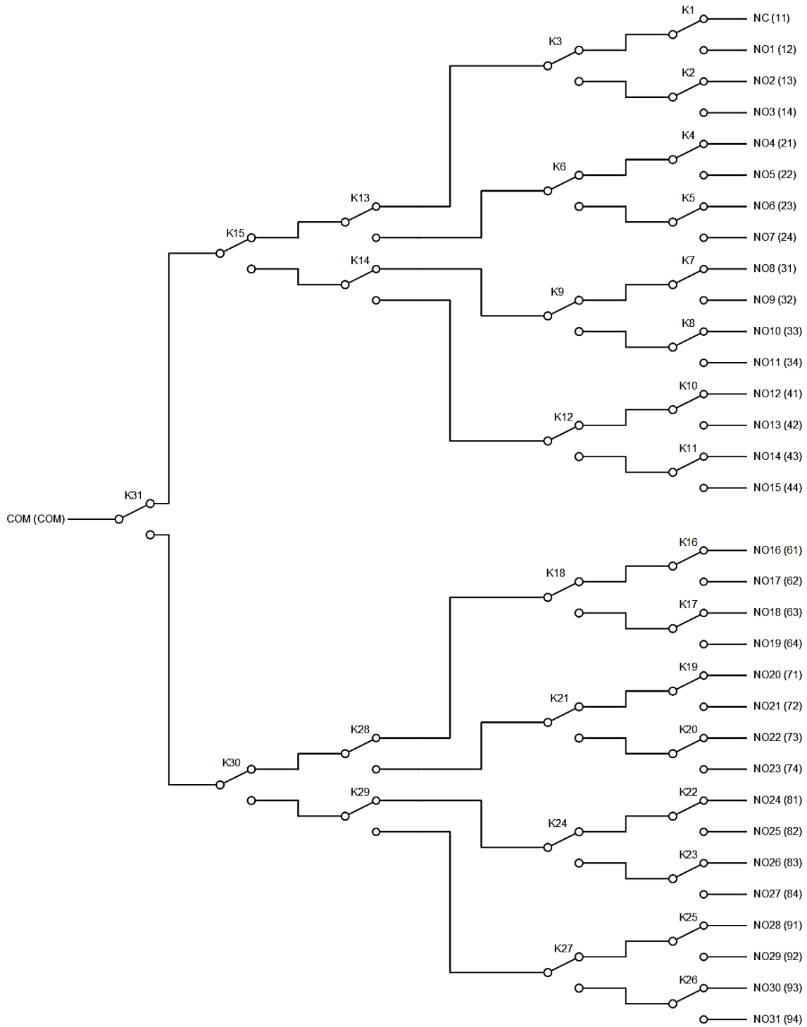
FIGURE 3-134: SMX-6103SMB LOGICAL DIAGRAM
