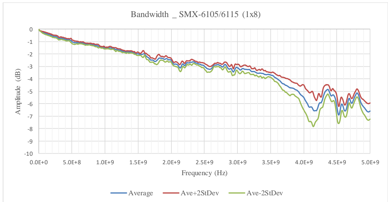
FIGURE 3-129: SMX-6115PkZBANDWIDTH GRAPH
