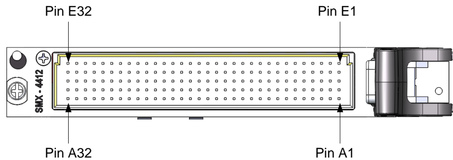
FIGURE 3-77: SMX-4412 FRONT PANEL (FRONT VIEW)
