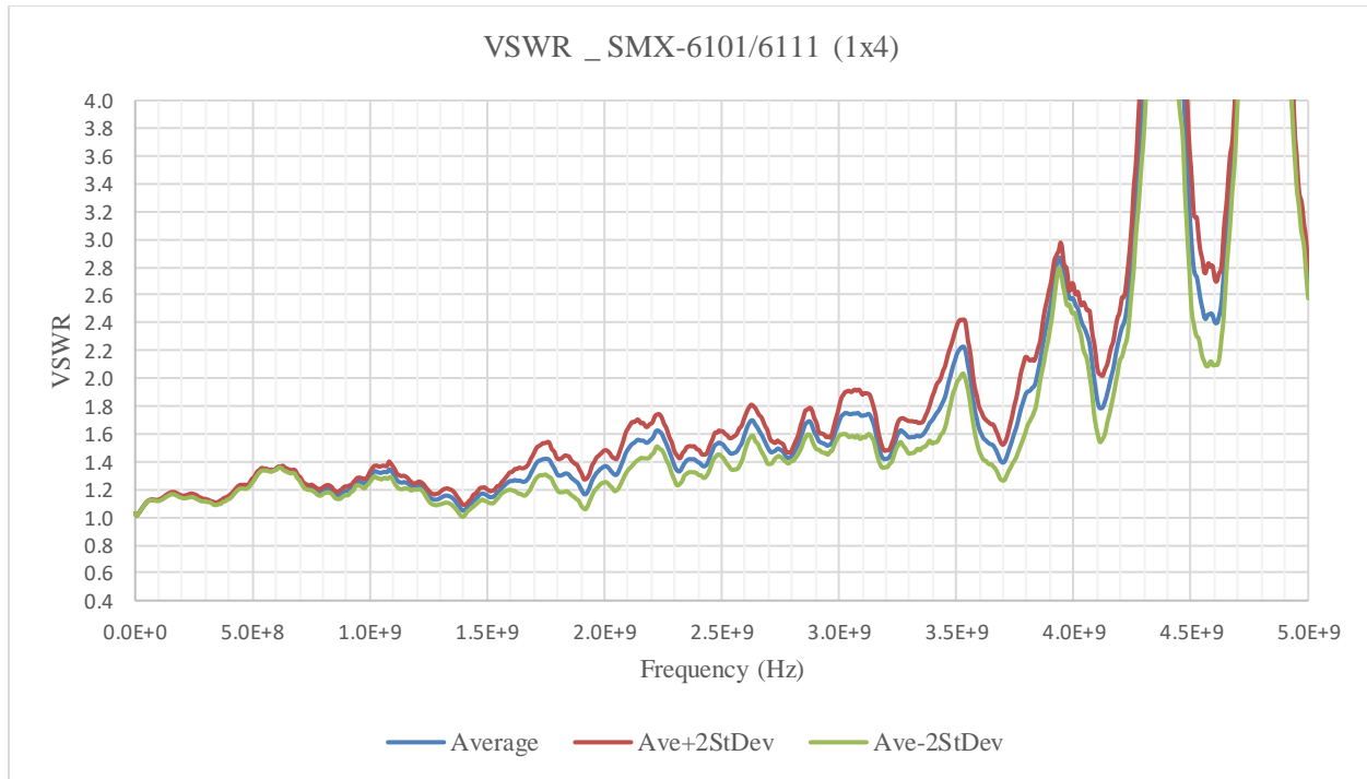
FIGURE 3-97: SMX-6101 SMB VSWR GRAPH
