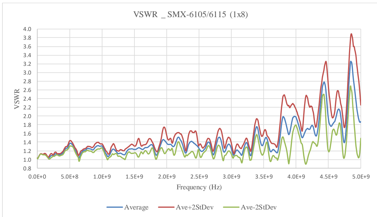
FIGURE 3-123: SMX-6105SMB VSWR GRAPH
