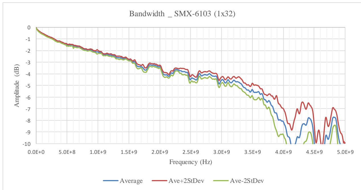
FIGURE 3-136: SMX-6103PKZ BANDWIDTH GRAPH
