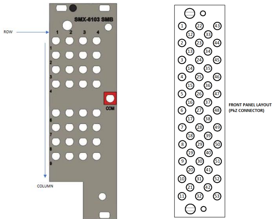
FIGURE 3-132: SMX-6103 FRONT PANEL LAYOUT (SMB CONNECTOR -LEFT IMAGE, PkZ CONNECTOR- RIGHT IMAGE)
