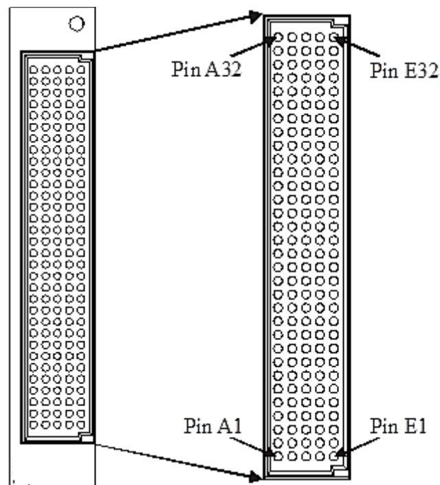
FIGURE 3-21: SMX-3002 FRONT PANEL CONNECTOR PINS (FRONT VIEW)
