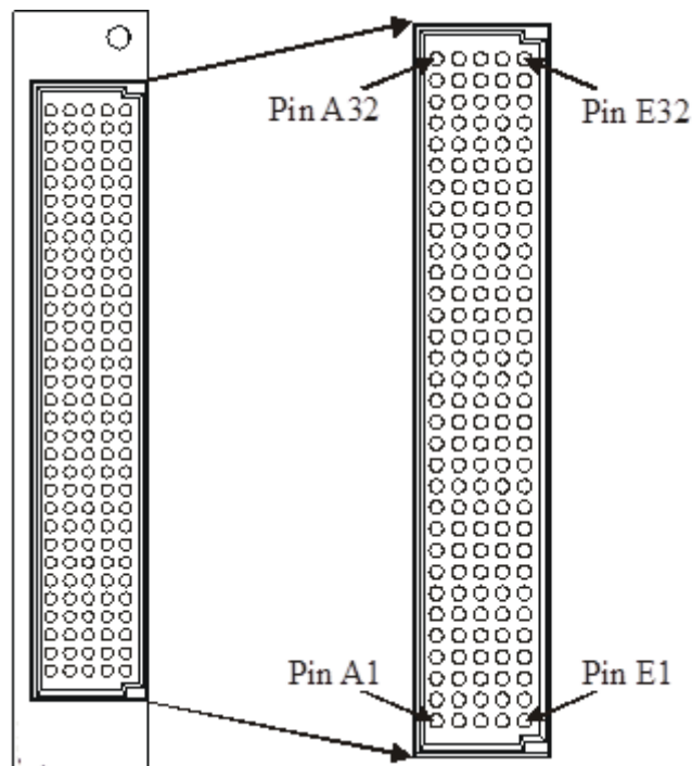
FIGURE 3-23: SMX-3002DS FRONT PANEL (FRONT VIEW)
