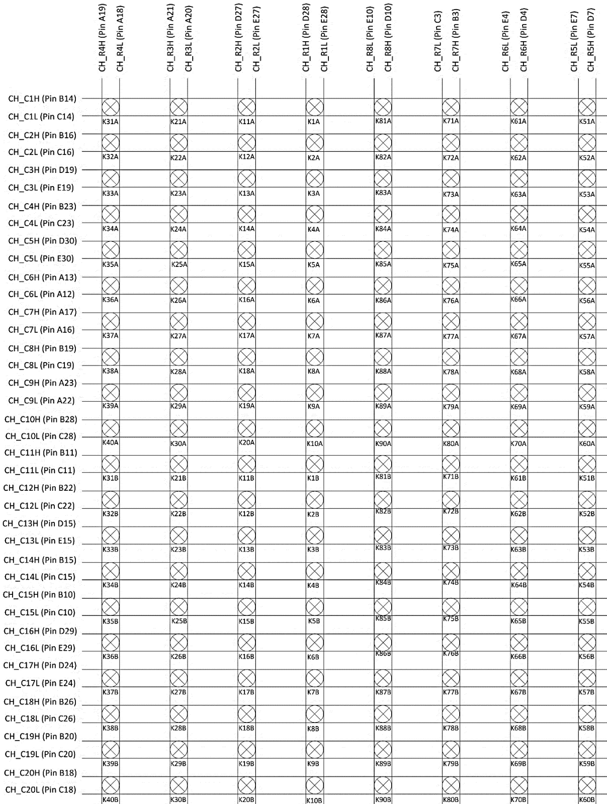
FIGURE 3-84: SMX-4415 LOGICAL DIAGRAM
