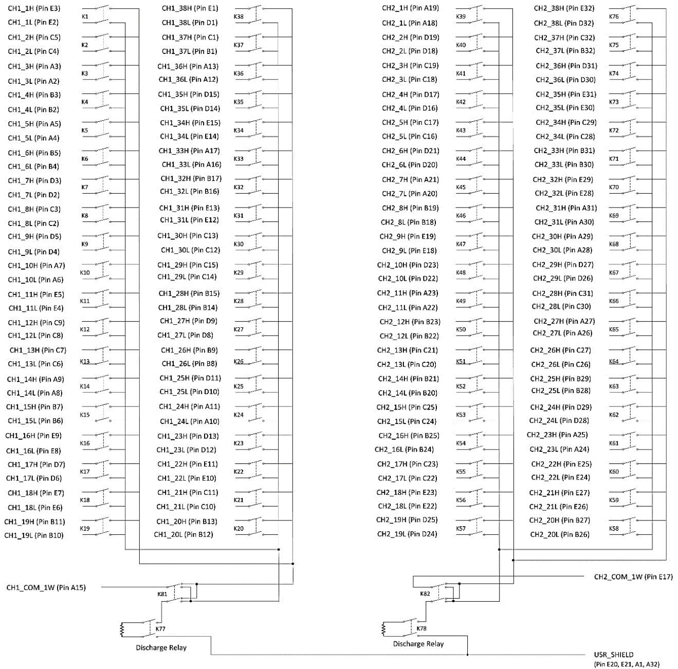
FIGURE 3-48: SMX-3277DS LOGICAL DIAGRAM
