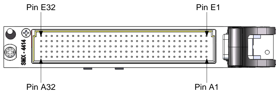
FIGURE 3-81: SMX-4414 FRONT PANEL (FRONT VIEW)
