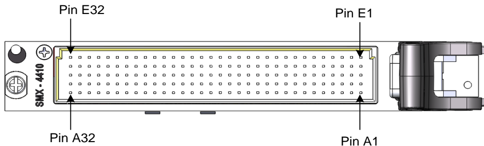
FIGURE 3-75: SMX-4411 FRONT PANEL (FRONT VIEW)
