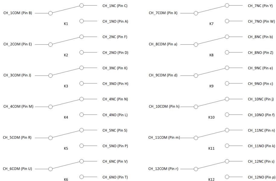
FIGURE 3-14: SMX-2002-12 LOGICAL DIAGRAM
