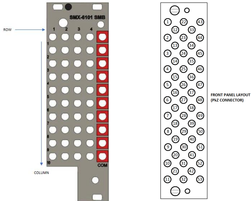
FIGURE 3-92: SMX-6101 FRONT PANEL LAYOUT (SMB CONNECTOR -LEFT IMAGE, PkZ CONNECTOR- RIGHT IMAGE)
