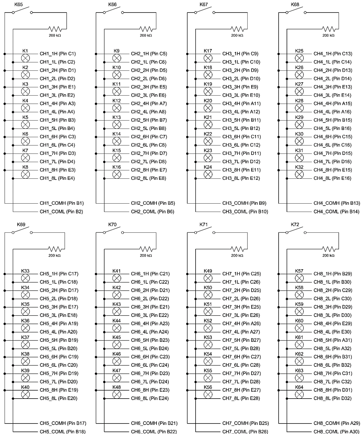
FIGURE 3-24: SMX-3002DS LOGICAL DIAGRAM
