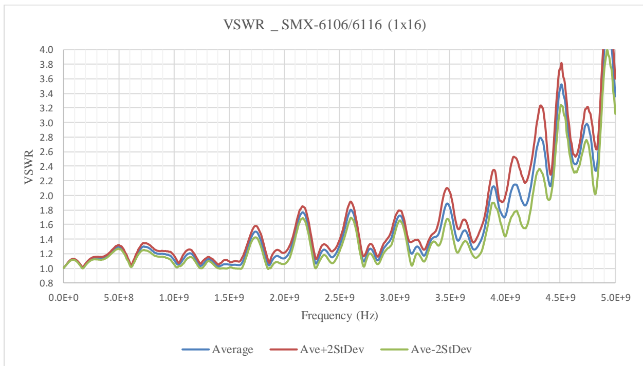
FIGURE 3-117: SMX-6116SMB AND PkZ VSWR GRAPH
