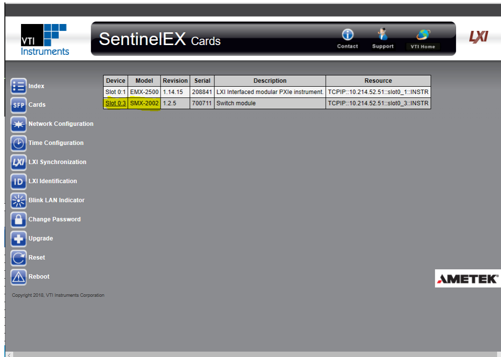
FIGURE 3-131: SFP SWITCH CARD SELECTION
