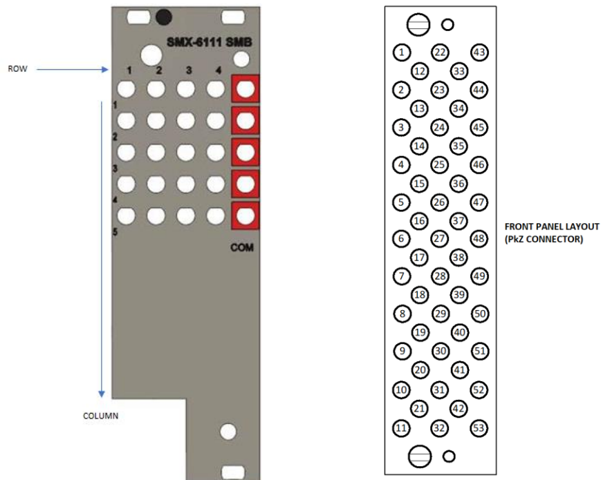
FIGURE 3-99: SMX-6111 FRONT PANEL LAYOUT(SMB CONNECTOR -LEFT IMAGE, PkZ CONNECTOR- RIGHT IMAGE)
