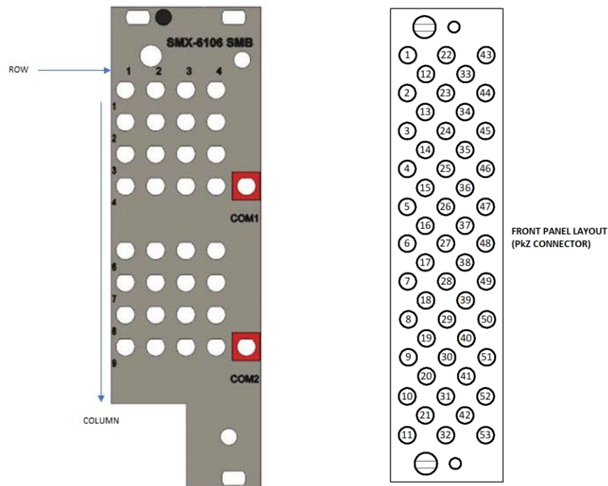
FIGURE 3-106: SMX-6106 FRONT PANEL LAYOUT (SMB CONNECTOR -LEFT IMAGE, PkZ CONNECTOR- RIGHT IMAGE)
