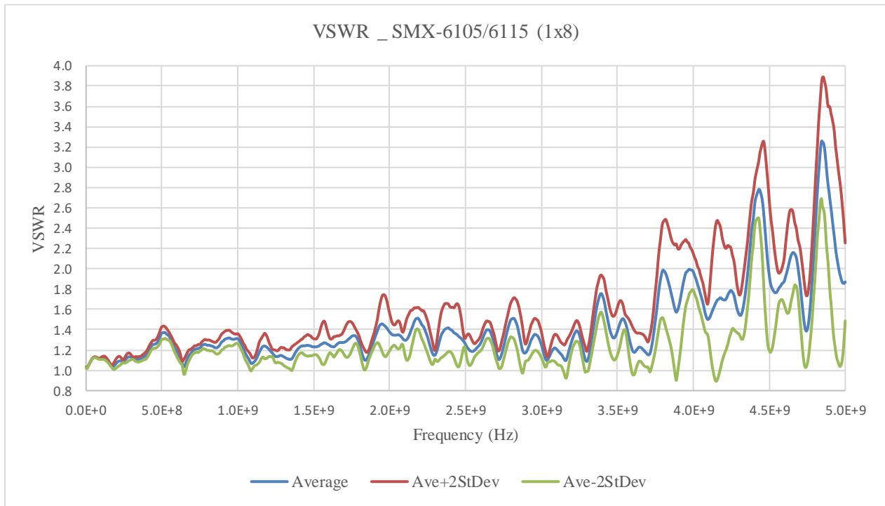
FIGURE 3-130: SMX-6115SMB VSWR GRAPH
