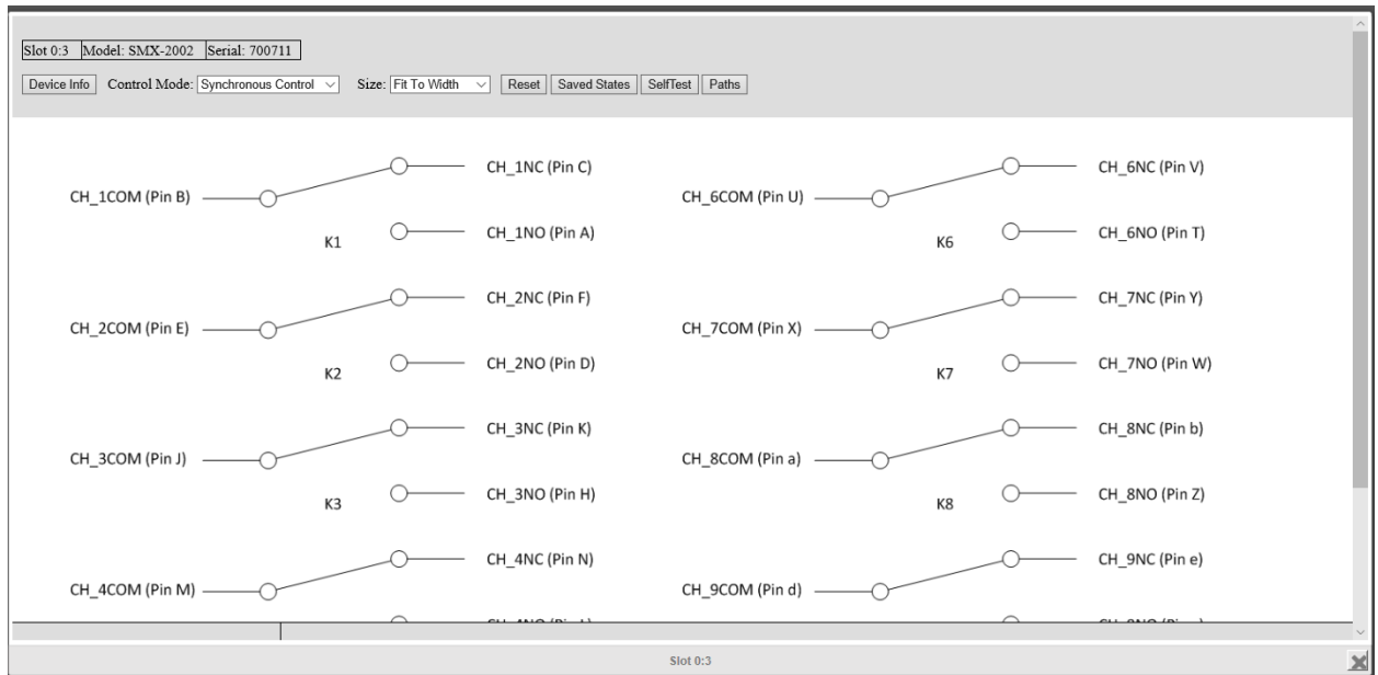
FIGURE 3-148: SMX-2002 SWITCH CARD SFP PAGE
