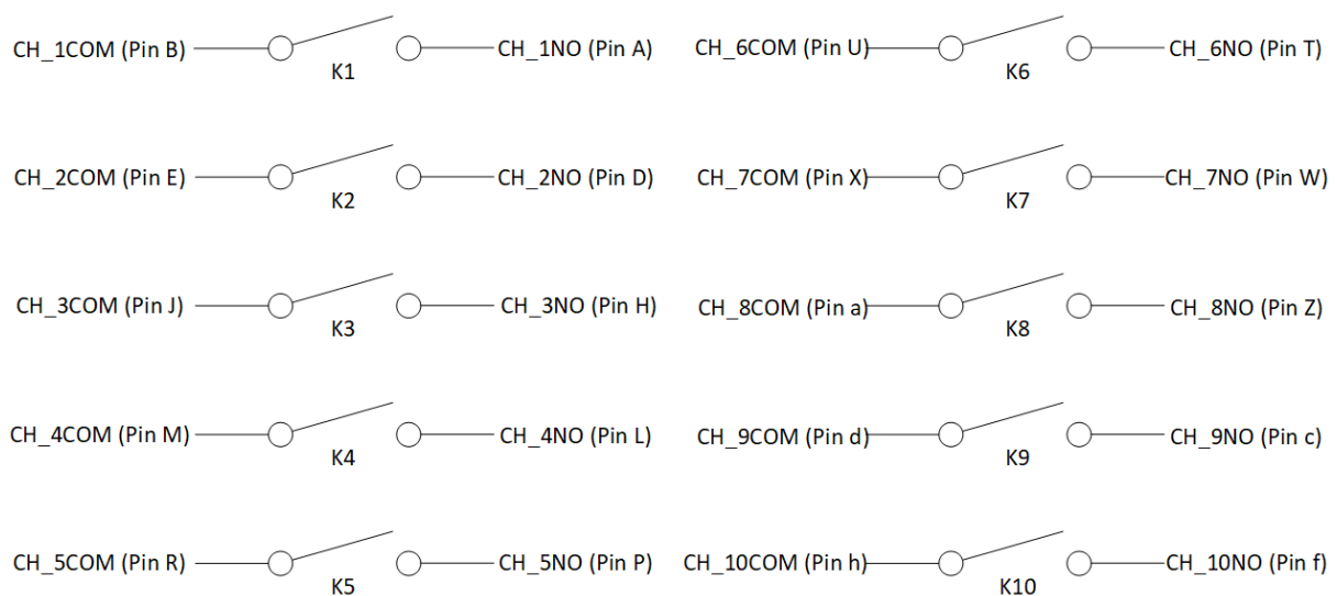
Figure 3-2: SMX-2001-10 Logical Diagram
