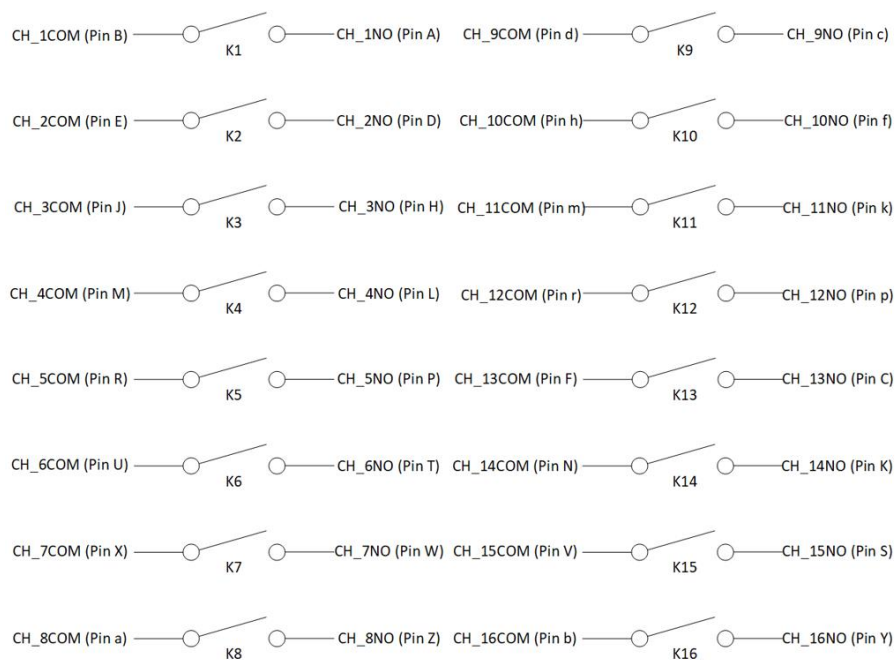
FIGURE 3-8: SMX-2001-16 LOGICAL DIAGRAM
