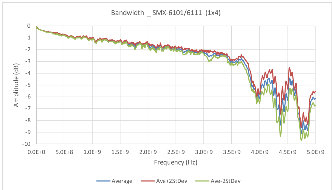
FIGURE 3-95: SMX-6101 SMB BANDWIDTH GRAPH
