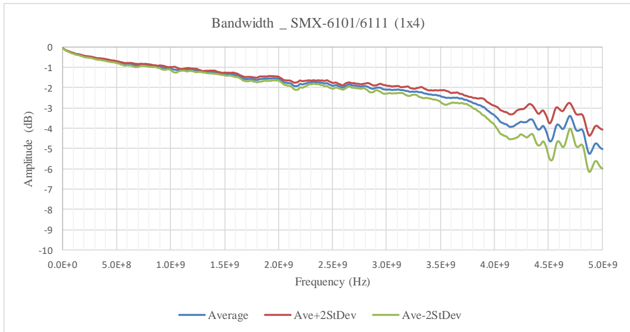
FIGURE 3-103: SMX-6111PKZ BANDWIDTH GRAPH
