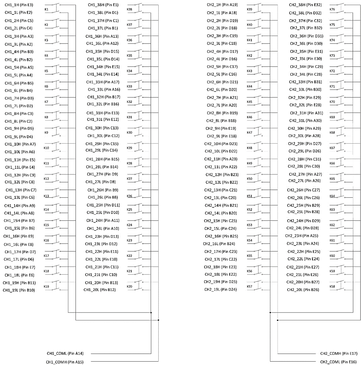
FIGURE 3-50: SMX-3278 LOGICAL DIAGRAM
