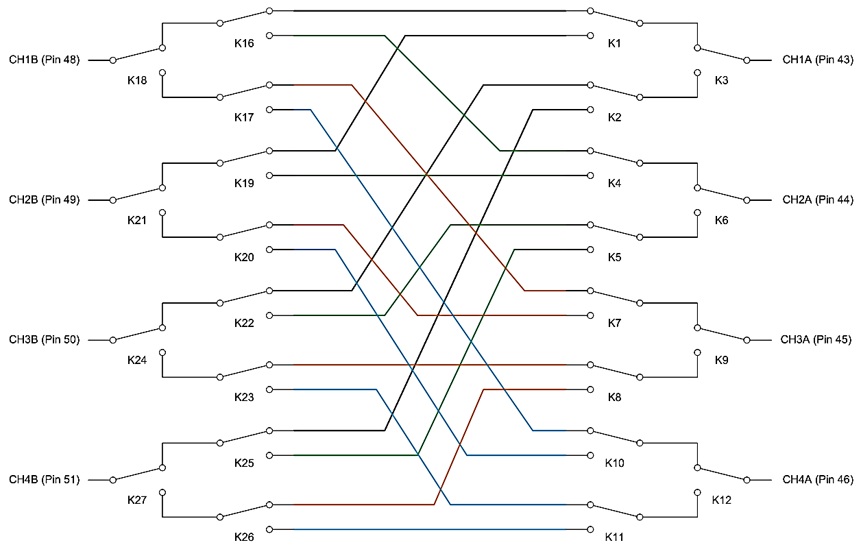
FIGURE 3-140: SMX-6144PkZ LOGICAL DIAGRAM
