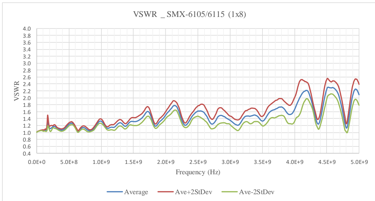
FIGURE 3-124: SMX-6105PkZ VSWR GRAPH
