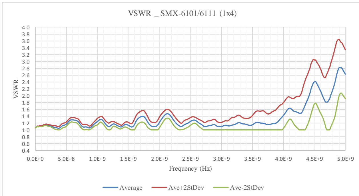
FIGURE 3-98: SMX-6101 PkZ VSWR GRAPH
