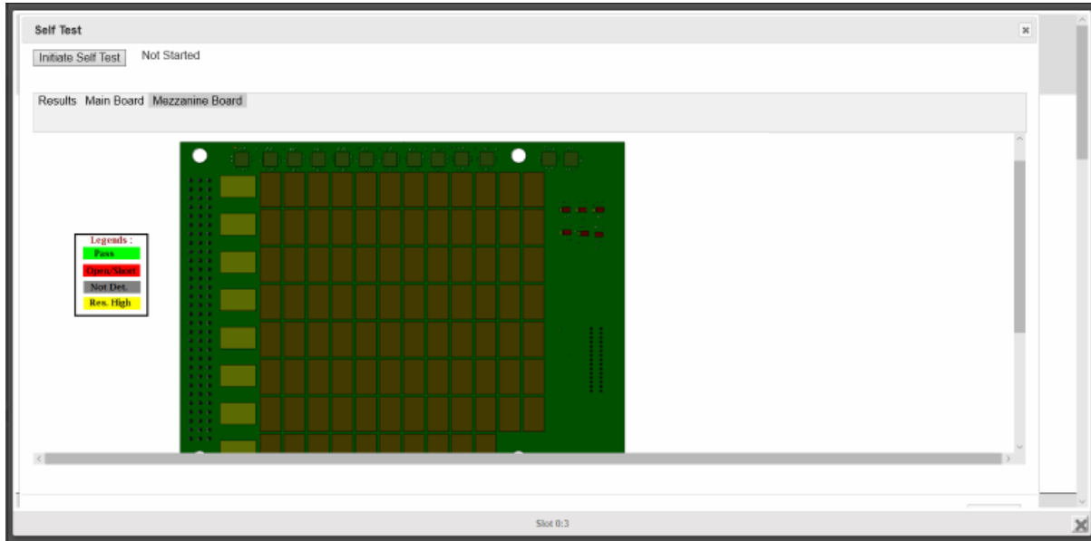
FIGURE 3-67: SMX-4410SELFTTEST-MEZZANINE BOARD RELAY LOCATION PAGE
