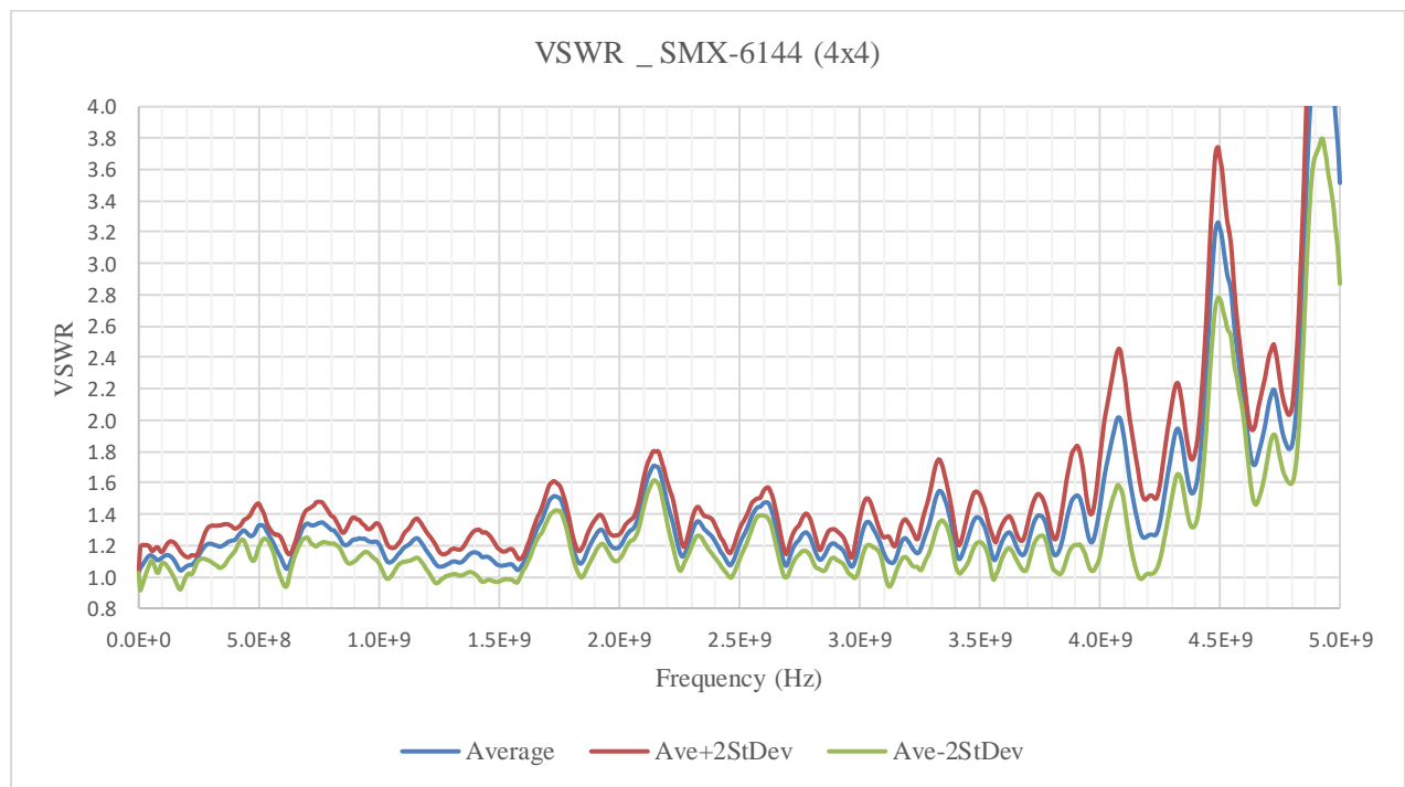
FIGURE 3-144: SMX-6144SMB VSWR GRAPH
