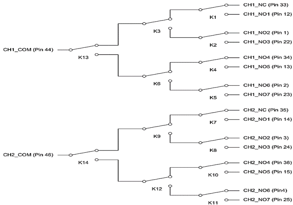
FIGURE 3-126: SMX-6115PkZ LOGICAL DIAGRAM
