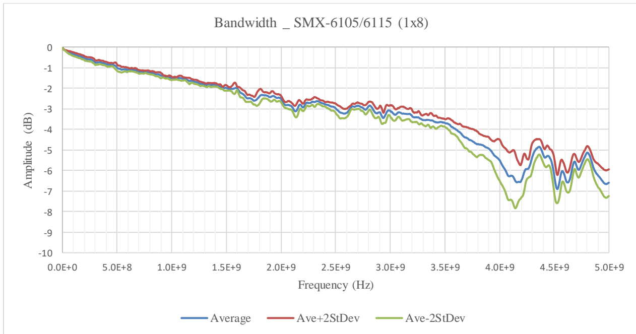
FIGURE 3-122: SMX-6105PkZ BANDWIDTH GRAPH
