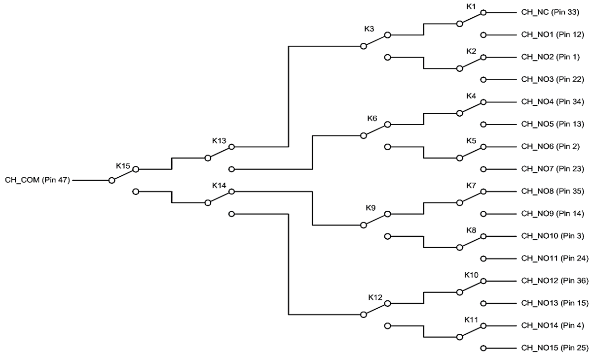
FIGURE 3-113: SMX-6116PkZ LOGICAL DIAGRAM
