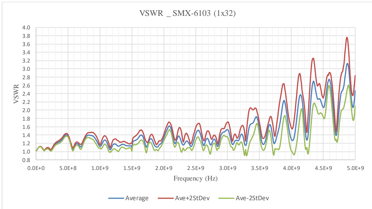
FIGURE 3-137: SMX-6103SMB VSWR GRAPH
