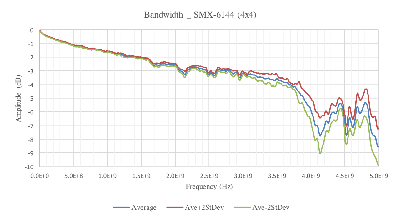
FIGURE 3-143: SMX-6144PkZBANDWIDTH GRAPH
