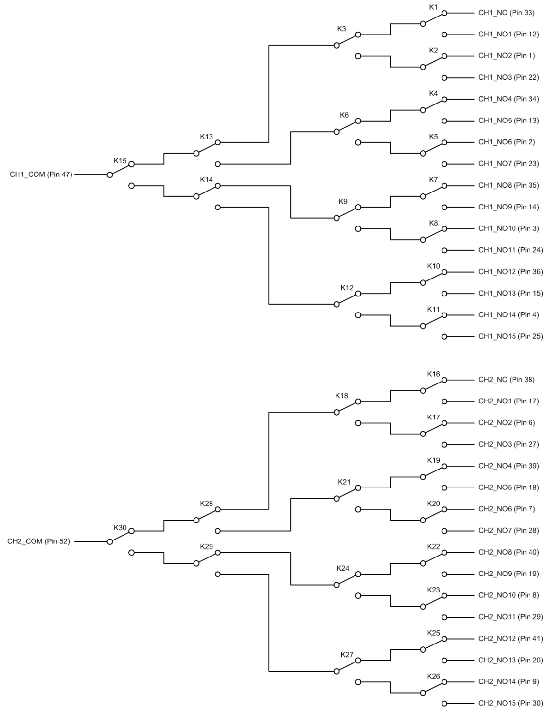
FIGURE 3-107: SMX-6106PkZ LOGICAL DIAGRAM
