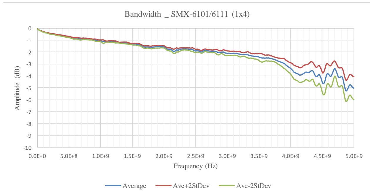
FIGURE 3-96: SMX-6101 PkZ BANDWIDTH GRAPH
