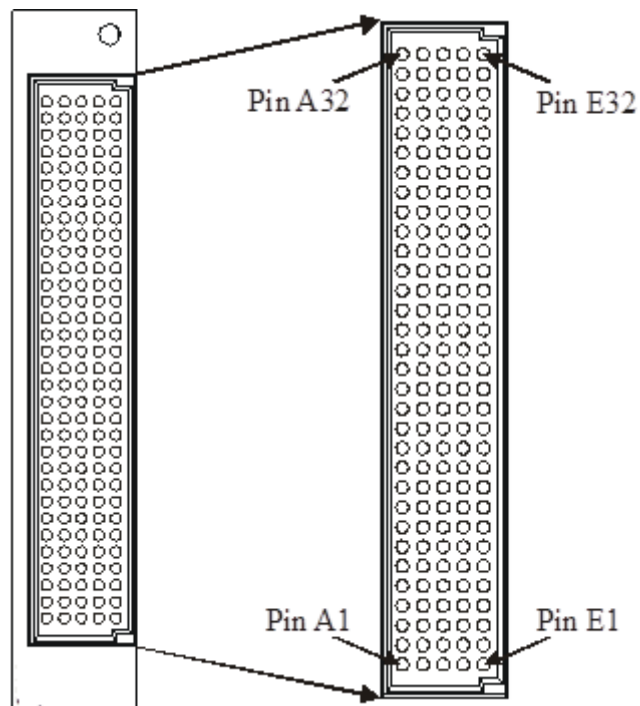
FIGURE 3-37: SMX-3006 FRONT PANEL CONNECTOR PINS (FRONT VIEW)
