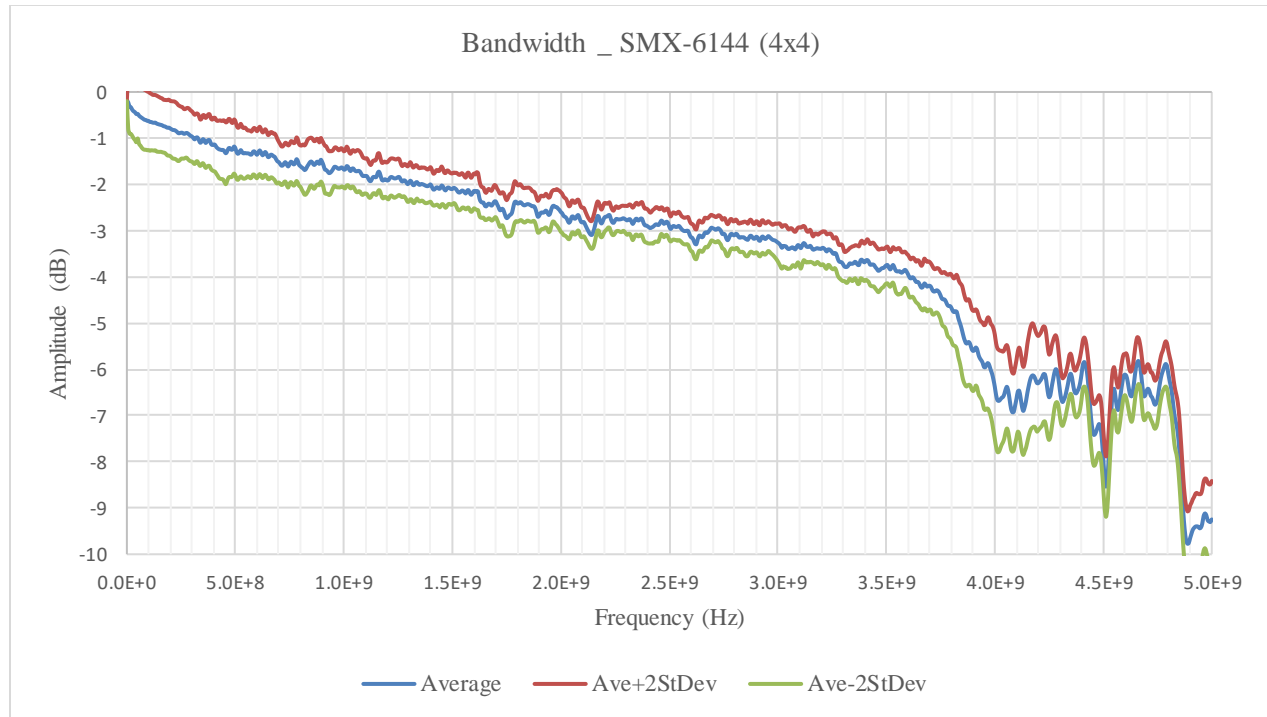
FIGURE 3-142: SMX-6144SMBBANDWIDTH GRAPH
