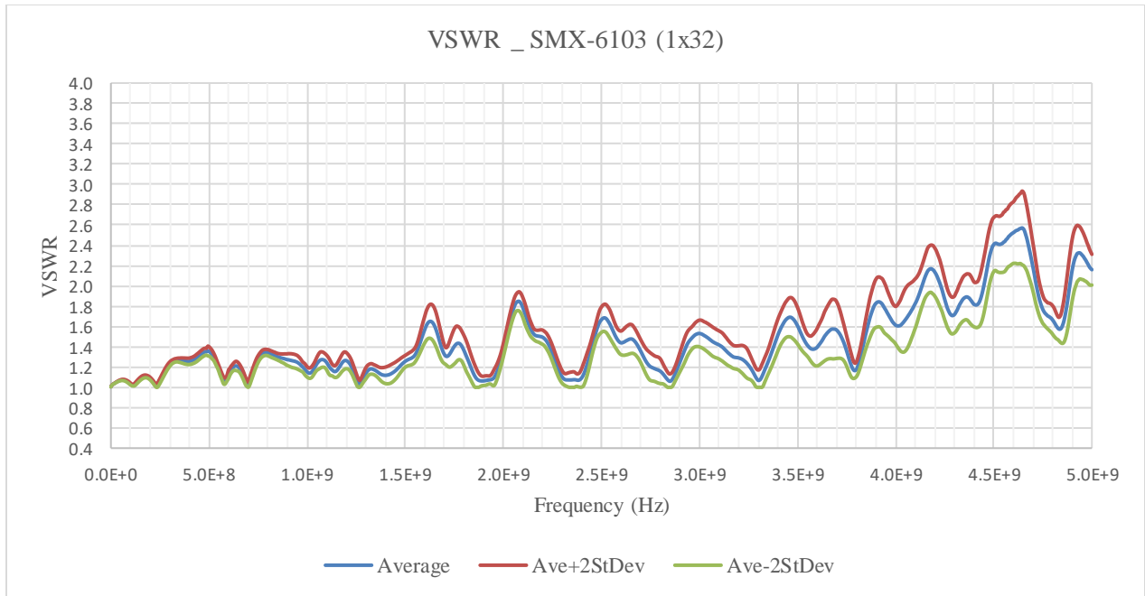
FIGURE 3-138: SMX-6103PKZ VSWR GRAPH
