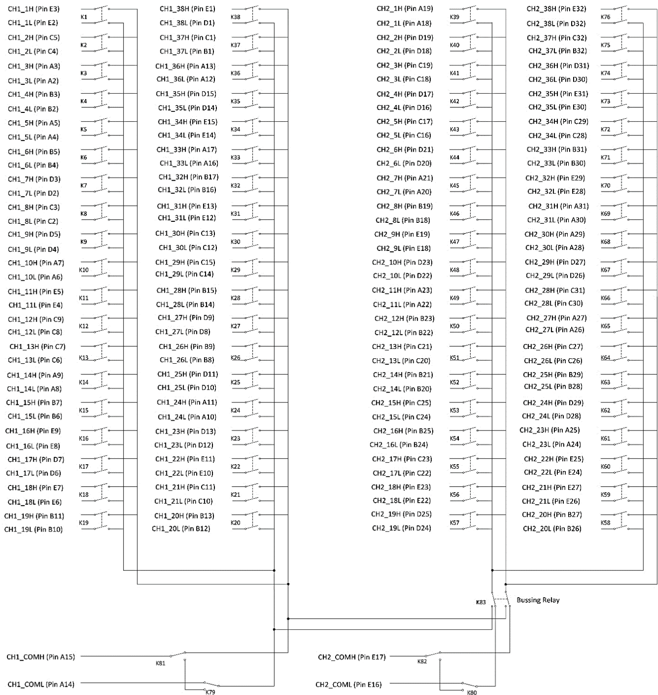
FIGURE 3-42: SMX-3276 LOGICAL DIAGRAM
