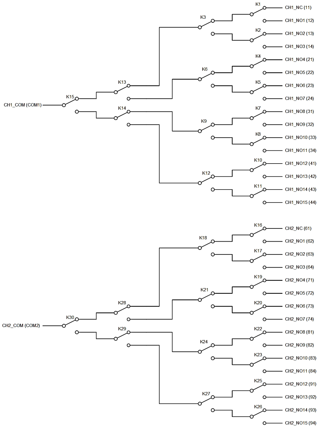
FIGURE 3-108: SMX-6106SMB LOGICAL DIAGRAM
