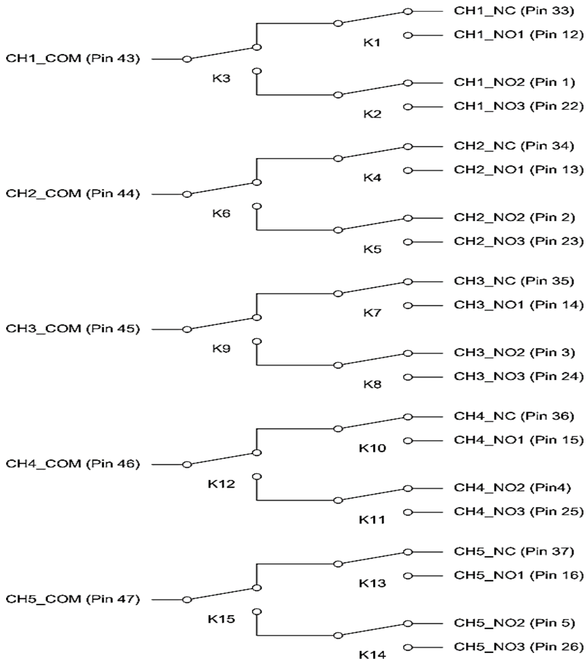
FIGURE 3-100: SMX-6111PkZ LOGICAL DIAGRAM
