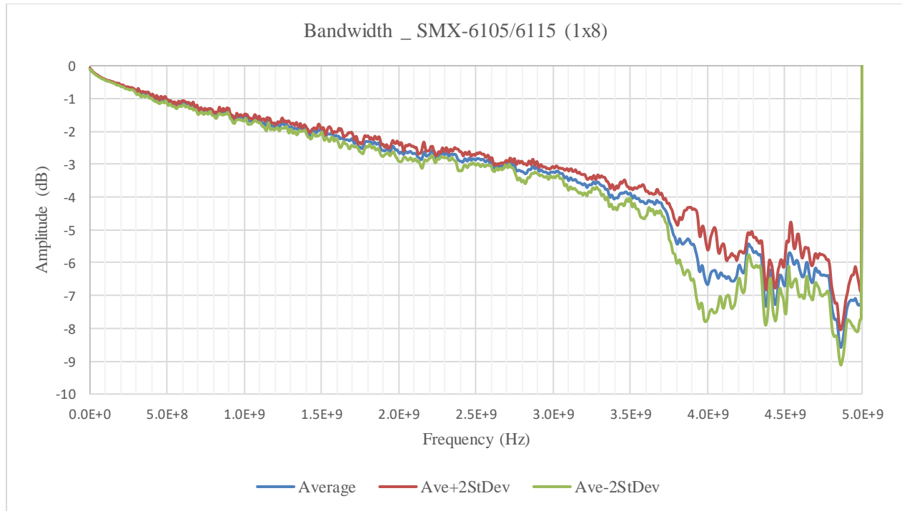
FIGURE 3-121: SMX-6105SMB BANDWIDTH GRAPH
