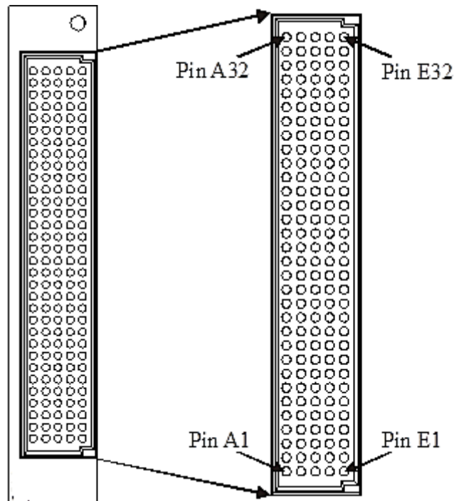
FIGURE 3-31: SMX-3004DS FRONT PANEL (FRONT VIEW)
