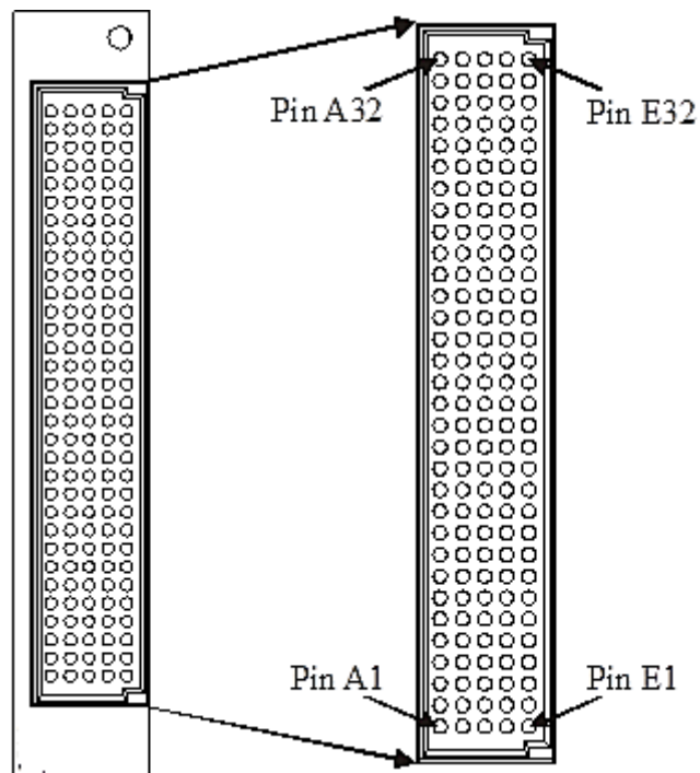
FIGURE 3-39: SMX-3007 FRONT PANEL CONNECTOR PINS (FRONT VIEW)
