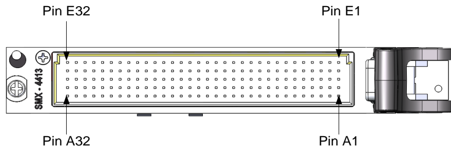
FIGURE 3-79: SMX-4413 FRONT PANEL (FRONT VIEW)
