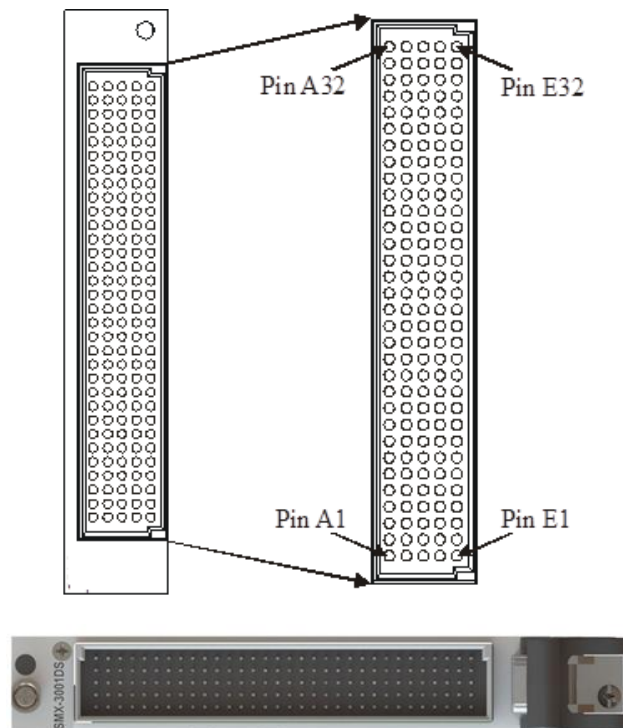
FIGURE 3-18: SMX-3001DS FRONT PANEL (FRONT VIEW)
