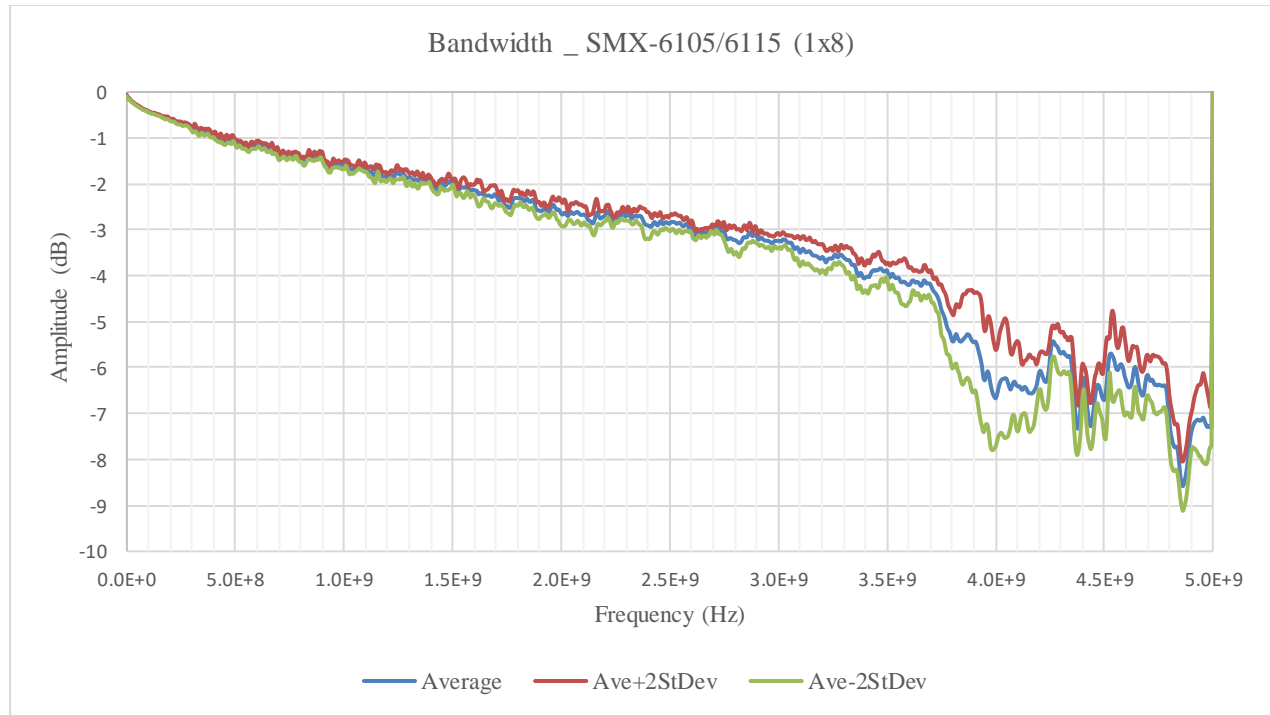
FIGURE 3-128: SMX-6115SMBBANDWIDTH GRAPH
