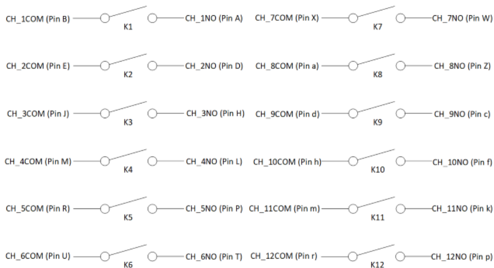
FIGURE 3-5: SMX-2001-12 LOGICAL DIAGRAM
