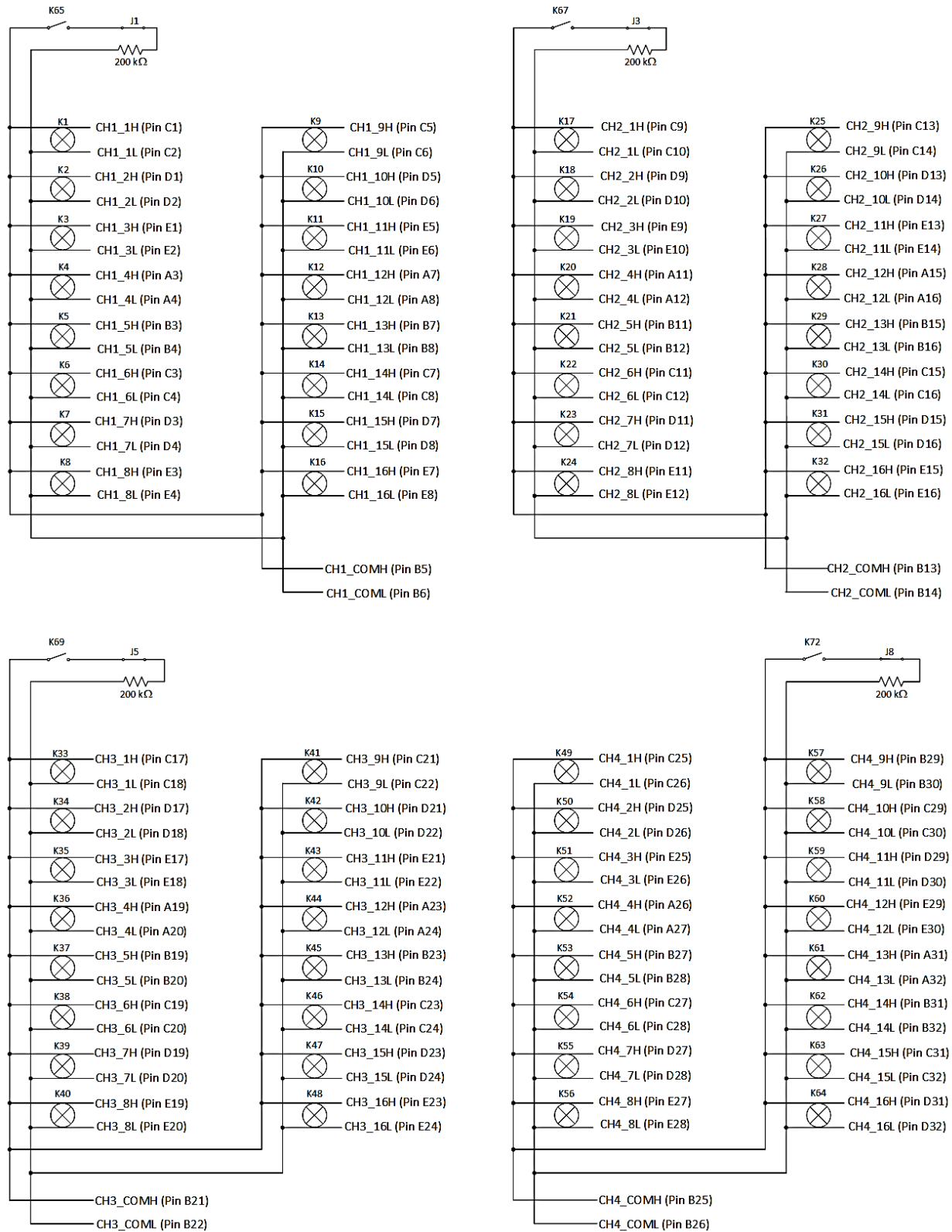
FIGURE 3-28: SMX-3003DS LOGICAL DIAGRAM
