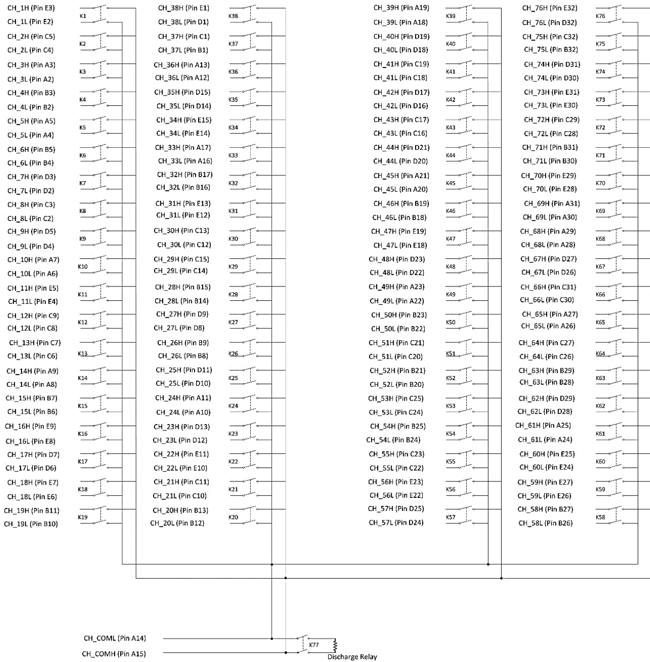
FIGURE 3-56: SMX-3279DS LOGICAL DIAGRAM
