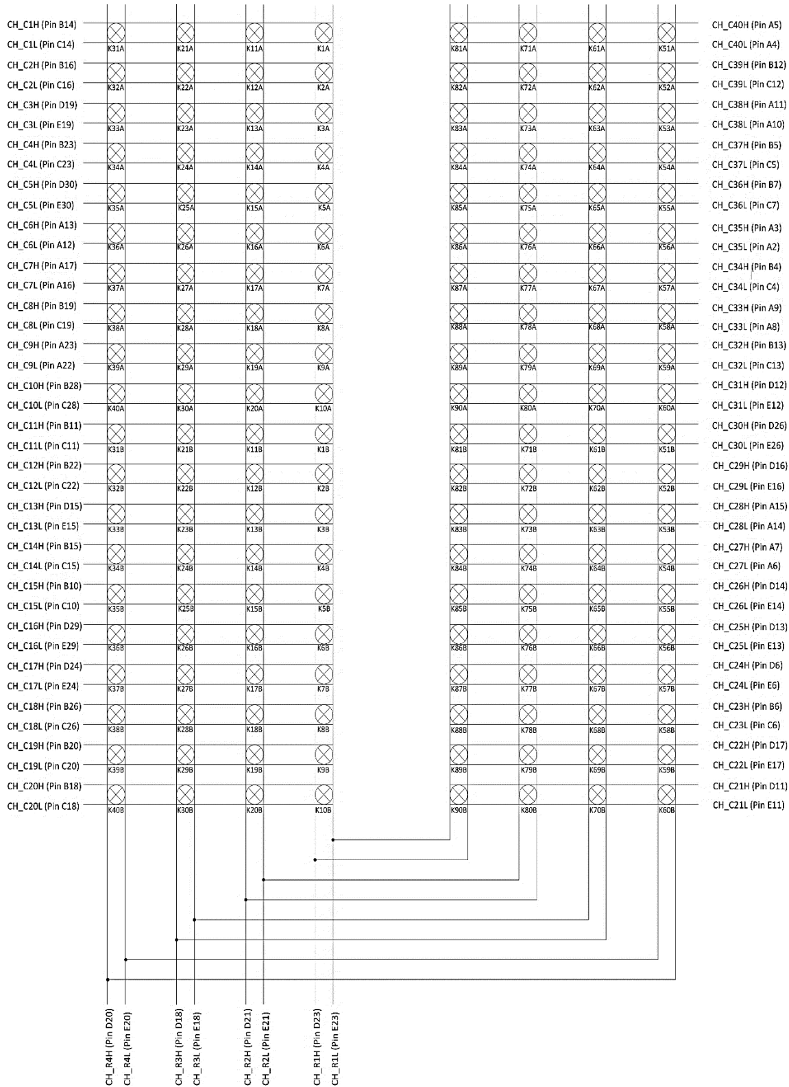
FIGURE 3-80: SMX-4413 LOGICAL DIAGRAM
