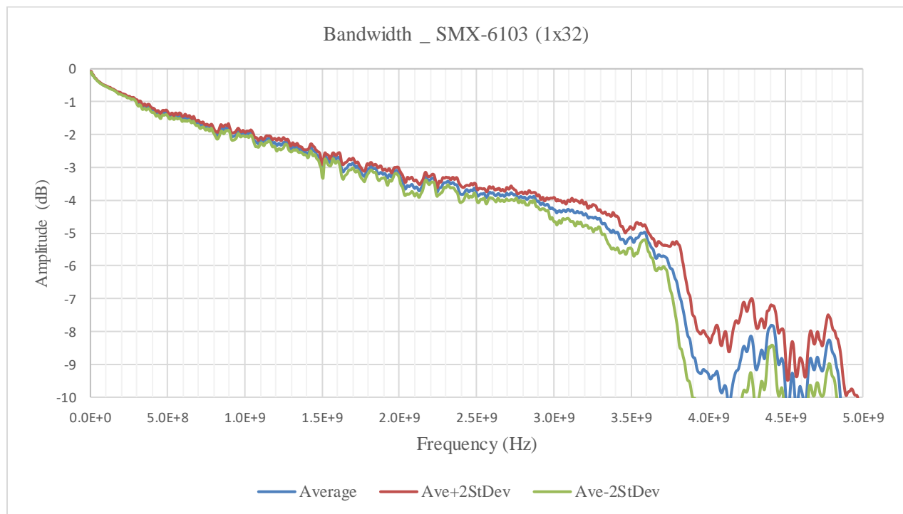
FIGURE 3-135: SMX-6103SMB BANDWIDTH GRAPH
