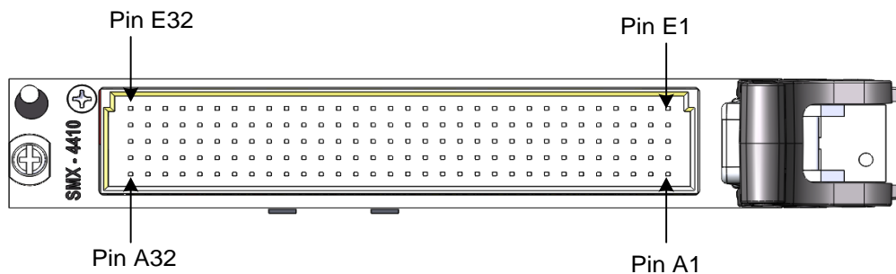
FIGURE 3-61: SMX-4410 FRONT PANEL (FRONT VIEW)
