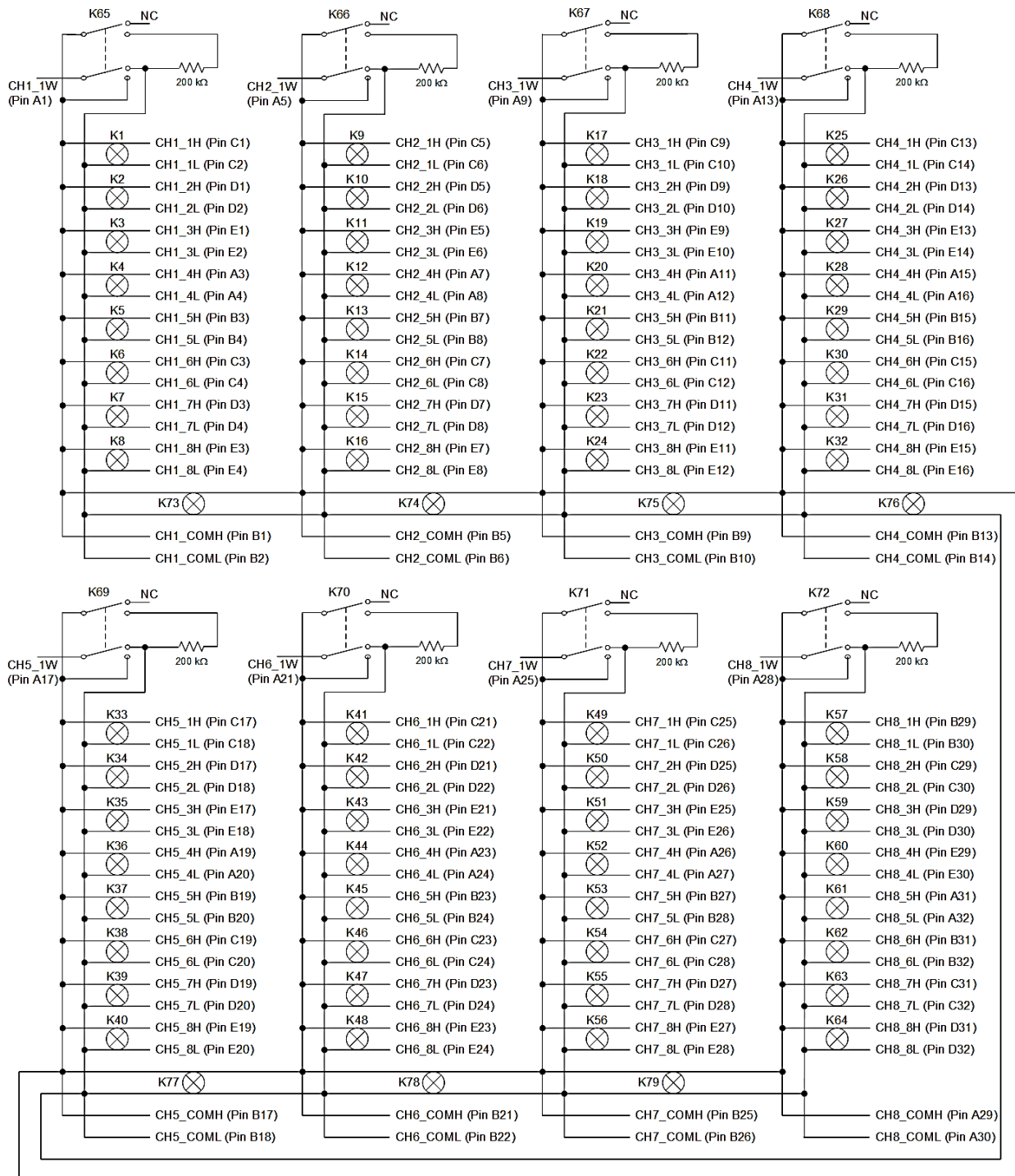
FIGURE 3-20: SMX-3001DS LOGICAL DIAGRAM
