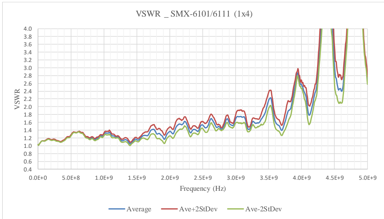
FIGURE 3-104: SMX-6111SMB VSWR GRAPH
