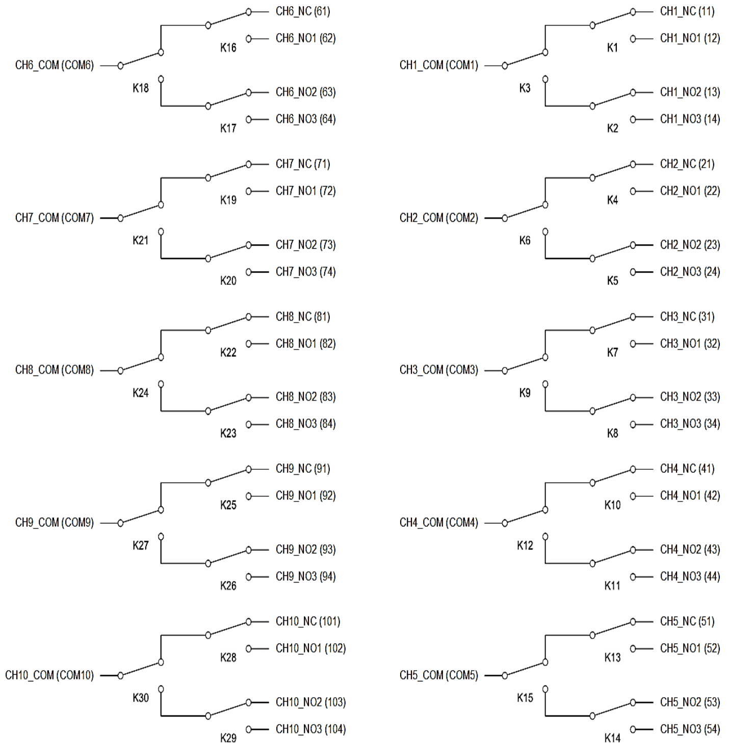
FIGURE 3-94: SMX-6101 SMB LOGICAL DIAGRAM
