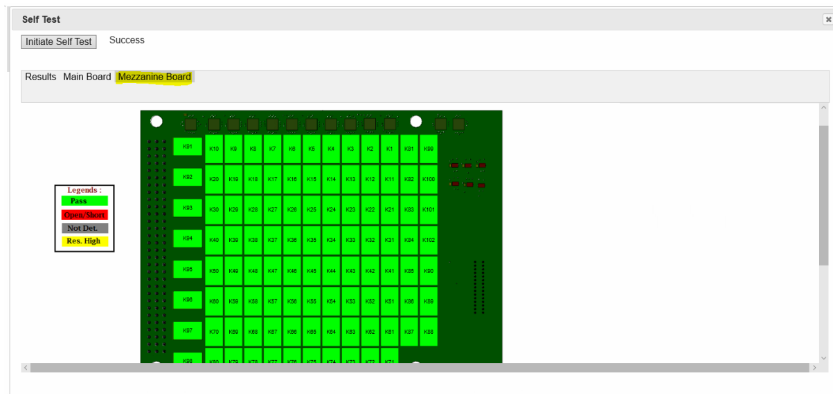
FIGURE 3-74: SMX-4410 SELF-TEST - RELAY LOCATION (MEZZANINE BOARD) SCREEN, POST SELF-TEST INDICATING THE STATUS
