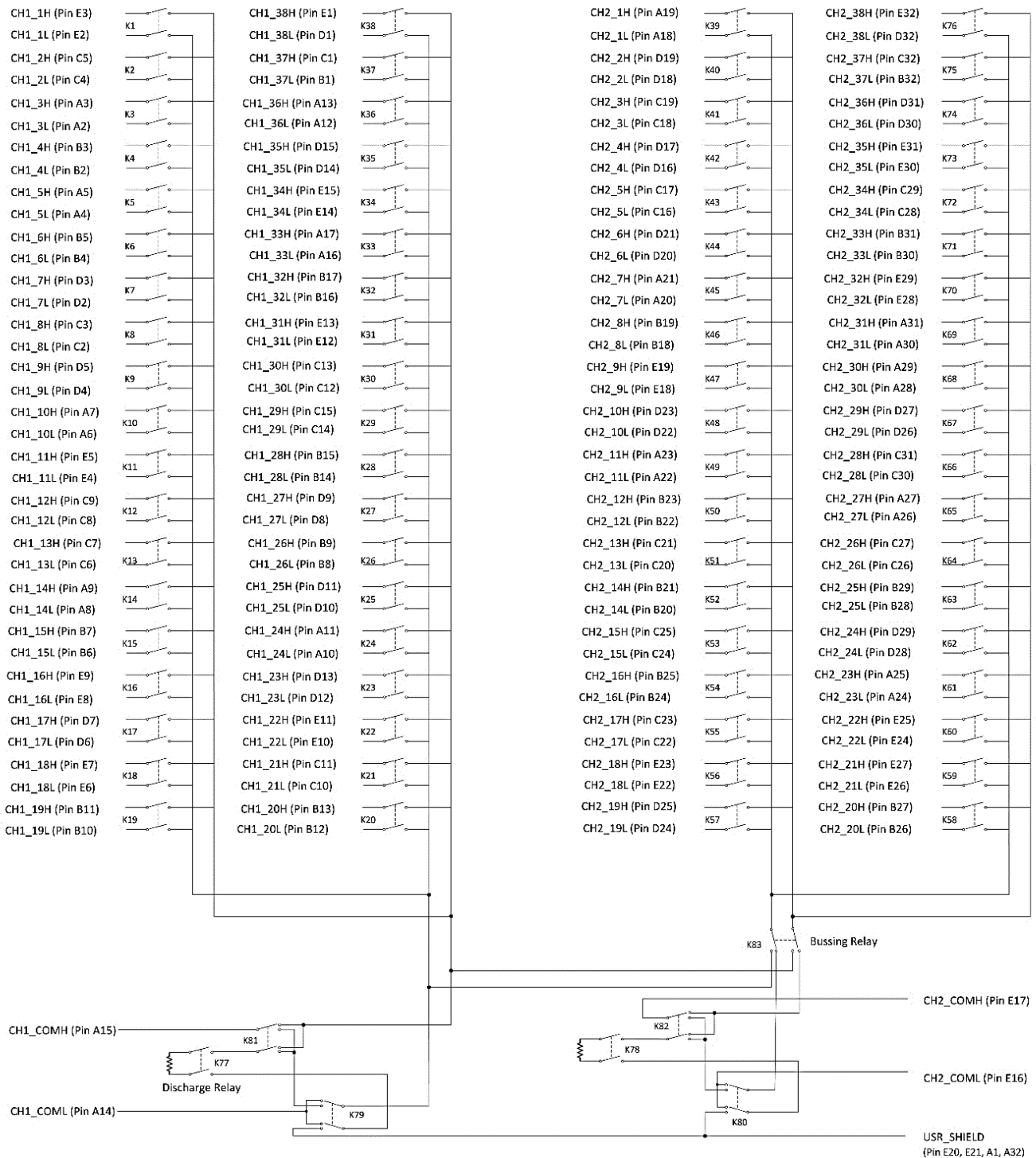
FIGURE 3-44: SMX-3276DS LOGICAL DIAGRAM
