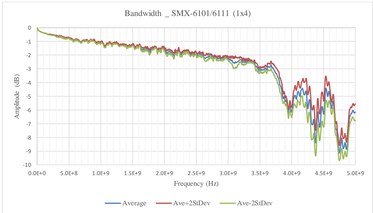
FIGURE 3-102: SMX-6111SMB BANDWIDTH GRAPH
