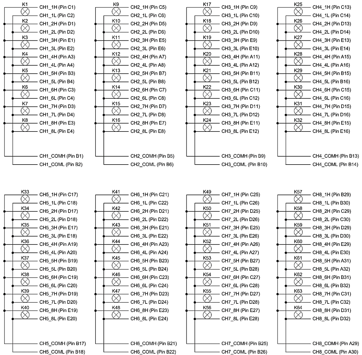
FIGURE 3-22: SMX-3002 LOGICAL DIAGRAM
