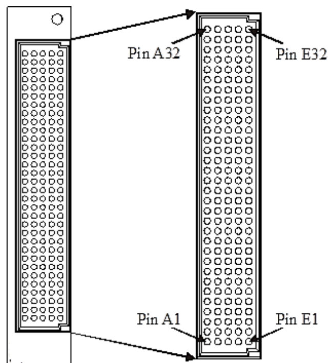
FIGURE 3-33: SMX-3005 FRONT PANEL CONNECTOR PINS (FRONT VIEW)
