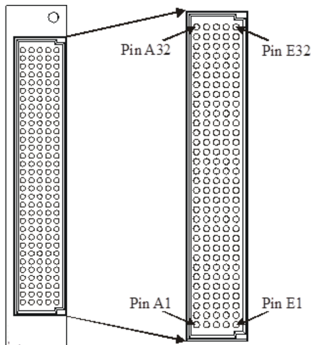
FIGURE 3-55: SMX-3279DS FRONT PANEL CONNECTOR (FRONT VIEW)
