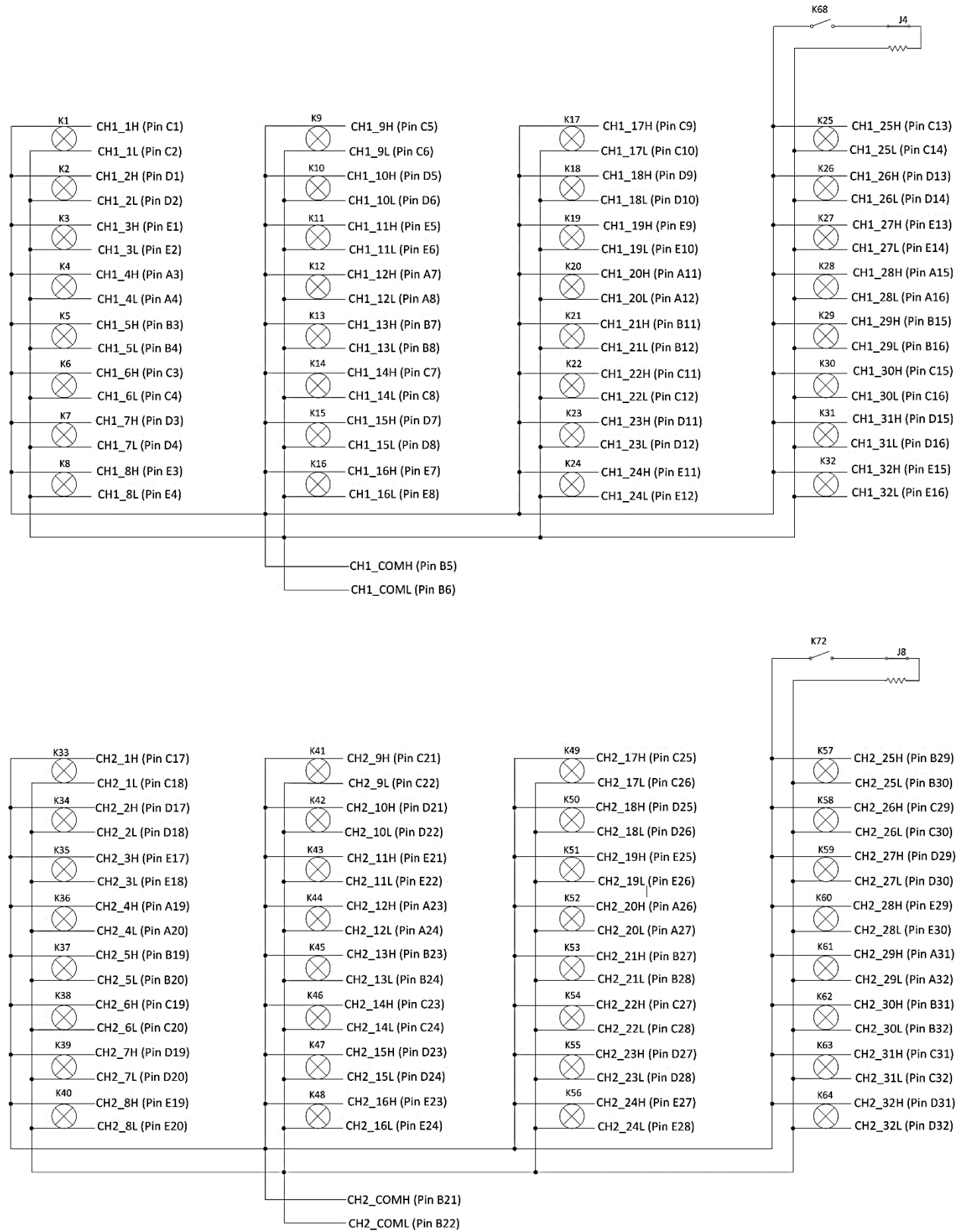
FIGURE 3-32: SMX-3004DS LOGICAL DIAGRAM
