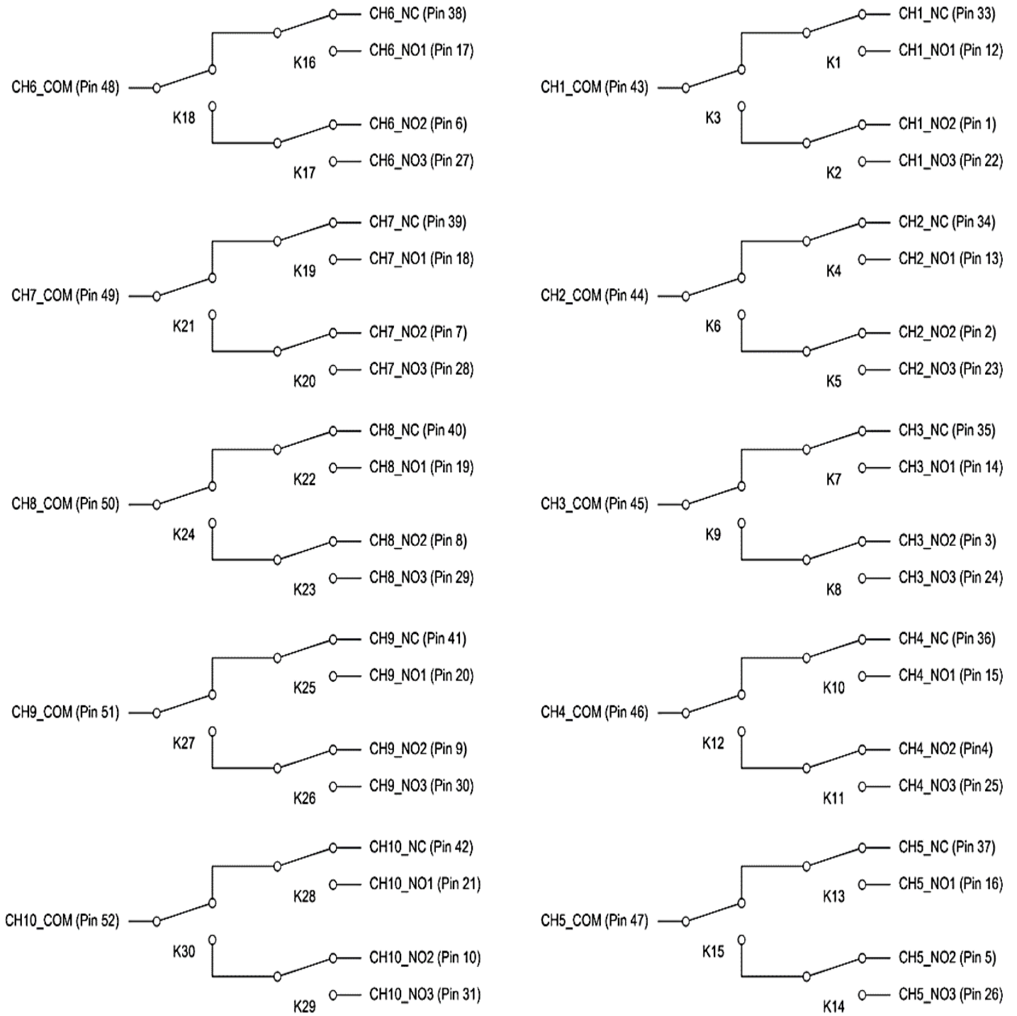
FIGURE 3-93: SMX-6101 PkZ LOGICAL DIAGRAM
