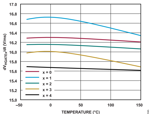
Figure 20. dV_{HGATE}/dt vs. Temperature
