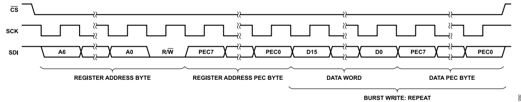
Figure 51. SPI Write
