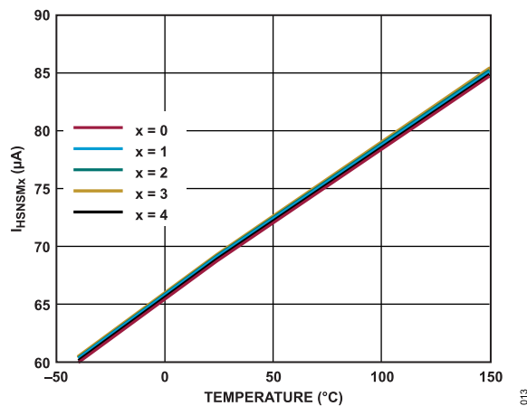
Figure 13. I_{HSNSMx} vs. Temperature, Port in Power-On State
