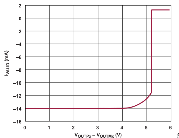
Figure 39. I_{INVALID} vs. V_{OUTPx} - V_{OUTMx}
