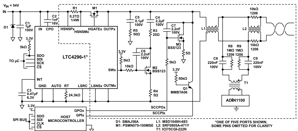
Figure 62. IEEE 802.3cq Class 14 PSE
