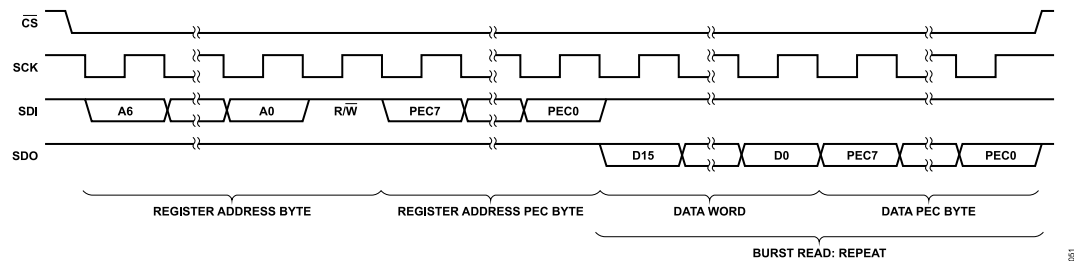
Figure 52. SPI Read
