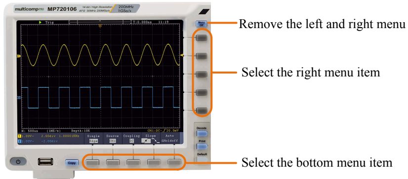
Figure 3-2 Menu Buttons
