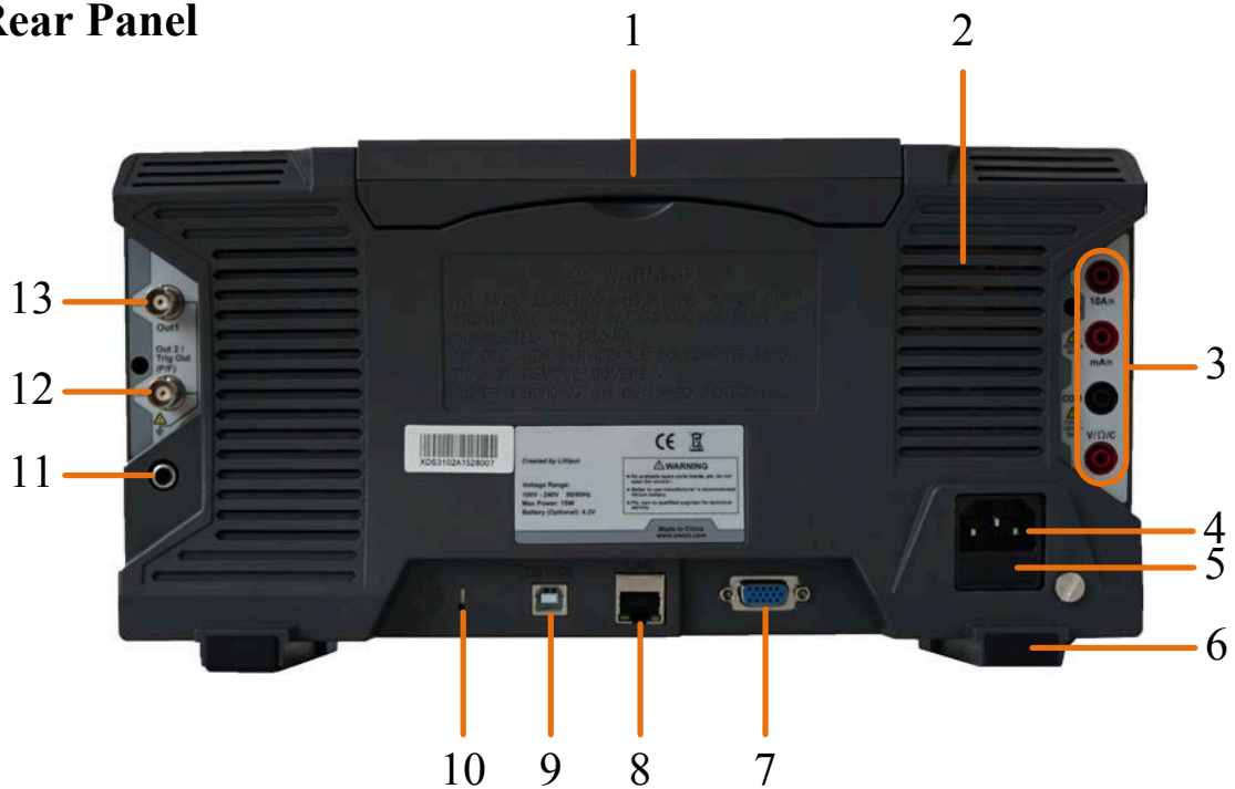
Figure 3-3 Rear Panel
