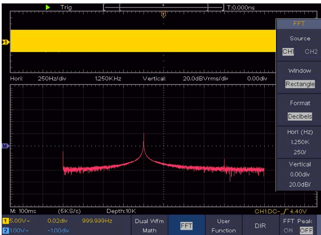
Figure 4-2 Rectangle window
