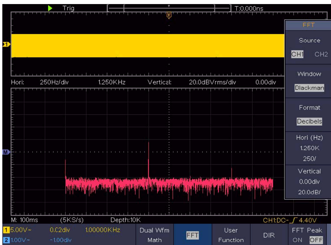
Figure 4-3 Blackman window
