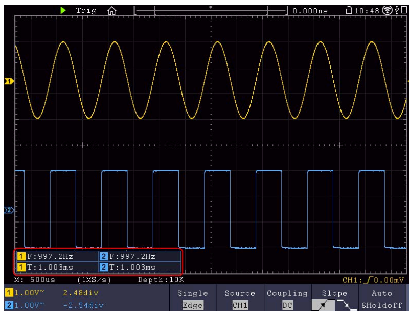
Figure 4-20 Automatic measurement
