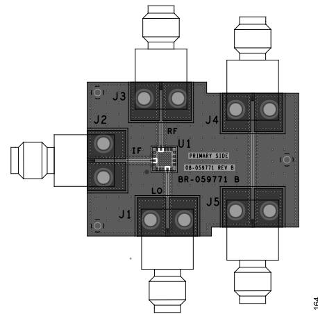
Figure 134. Evaluation PCB Top Layer
