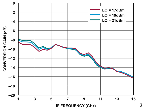
Figure 123. Conversion Gain vs. IF Frequency at Various LO Power Levels, T_A = 25^\circ\text{C}
