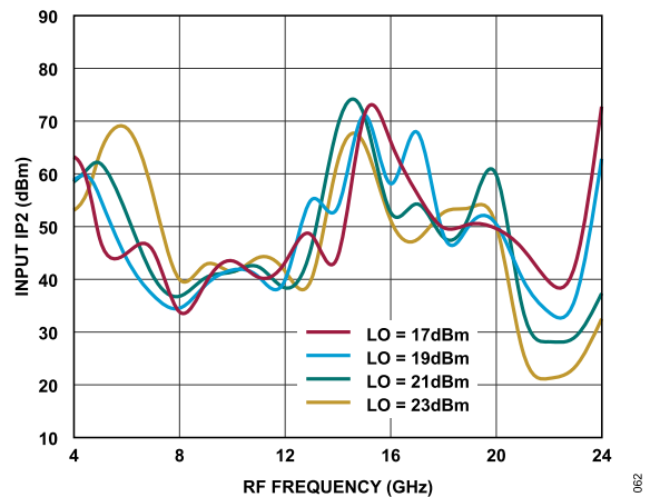
Figure 54. Input IP2 vs. RF Frequency at Various LO Power Levels, T_A = 25^\circ\text{C}
