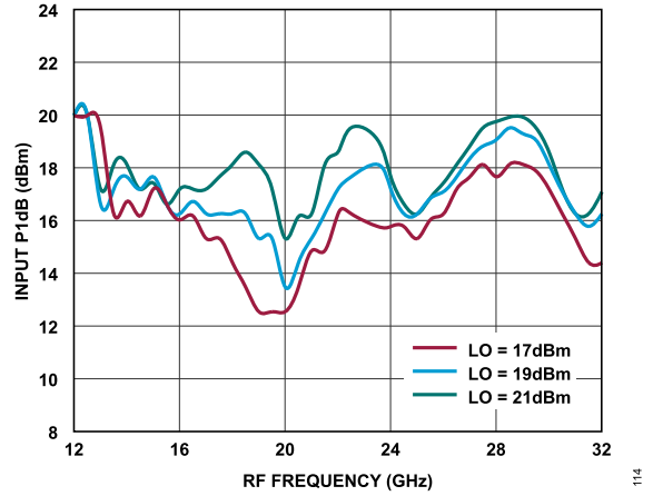
Figure 96. Input P1dB vs. RF Frequency at Various LO Power Levels, TA = 25°C
