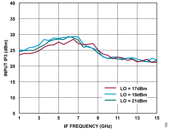
Figure 124. Input IP3 vs. IF Frequency at Various LO Power Levels, T_A = 25^\circ\text{C}
