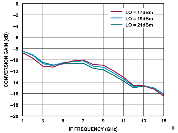
Figure 131. Conversion Gain vs. IF Frequency at Various LO Power Levels, TA = 25°C
