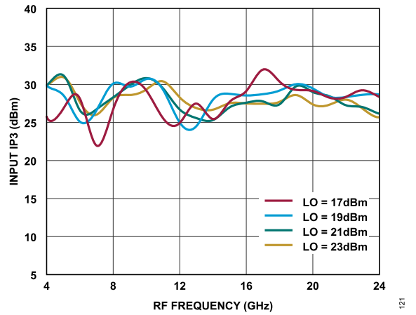
Figure 101. Input IP3 vs. RF Frequency at Various LO Power Levels, T_A = 25^\circ\text{C}
