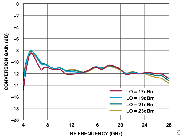
Figure 84. Conversion Gain vs. RF Frequency at Various LO Power Levels, TA = 25°C
