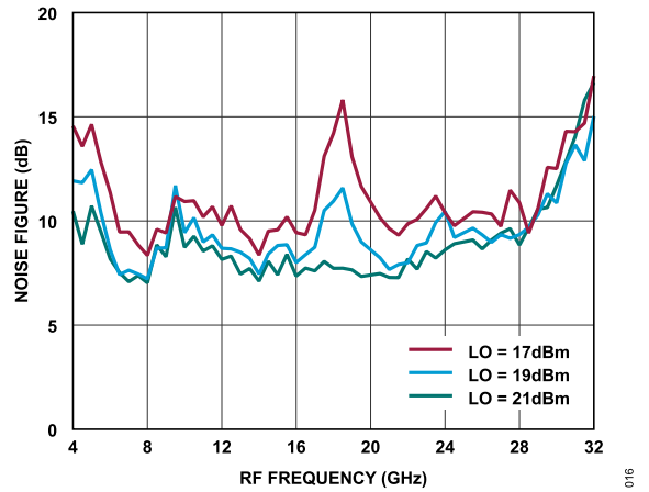
Figure 16. Noise Figure vs. RF Frequency at Various LO Power Levels, T_A = 25^\circ\text{C}
