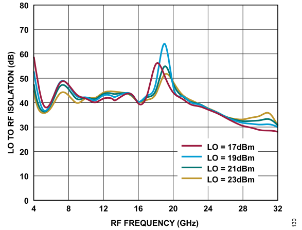
Figure 108. LO to RF Isolation vs. RF Frequency at Various LO Power Levels, TA = 25°C
