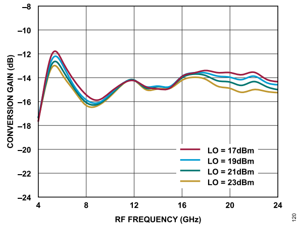
Figure 100. Conversion Gain vs. RF Frequency at Various LO Power Levels, T_A = 25^\circ\text{C}
