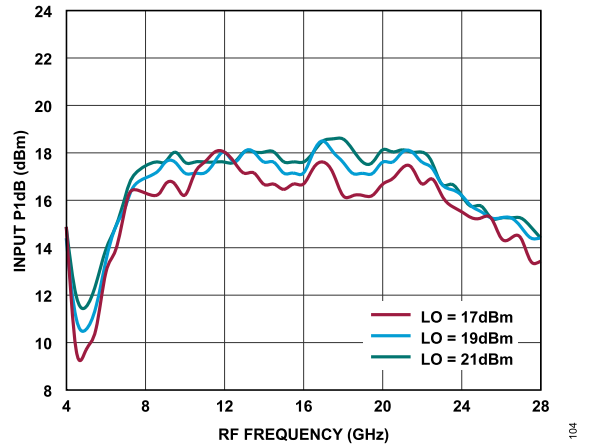
Figure 88. Input P1dB vs. RF Frequency at Various LO Power Levels, T_A = 25^\circ\text{C}
