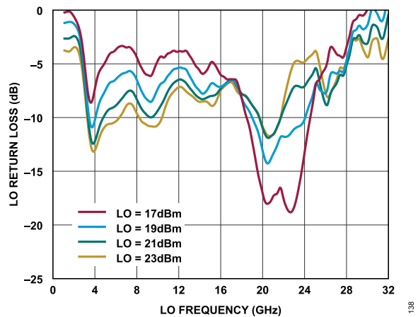
Figure 116. LO Return Loss vs. LO Frequency at Various LO Power Levels, TA = 25°C
