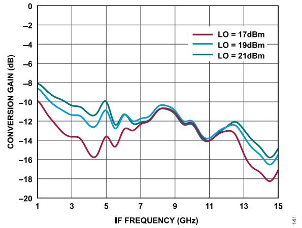
Figure 119. Conversion Gain vs. IF Frequency at Various LO Power Levels, T_A = 25^\circ\text{C}
