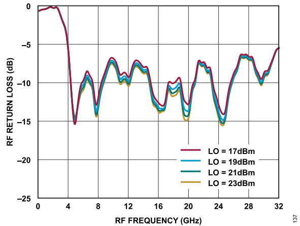
Figure 115. RF Return Loss vs. RF Frequency at Various LO Power Levels, TA = 25°C, LO = 20 GHz
