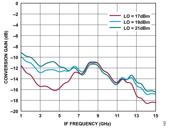
Figure 127. Conversion Gain vs. IF Frequency at Various LO Power Levels, T_A = 25^\circ\text{C}
