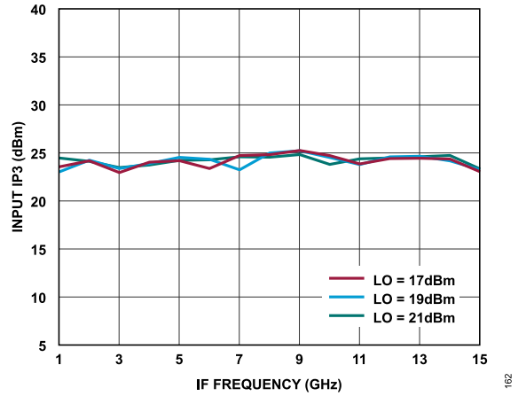
Figure 132. Input IP3 vs. IF Frequency at Various LO Power Levels, TA = 25°C
