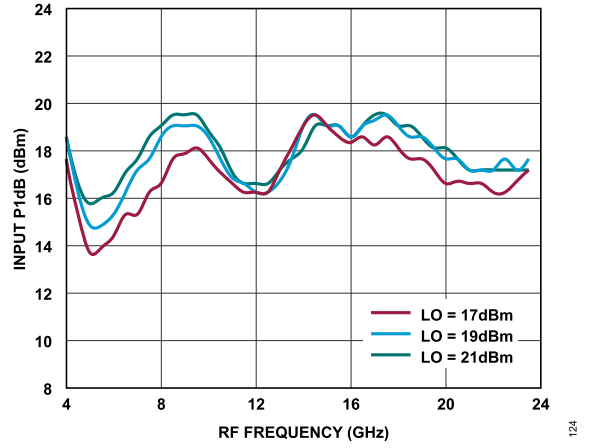
Figure 104. Input P1dB vs. RF Frequency at Various LO Power Levels, TA = 25°C
