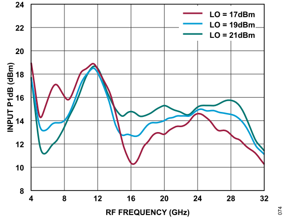
Figure 64. Input P1dB vs. RF Frequency at Various LO Power Levels, TA = 25°C
