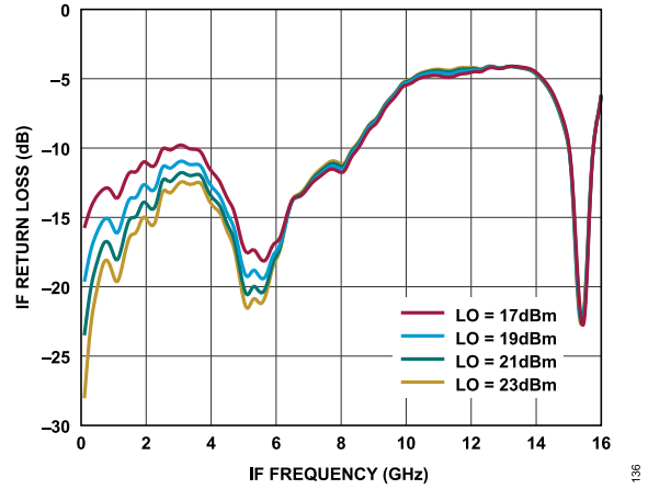
Figure 114. IF Return Loss vs. IF Frequency at Various LO Power Levels, TA = 25°C, LO = 20 GHz
