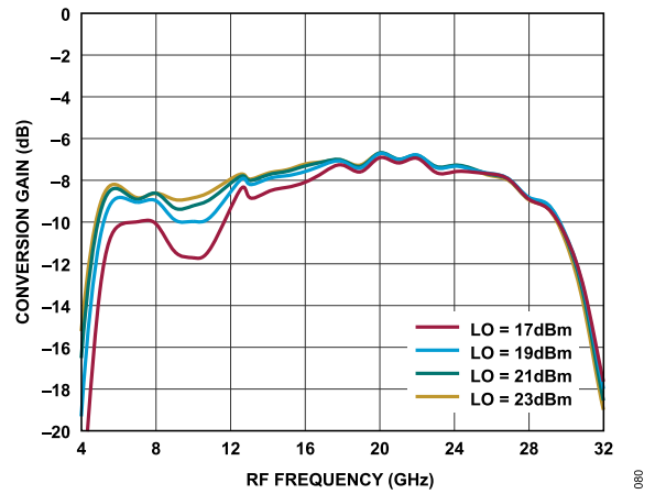
Figure 68. Conversion Gain vs. RF Frequency at Various LO Power Levels, T_A = 25^\circ\text{C}
