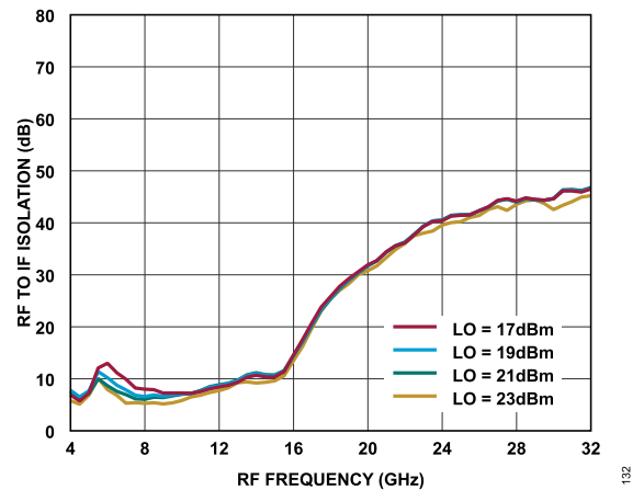
Figure 110. RF to IF Isolation vs. RF Frequency at Various LO Power Levels, TA = 25°C
