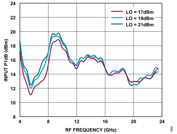
Figure 56. Input P1dB vs. RF Frequency at Various LO Power Levels, TA = 25°C
