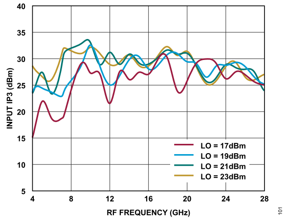
Figure 85. Input IP3 vs. RF Frequency at Various LO Power Levels, TA = 25°C
