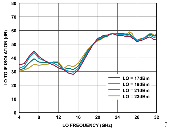
Figure 109. LO to IF Isolation vs. LO Frequency at Various LO Power Levels, TA = 25°C
