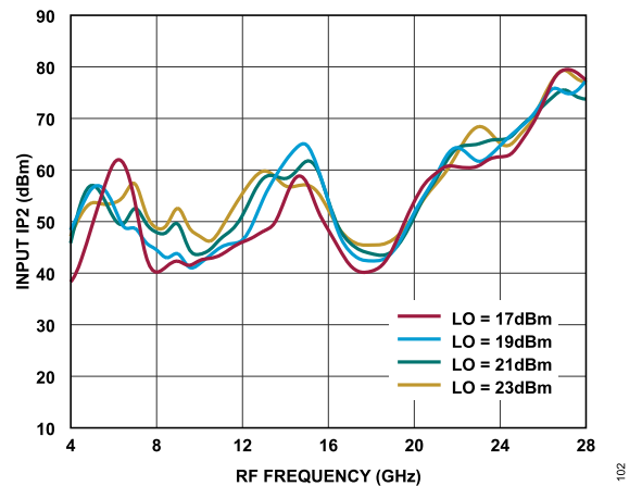
Figure 86. Input IP2 vs. RF Frequency at Various LO Power Levels, TA = 25°C
