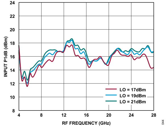
Figure 40. Input P1dB vs. RF Frequency at Various LO Power Levels, T_A = 25^\circ\text{C}
