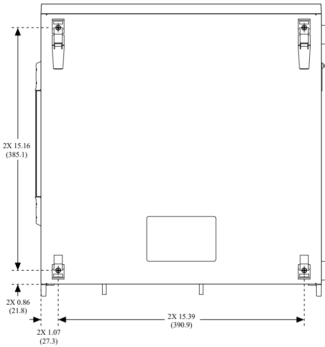
Figure 1. PXIe-1095 Chassis Dimensions (Bottom)
