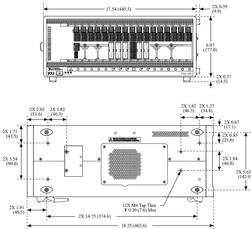
Figure 1. PXIe-1095 Chassis Dimensions (Front and Side)
