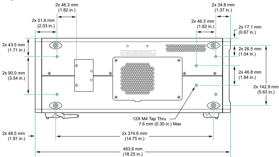
Figure 2. PXle-1092 Chassis Dimensions (side)
