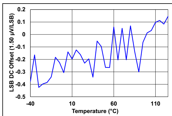
FIGURE 2-19: Input Offset for V_{SENSE} Measurements vs. Temperature.
