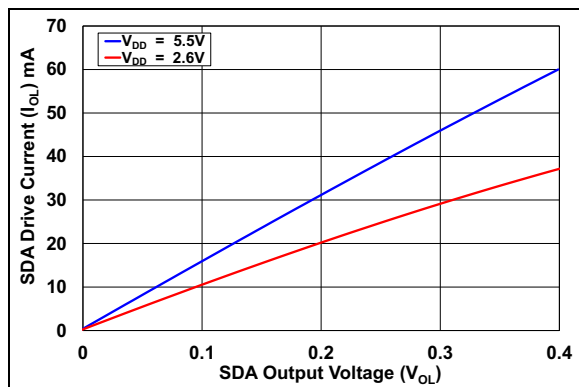
FIGURE 2-20: SDA Drive Current vs. V_{OL} at +25^{\circ}\text{C} .
