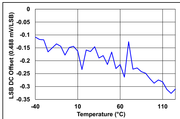
FIGURE 2-18: Input Offset for V_{BUS} Measurements vs. Temperature.
