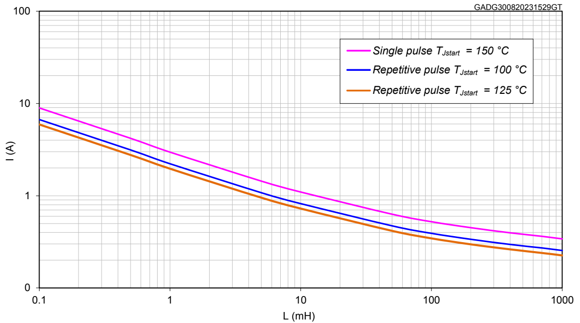
Figure 36. Maximum turn-off current versus inductance - Bulb mode all channels
