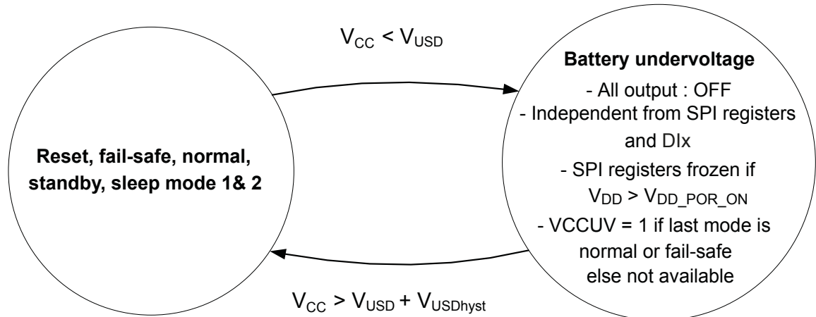
Figure 4. Battery undervoltage shutdown diagram
