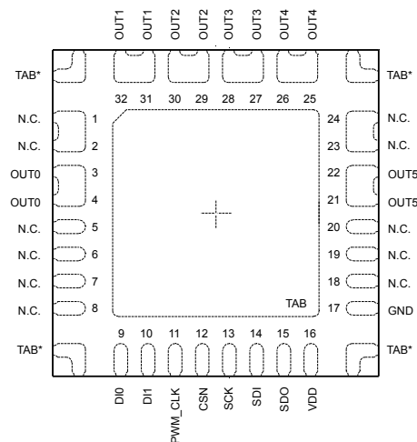
Figure 2. Connection diagram (top view)
