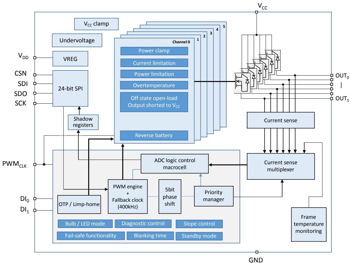
Figure 1. Block diagram
