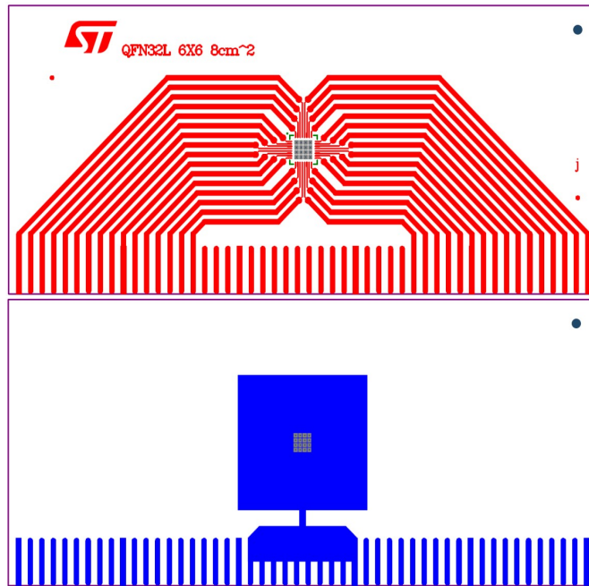
Figure 42. QFN 6x6 PCB 8 cm 2
