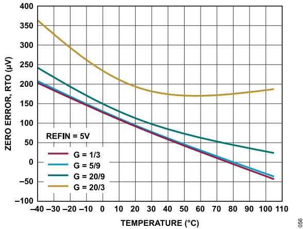
Figure 56. Zero Error vs. Temperature
