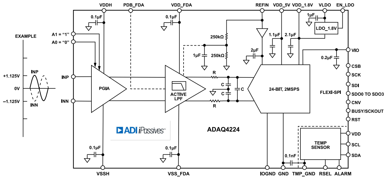
Figure 87. Differential Input Configuration with G = 20/9 \text{ V/V}
