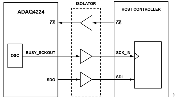
Figure 103. Host Clock Mode Signal Path Example
