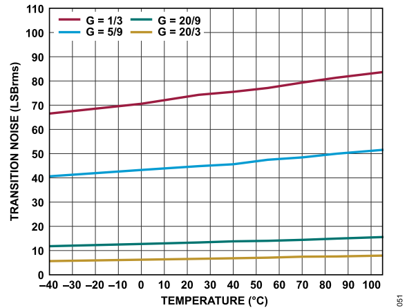
Figure 51. Transition Noise vs. Temperature, REFIN = 5 V
