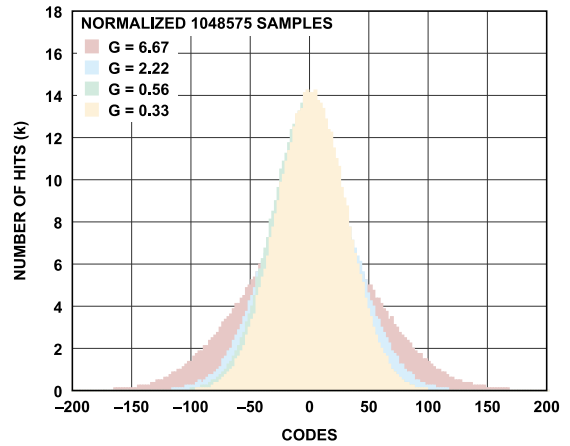
Figure 23. Code Histogram for Shorted Inputs, REFIN = 4.096 V
