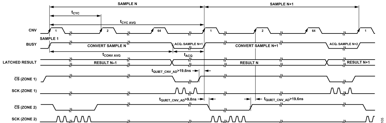
Figure 106. Example of Different Zones in Averaging Mode (64 Samples Averaged)
