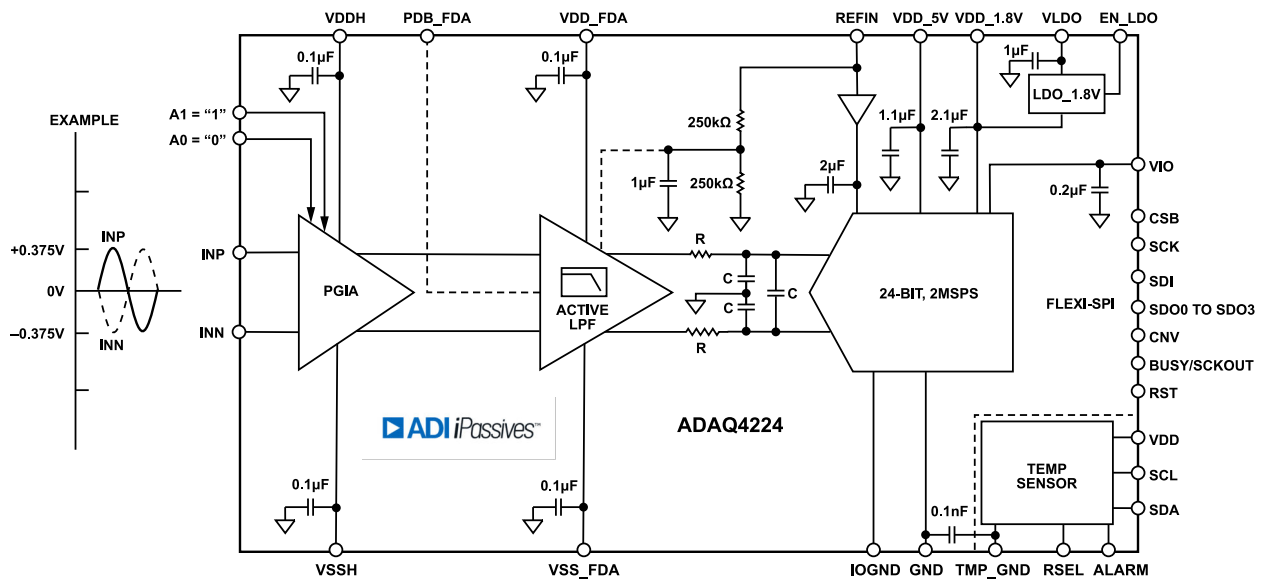
Figure 88. Differential Input Configuration with G = 20/3 \text{ V/V}
