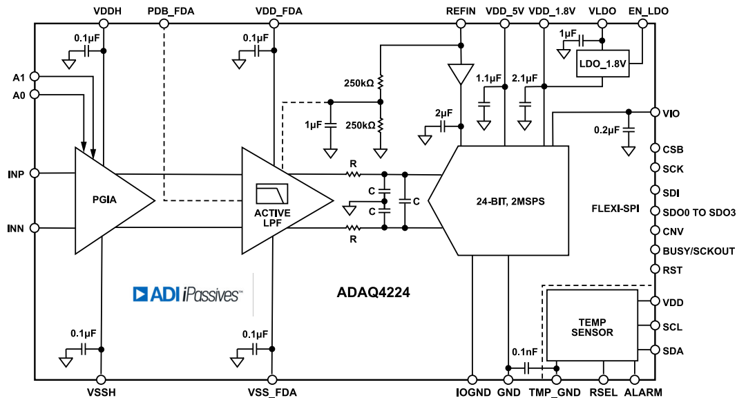
Figure 80. ADAQ4224 Functional Block Diagram
