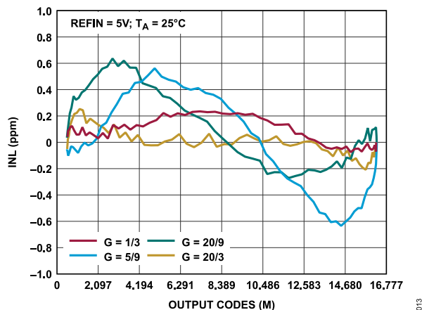
Figure 13. INL Error vs. Output Code, Differential Input, REFIN = 5 V
