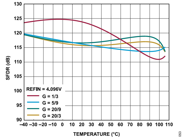
Figure 53. SFDR vs. Temperature, f_{IN} = 1 kHz, REFIN = 4.096 V
