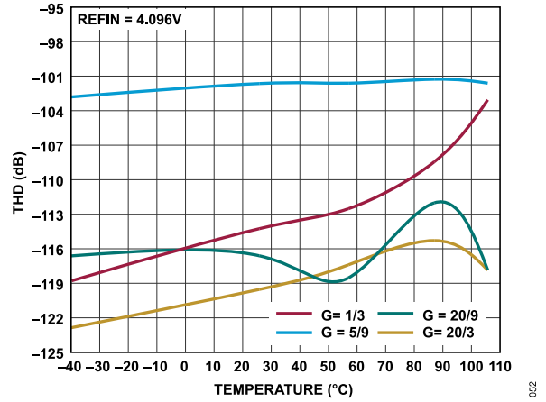
Figure 52. THD vs. Temperature, f_{IN} = 1 kHz Single-Ended Input, REFIN = 4.096 V
