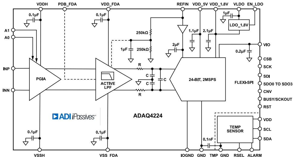
Figure 1. ADAQ4224 Functional Block Diagram
