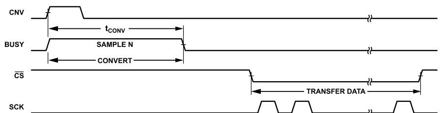
Figure 101. Typical Sample Cycle for SPI Clocking Mode
