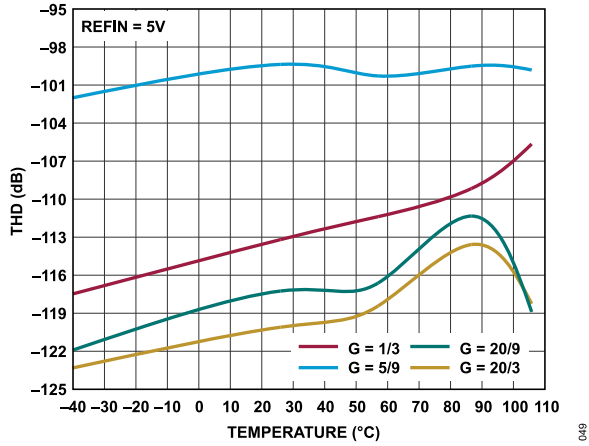
Figure 49. THD vs. Temperature, f_{IN} = 1 kHz Single-Ended Input, REFIN = 5 V
