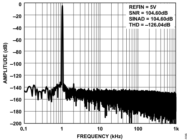
Figure 26. FFT, 2 MSPS, f_{IN} = 1 kHz, Differential Input = -0.5 dBFS, G = 20/9
