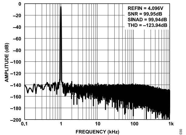
Figure 30. FFT, 2 MSPS, f_{IN} = 1 kHz, Differential Input = -0.5 dBFS, G = 20/3
