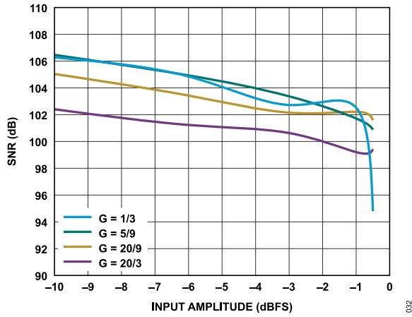
Figure 32. SNR vs. Input Amplitude at f_{IN} = 20 kHz
