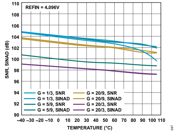
Figure 47. SNR, SINAD vs. Temperature, f_{IN} = 1 kHz Single-Ended Input, REFIN = 4.096 V
