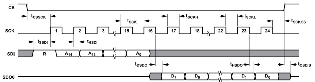
Figure 4. Register Configuration Mode Read Timing
