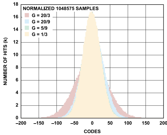
Figure 20. Code Histogram for Shorted Inputs, REFIN = 5 V
