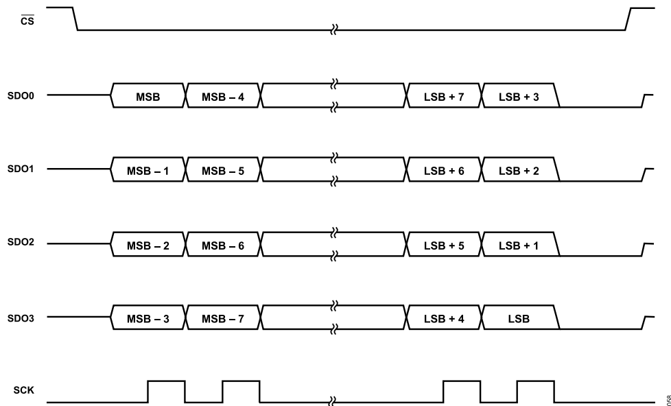
Figure 110. 4-Lane, SDR Timing Diagram
