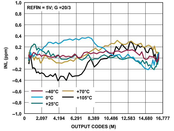
Figure 22. INL Error vs. Output Code across Temperature, G = 20/3
