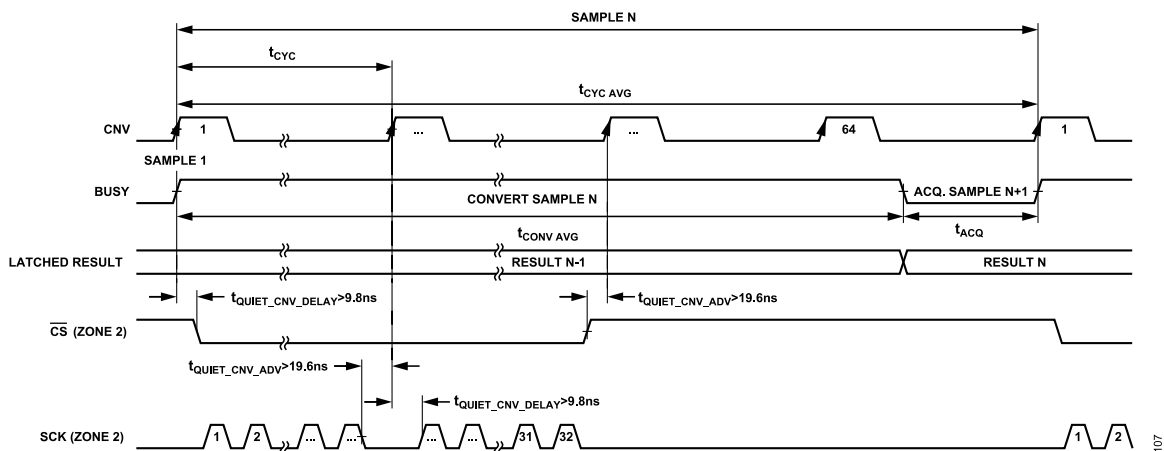
Figure 108. Example of Zone 2 in Averaging Mode (N Bits per Cycle)
