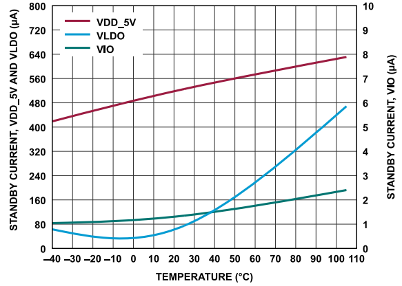
Figure 76. Standby Current ADC vs. Temperature
