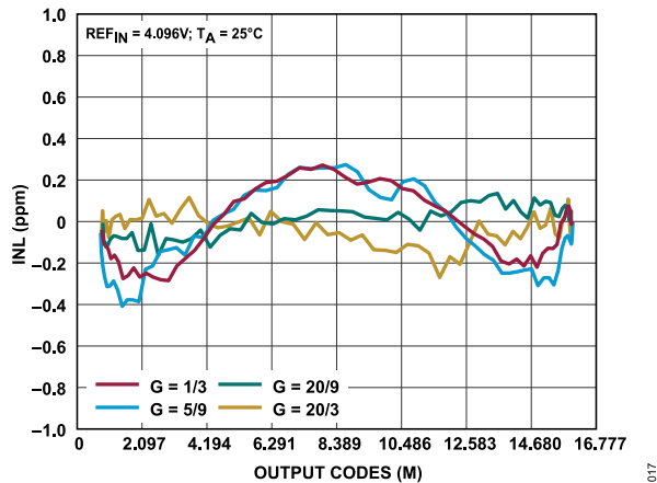
Figure 17. INL Error vs. Output Code, Single-Ended Input, REFIN = 4.096 V
