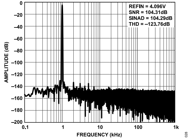
Figure 28. FFT, 2 MSPS, f_{IN} = 1 kHz, Differential Input = -0.5 dBFS, G = 5/9
