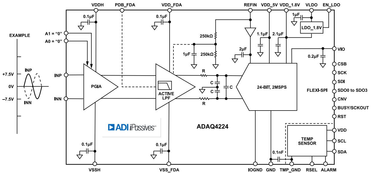
Figure 85. Differential Input Configuration with G = 1/3 \text{ V/V}
