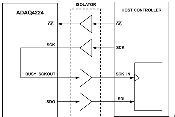
Figure 102. Echo Clock Mode Signal Path Diagram
