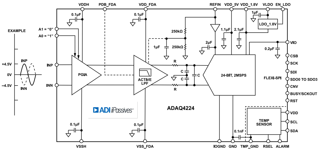
Figure 86. Differential Input Configuration with G = 5/9 \text{ V/V}
