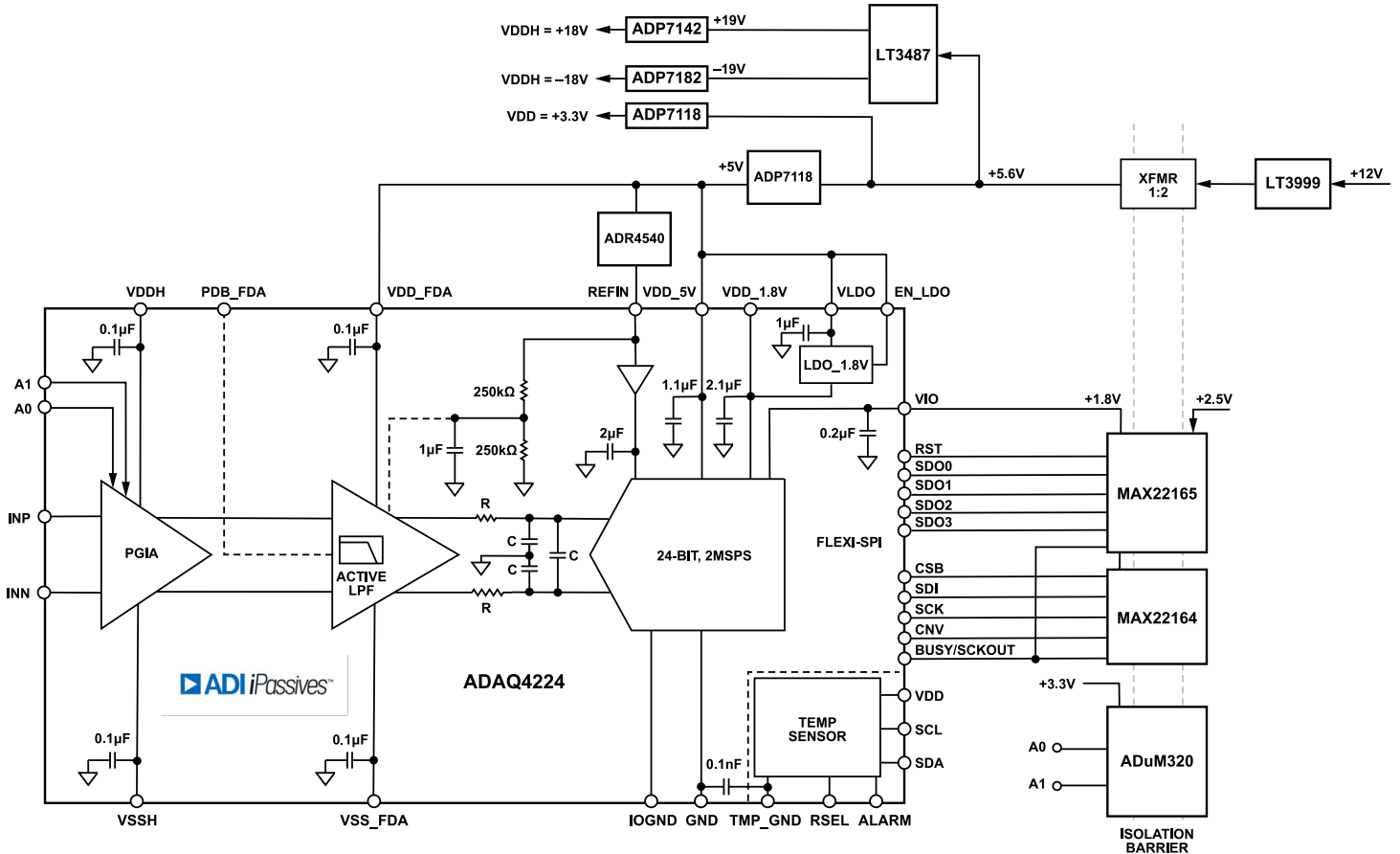
Figure 84. Functional Block Diagram of a Fully Isolated Data-Acquisition System
