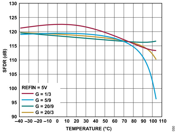
Figure 50. SFDR vs. Temperature, f_{IN} = 1 kHz, REFIN = 5 V
