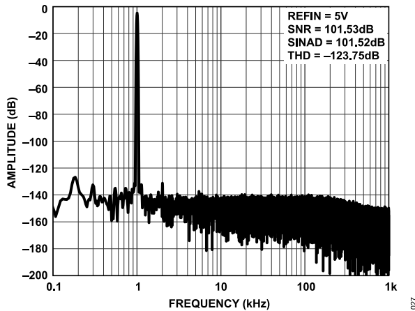
Figure 27. FFT, 2 MSPS, f_{IN} = 1 kHz, Differential Input = -0.5 dBFS, G = 20/3
