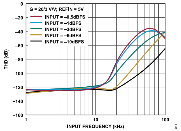
Figure 41. THD vs. Input Frequency, Various Amplitudes, G = 20/3
