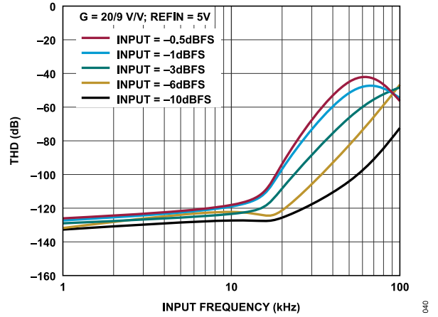
Figure 40. THD vs. Input Frequency, Various Amplitudes, G = 20/9
