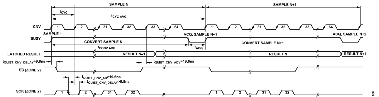
Figure 107. Example of Zone 2 in Averaging Mode (1 Bit per Sample)
