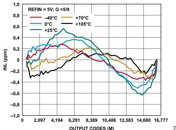
Figure 18. INL Error vs. Output Code across Temperature, G = 5/9
