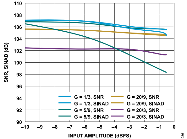
Figure 36. SNR, SINAD vs. Input Amplitude at f_{IN} = 1 kHz Single-Ended
