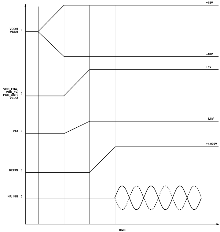
Figure 96. Power Supply Sequence
