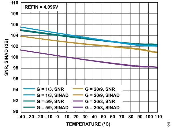
Figure 46. SNR, SINAD vs. Temperature, f_{IN} = 1 kHz Differential Input, REFIN = 4.096 V
