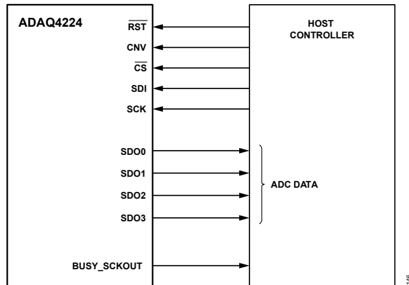
Figure 98. ADAQ4224 Multilane SPI
