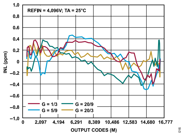
Figure 16. INL Error vs. Output Code, Differential Input, REFIN = 4.096 V
