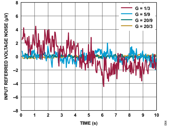
Figure 64. Low Frequency Noise (Output Data Rate = 19.5 SPS After Averaging Blocks of 2048 Samples), REFIN = 4.096 V
