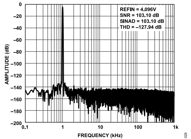
Figure 29. FFT, 2 MSPS, f_{IN} = 1 kHz, Differential Input = -0.5 dBFS, G = 20/9
