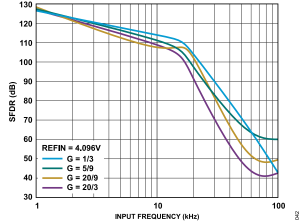
Figure 42. SFDR vs. Input Frequency, -0.5 dBFS, REFIN = 4.096 V
