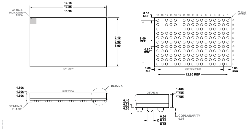
Figure 111. 178-Ball Chip-Scale Package, Ball Grid Array [CSP_BGA] (BC-178-2) Dimensions Shown in millimeters
