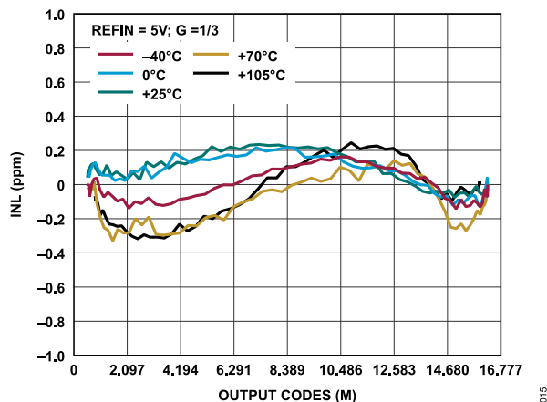
Figure 15. INL Error vs. Output Code across Temperature, G = 1/3
