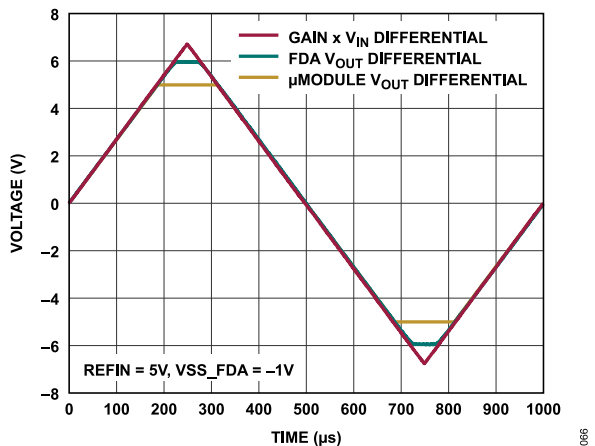
Figure 66. Output Overdrive Recovery, IN = 1 kHz
