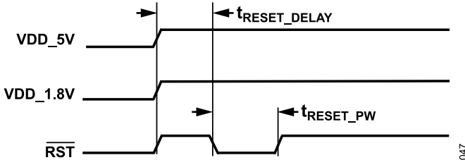
Figure 95. Power-On Reset (POR) Timing
