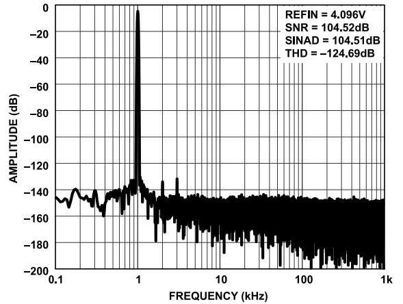
Figure 24. FFT, 2 MSPS, f_{IN} = 1 kHz, Differential Input = -0.5 dBFS, G = 1/3
