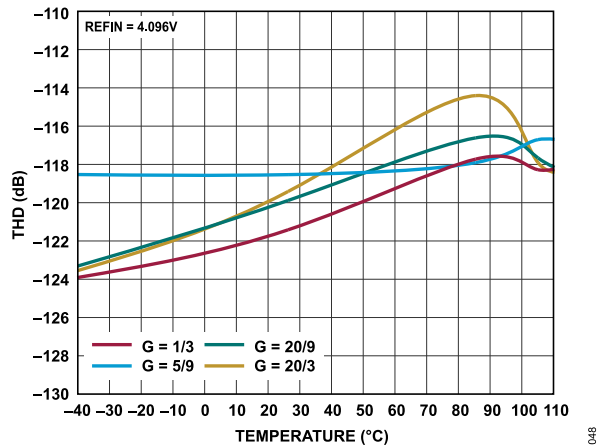
Figure 48. THD vs. Temperature, f_{IN} = 1 kHz Differential Input, REFIN = 4.096 V
