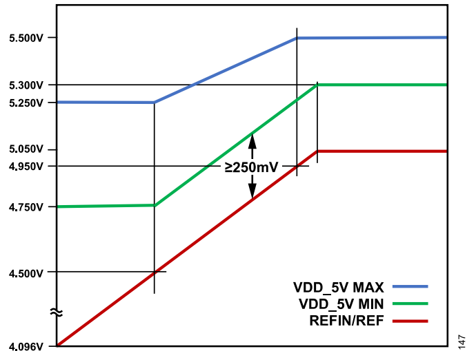
Figure 97. VDD_5V Minimum and Maximum Values for REFIN
