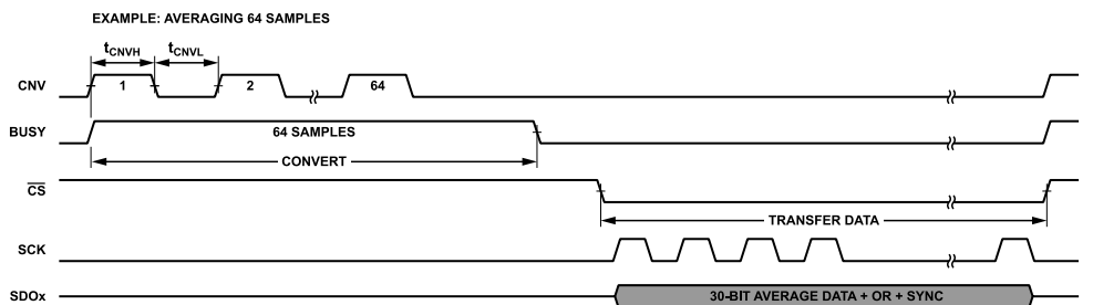
Figure 105. Example Conversion Cycle for Averaging Mode
