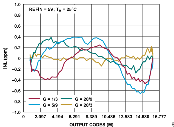
Figure 14. INL Error vs. Output Code, Single-Ended Input, REFIN = 5 V
