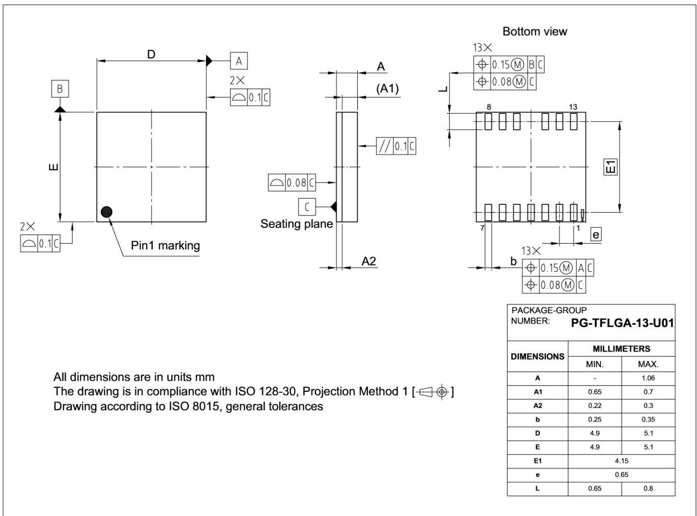
Figure 21 LGA 5x5 package outline
