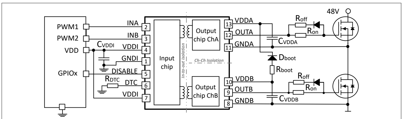
Figure 1 Application diagram
