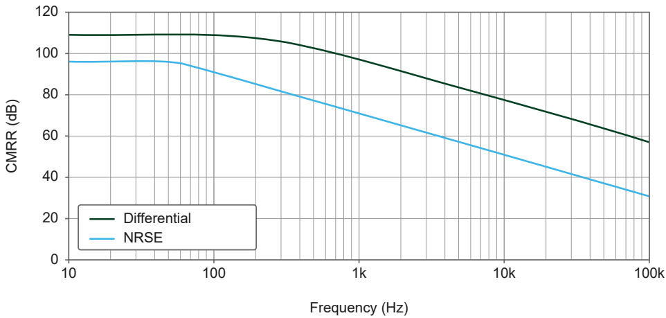
Figure 6. USB-6421 CMRR versus Frequency
