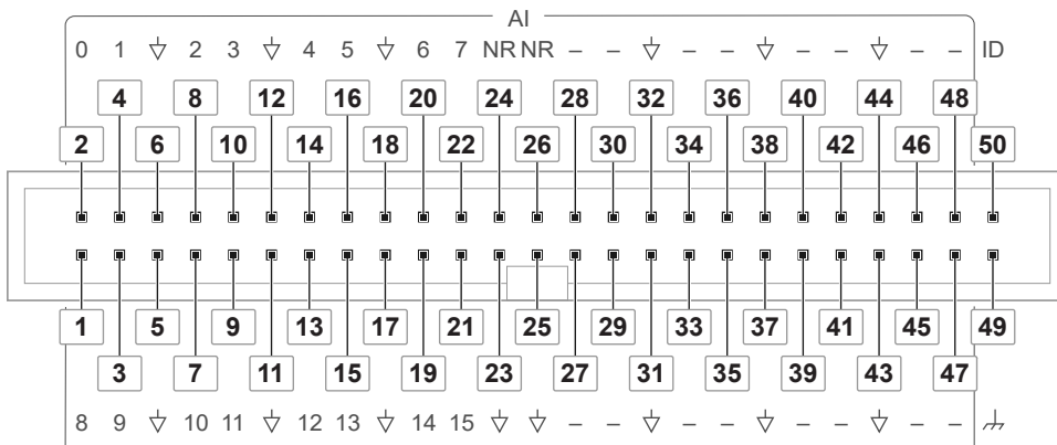
Figure 4. USB-6421 (OEM) AI Connector Pinout
