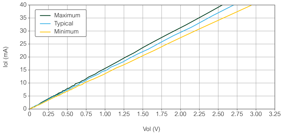
Figure 9. I_{OL} versus V_{OL} , 5.0 V Logic Family
