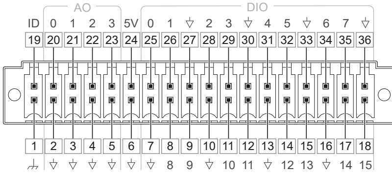
Figure 4. USB-6423 AO/DIO Connector Pinout
