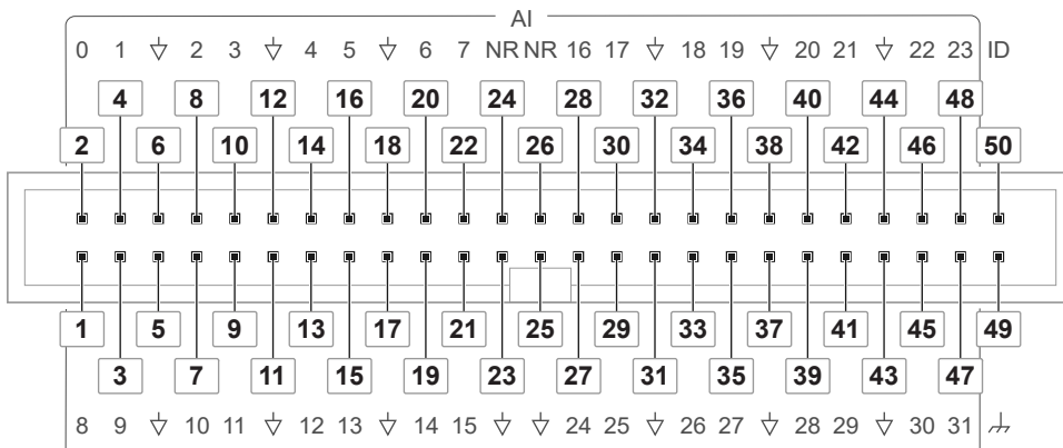
Figure 4. USB-6423 (OEM) AI Connector Pinout
