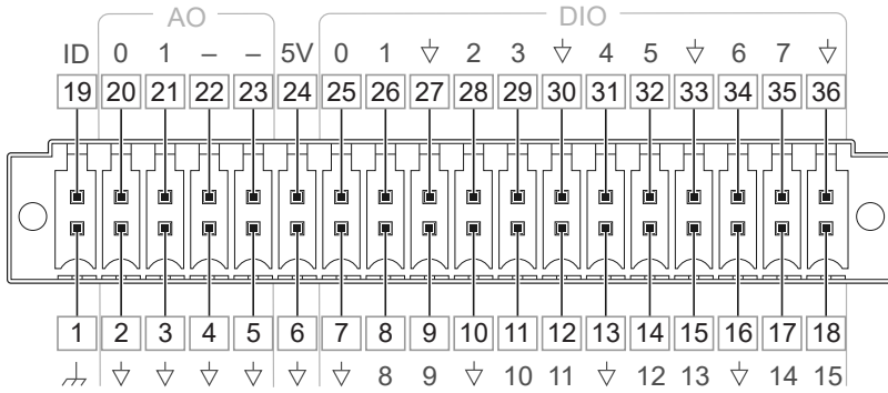
Figure 4. USB-6451 AO/DIO Connector Pinout
