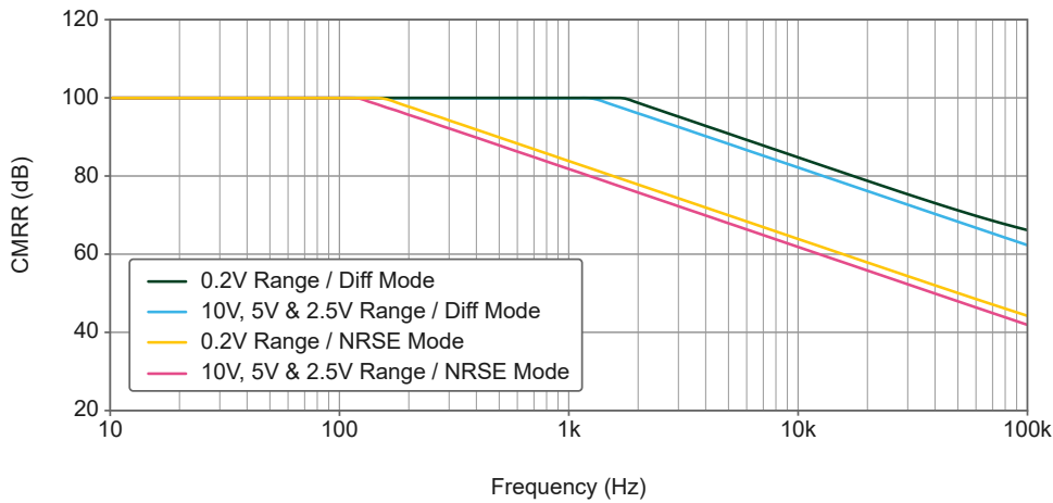
Figure 8. USB-6451 (OEM) CMRR versus Frequency
