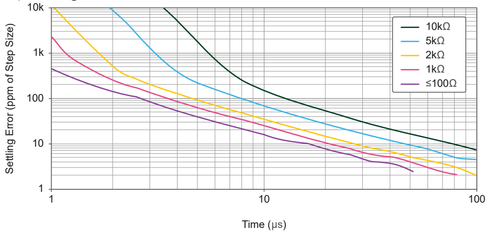
Figure 10. USB-6451 Settling Error versus Time for Different Source Impedances at the 0.2 V Input Range
