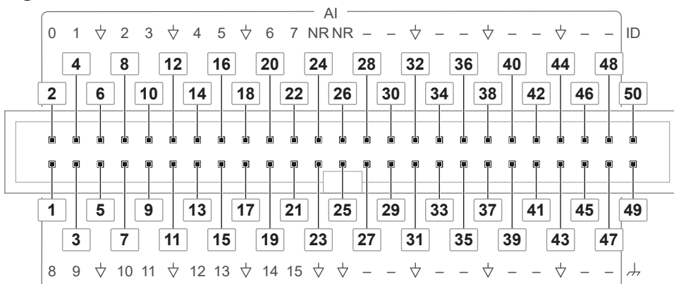
Figure 4. USB-6451 (OEM) AI Connector Pinout
