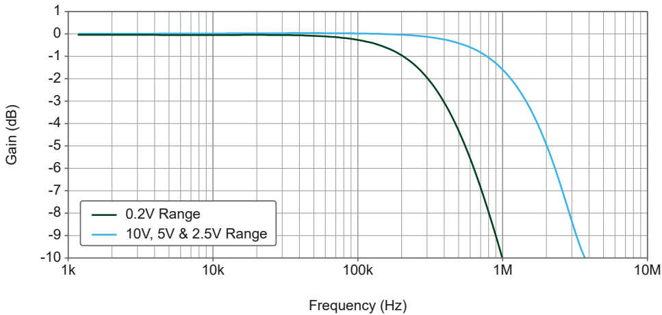
Figure 6. USB-6451 (OEM) Small Signal Bandwidth versus Frequency
