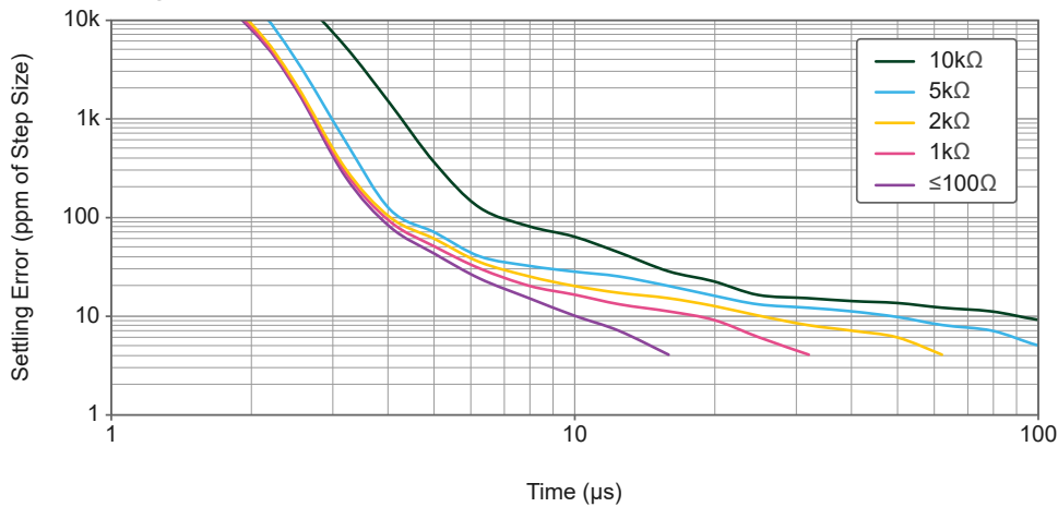
Figure 11. USB-6451 (OEM) Settling Error versus Time for Different Source Impedances at the 0.2 V Input Range
