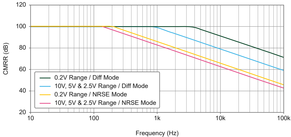
Figure 8. USB-6451 (OEM) CMRR versus Frequency
