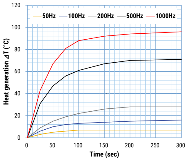
Figure 6 - Heat Generation vs. Drive Frequency - 1 Model: AL0505D16KF Input voltage: 150Vp-p, 75VDC bias
