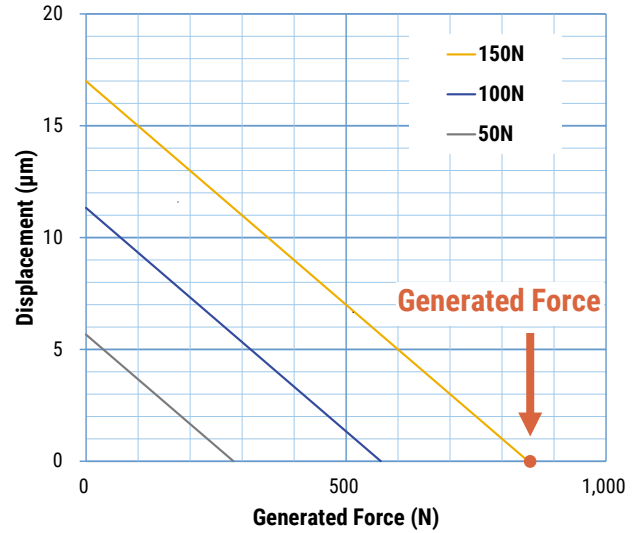
Figure 2 - Generated Force vs. Displacement of AL0505D18KF in Driving Voltage
