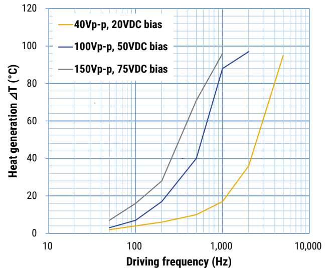
Figure 7 - Heat Generation vs. Drive Frequency - 2 Model: AL0505D16KF Temperature measurement: 5 minutes later from operation
