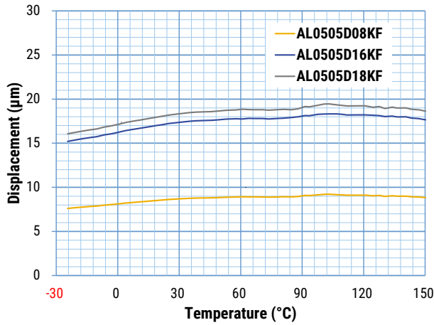
Figure 4 - Temperature vs. Displacement
