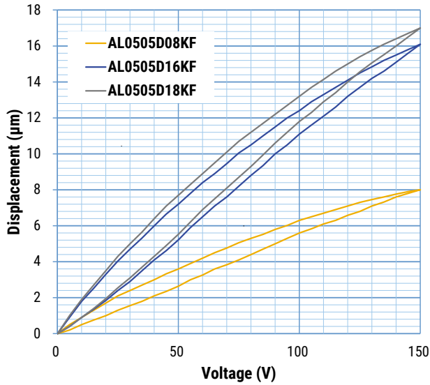
Figure 1 - Voltage vs. Displacement
