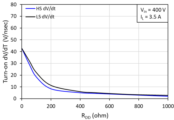
Fig. 19. Slew rate ( dV/dt ) vs. gate drive turn-on current set resistance ( R_{DDL} ) at T = 25\text{ °C}
