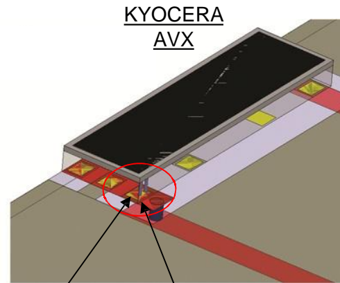
KYOCERA AVX Shorting pin and feed pin are shared in KYOCERA AVX ceramic antennas Figure 2 KYOCERA AVX Antenna Layout (Required)
