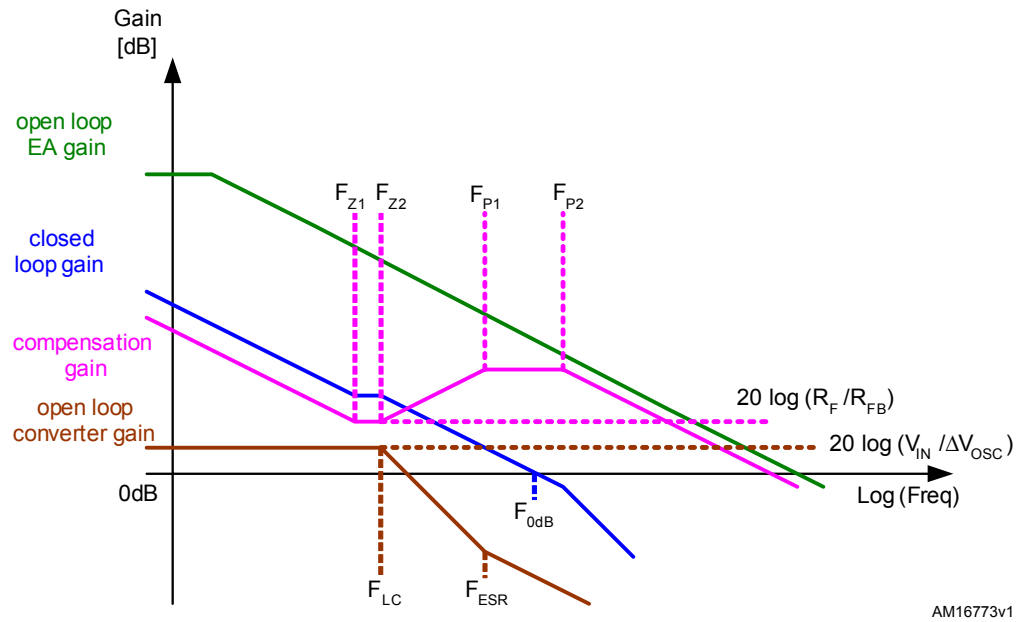
Figure 9. Example of type III compensation.
