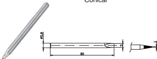
MP740164 Chisel
