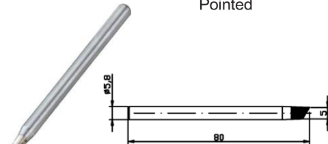
MP740165 Conical
