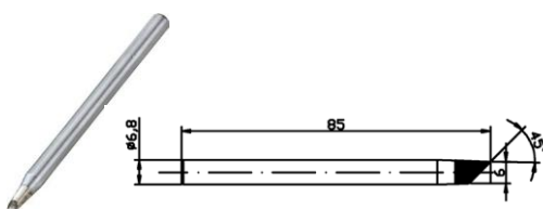
MP740168 Conical
