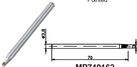
MP740162 Conical
