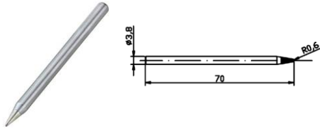
MP740160 Pointed
