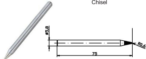
MP740163 Pointed
