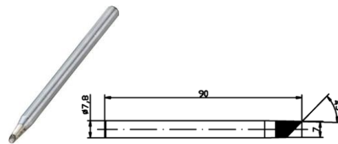
MP740171 Conical
