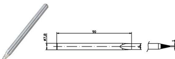
MP740170 Chisel
