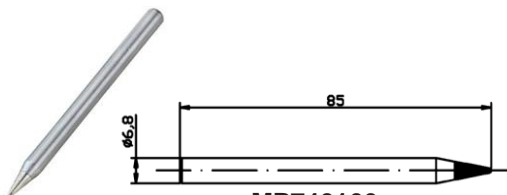
MP740166 Pointed
