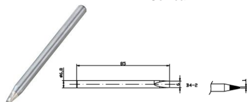
MP740167 Chisel
