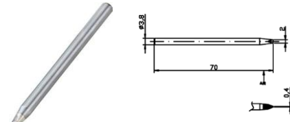
MP740161 Chisel
