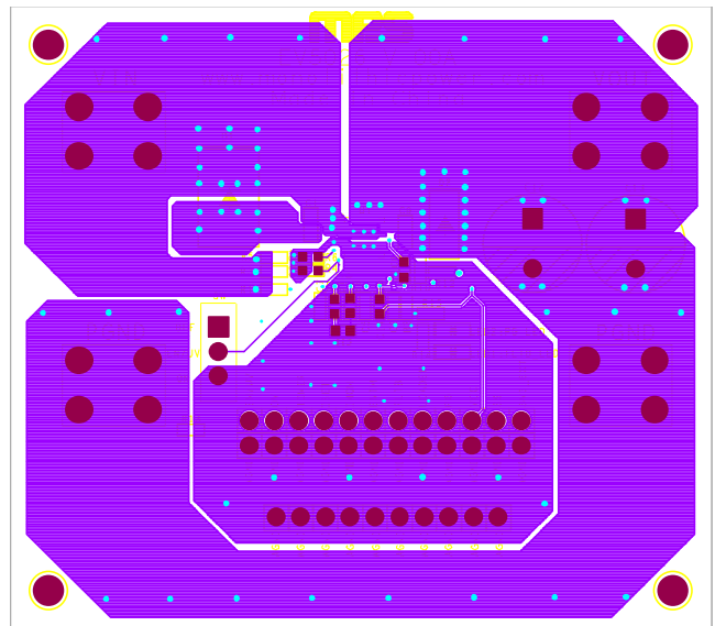
Figure 6: Bottom Layer
