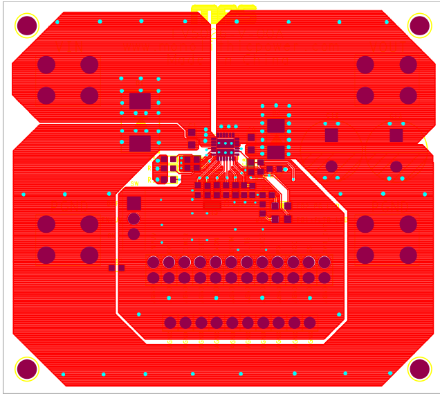
Figure 3: Top Layer
