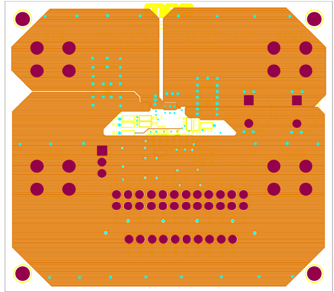
Figure 4: Mid-Layer 1
