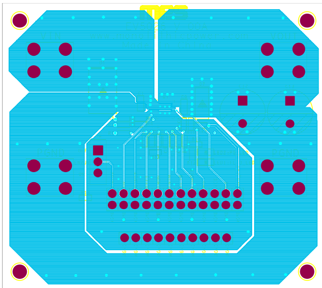
Figure 5: Mid-Layer 2
