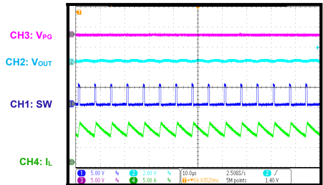
Short-Circuit Protection
