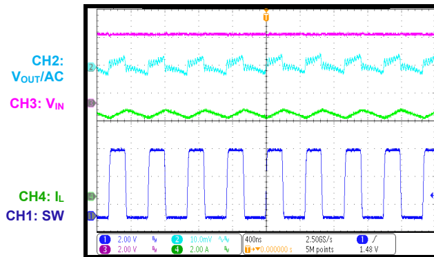
Steady State I_{OUT} = 6A
