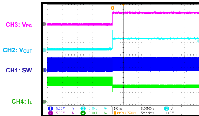
SCP Recovery I_{OUT} = 6A
