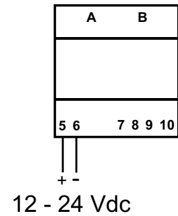
Fig. 12 Power supply
