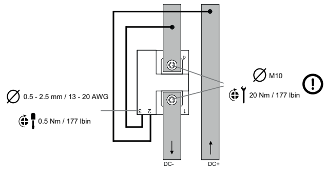
Fig. 9 Current (option B) and voltage inputs
