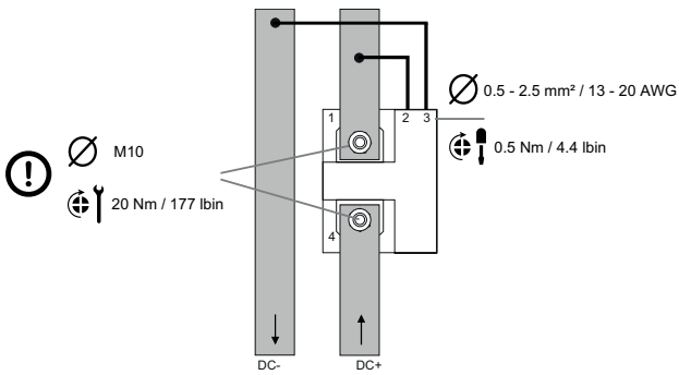
Fig. 8 Current (option A) and voltage inputs
