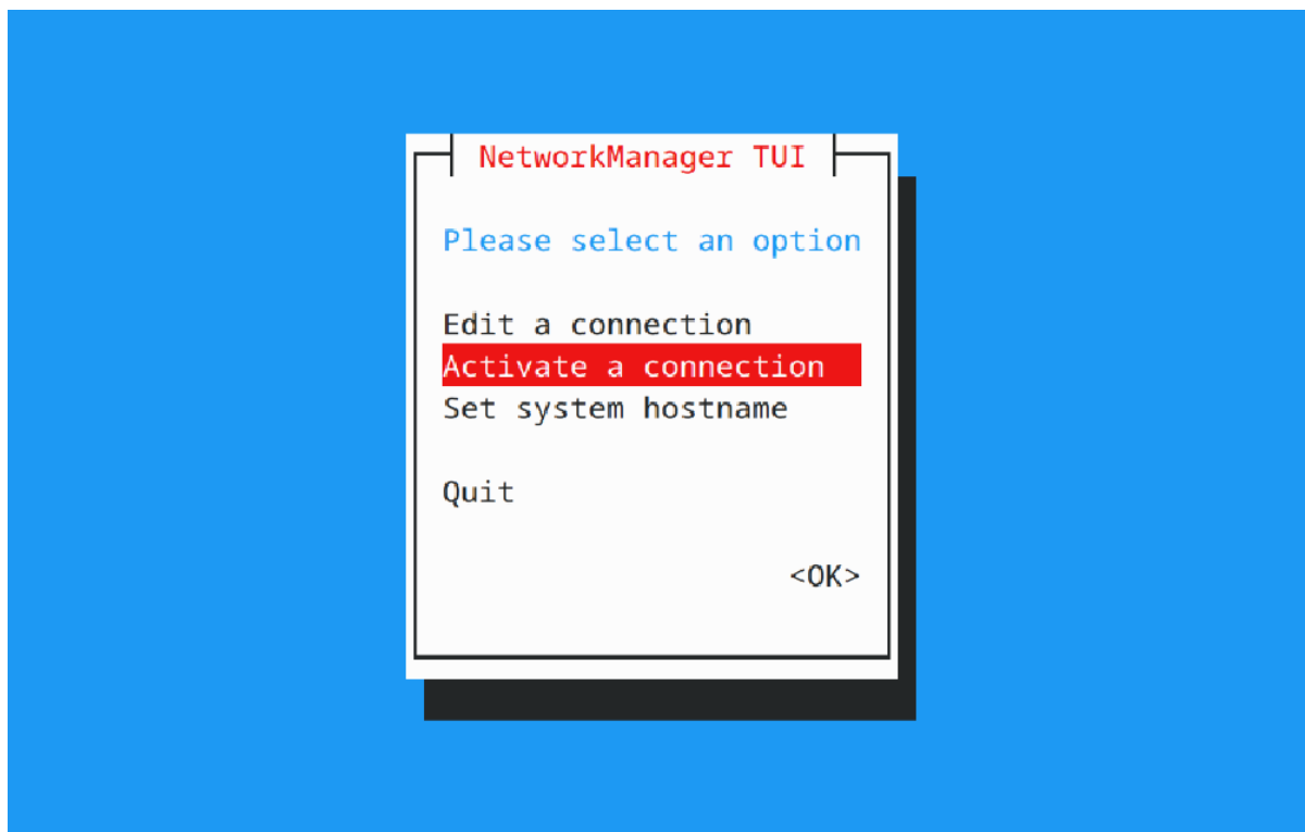
Fig. 2.33: NetworkManager TUI
