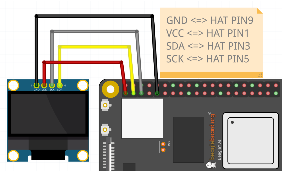
Fig. 5.16: OLED display 128x32
