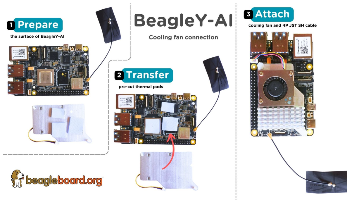
Fig. 2.34: Attaching cooling fan to BeagleY-AI
