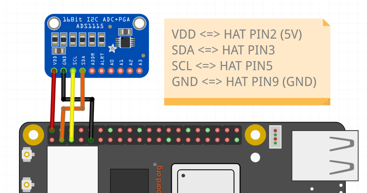
Fig. 5.26: ADS1115 connection
